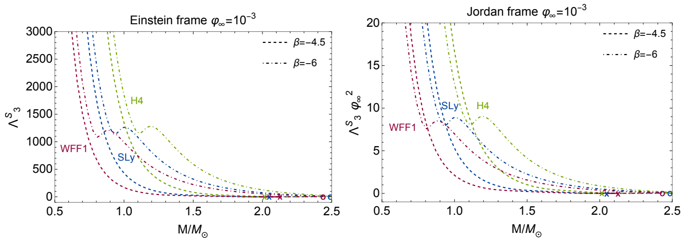
FIG. 24. Octupolar scalar dimensional tidal deformabilities \Lambda_3^S in the Einstein and Jordan frames for three equations of state (WFF1, SLy and H4). The Jordan frame plots use the Jordan frame mass. The dashed and dot-dashed lines are the scalarized configurations with \beta = -4.5 and \beta = -6 , respectively. The cross represents the maximum mass configuration for \beta = 0, -4.5 , and the circle for \beta = -6 . Both plots correspond to a scalar field at infinity \varphi_{0\infty} = 10^{-3} .
