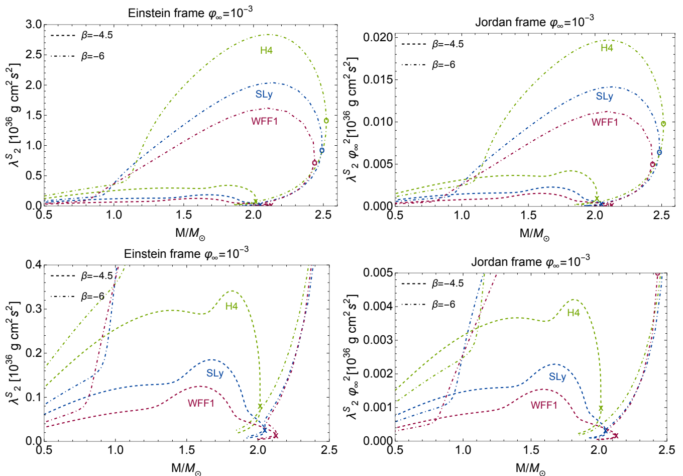
FIG. 11. Quadrupolar scalar tidal deformabilities \lambda_2^S in the Einstein and Jordan frames for three equations of state (WFF1, SLy and H4). The Jordan frame plots use the Jordan frame mass. The dashed and dot-dashed lines are the scalarized configurations with \beta = -4.5 and \beta = -6 , respectively, and the plots in the bottom panels are zoomed with respect to their counterparts in the top panels. The cross represents the maximum mass configuration for \beta = 0, -4.5 , and the circle for \beta = -6 . All plots correspond to a scalar field at infinity \varphi_{0\infty} = 10^{-3} .
