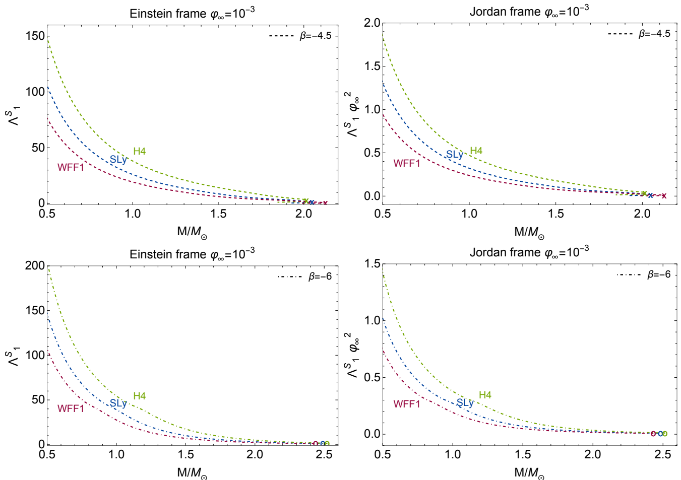
FIG. 15. Dipolar scalar adimensional tidal deformabilities \Lambda_1^S in the Einstein and Jordan frames for three equations of state (WFF1, SLy and H4). The Jordan frame plots use the Jordan frame mass. The dashed and dot-dashed lines are the scalarized configurations with \beta = -4.5 and \beta = -6 , respectively. The cross represents the maximum mass configuration for \beta = 0, -4.5 , and the circle for \beta = -6 . For \beta = -6 we have omitted the data beyond the maximum mass configuration for better readability. All plots correspond to a scalar field at infinity \varphi_{0\infty} = 10^{-3} .
