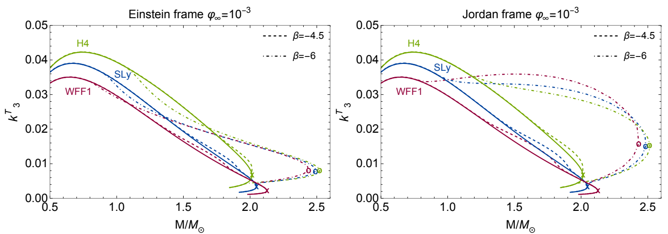
FIG. 26. Octupolar tensor Love numbers k_3^T in the Einstein and Jordan frames for three equations of state (WFF1, SLy and H4). The solid lines represent the GR configurations \beta = 0 and the dashed and dot-dashed lines are the scalarized configurations with \beta = -4.5 and \beta = -6 , respectively. The cross represents the maximum mass configuration for \beta = 0, -4.5 , and the circle for \beta = -6 . Both plots correspond to a scalar field at infinity \varphi_{0\infty} = 10^{-3} .
