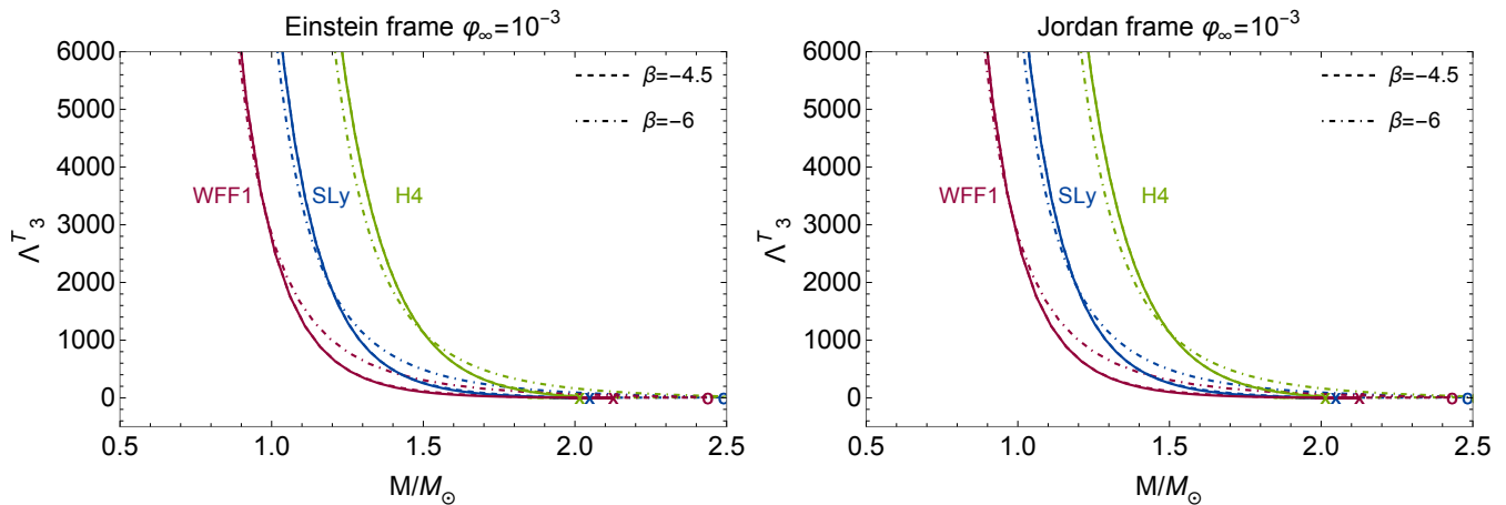
FIG. 23. Octupolar tensor adimensional tidal deformabilities \Lambda_3^T in the Einstein and Jordan frames for three equations of state (WFF1, SLy and H4). The Jordan frame plots use the Jordan frame mass. The solid lines represent the GR configurations \beta = 0 and the dashed and dot-dashed lines are the scalarized configurations with \beta = -4.5 and \beta = -6 , respectively. The cross represents the maximum mass configuration for \beta = 0, -4.5 , and the circle for \beta = -6 . Both plots correspond to a scalar field at infinity \varphi_{0\infty} = 10^{-3} .
