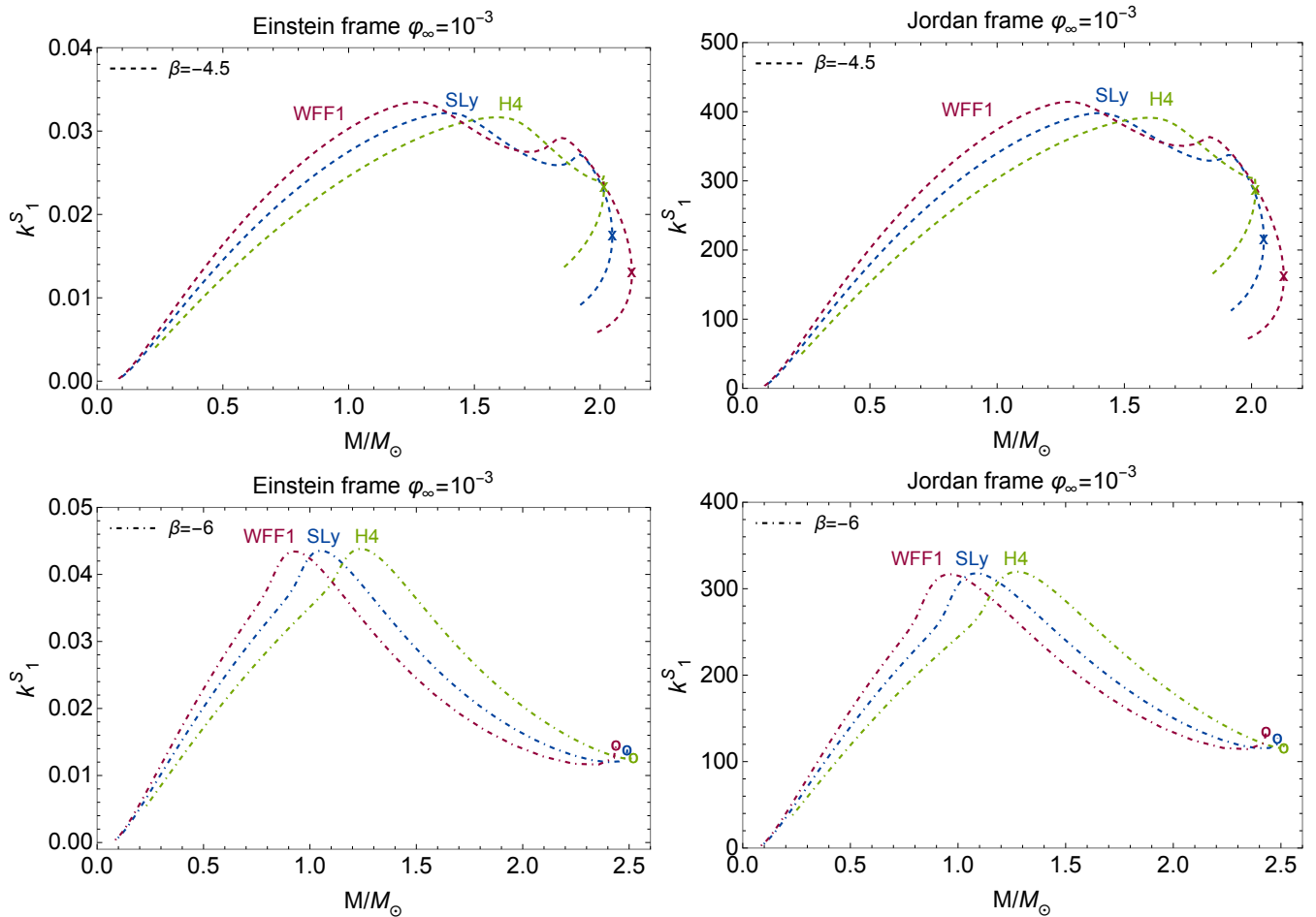
FIG. 16. Dipolar scalar Love number k_1^S in the Einstein and Jordan frames for three equations of state (WFF1, SLy and H4). The Jordan frame plots use the Jordan frame mass. The dashed and dot-dashed lines are the scalarized configurations with \beta = -4.5 and \beta = -6 , respectively. The cross represents the maximum mass configuration for \beta = 0, -4.5 , and the circle for \beta = -6 . For \beta = -6 we have omitted the data beyond the maximum mass configuration for better readability. All plots correspond to a scalar field at infinity \varphi_{0\infty} = 10^{-3} .
