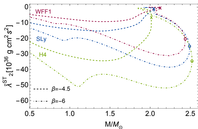
FIG. 10. Quadrupolar, scalar-field-independent scalar-tensor tidal deformabilities \tilde{\lambda}_2^{ST} in the Einstein frame for three equations of state (WFF1, SLy and H4). The dashed and dot-dashed lines are the scalarized configurations with \beta = -4.5 and \beta = -6 , respectively. The cross represents the maximum mass configuration for \beta = 0, -4.5 , and the circle for \beta = -6 .
