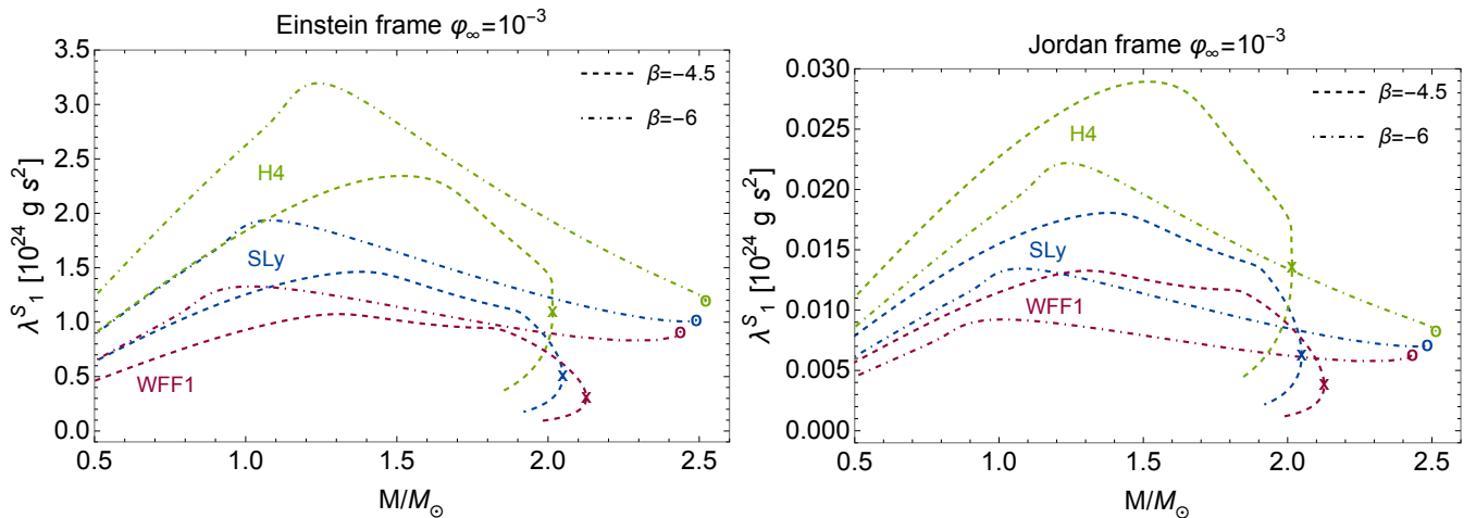
FIG. 6. Dipolar scalar tidal deformabilities \lambda_1^S in the Einstein and Jordan frames for three equations of state (WFF1, SLy and H4). The dashed and dot-dashed lines are the scalarized configurations with \beta = -4.5 and \beta = -6 , respectively. For \beta = -6 we have omitted the data beyond the maximum mass configuration for better readability. The cross represents the maximum mass configuration for \beta = 0, -4.5 , and the circle for \beta = -6 . All plots correspond to a scalar field at infinity \varphi_{0\infty} = 10^{-3} .
