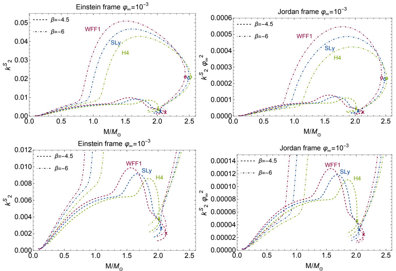
FIG. 21. Quadrupolar scalar Love numbers k_2^S in the Einstein and Jordan frames for three equations of state (WFF1, SLy and H4). The Jordan frame plots use the Jordan frame mass. The solid lines represent the GR configurations \beta = 0 and the dashed and dot-dashed lines are the scalarized configurations with \beta = -4.5 and \beta = -6 , respectively, and the plots in the bottom panels are zoomed with respect to their counterparts in the top panels. The cross represents the maximum mass configuration for \beta = 0, -4.5 , and the circle for \beta = -6 . All plots correspond to a scalar field at infinity \varphi_{0\infty} = 10^{-3} .
