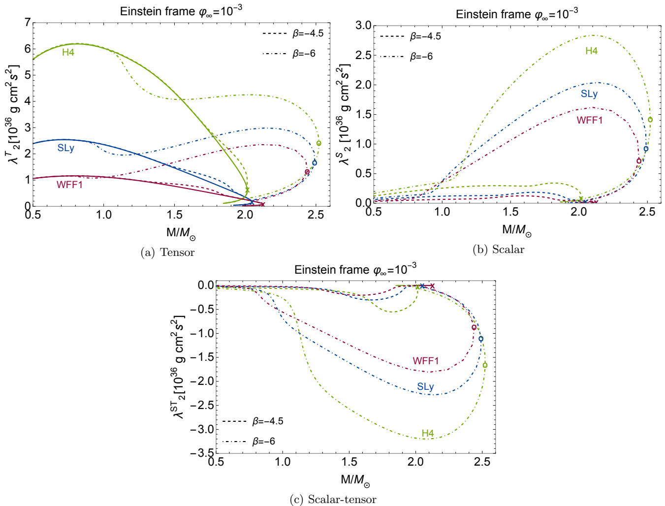
FIG. 7. Quadrupolar tidal deformabilities \lambda_2 in the Einstein frame for three equations of state (WFF1, SLy and H4). The solid lines represent the GR configurations \beta = 0 and the dashed and dot-dashed lines are the scalarized configurations with \beta = -4.5 and \beta = -6 , respectively. The plot corresponds to a scalar field at infinity \varphi_{0\infty} = 10^{-3} . The cross represents the maximum mass configuration for \beta = 0, -4.5 , and the circle for \beta = -6 . The corresponding results in the Jordan frame shown in Appendix D are qualitatively similar, the tensor Love numbers are the same in both frames (see (3.28a)), while the scalar and scalar-tensor ones are about two orders of magnitude smaller in the Jordan frame.
