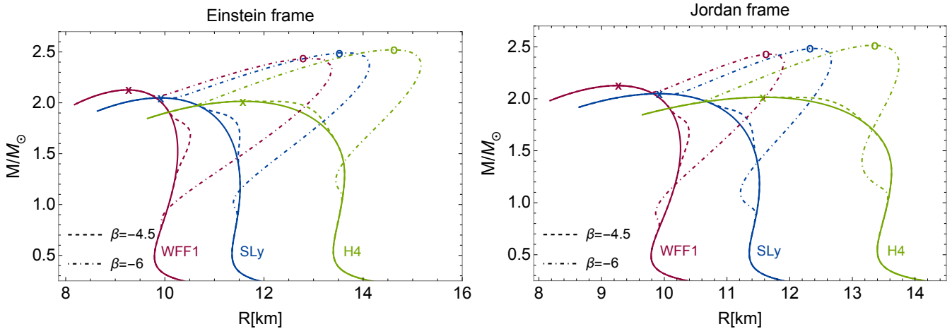
FIG. 4. Mass-Radius curves in the Einstein (left panel) and Jordan frames (right panel) for three equations of state (WFF1, SLy and H4). The solid lines represent the GR configurations \beta = 0 and the dashed and dot-dashed lines are the scalarized configurations with \beta = -4.5 and \beta = -6 , respectively. The cross represents the maximum mass configuration for \beta = 0, -4.5 , and the circle for \beta = -6 . Both plots correspond to a scalar field at infinity \varphi_{0\infty} = 10^{-3} .
