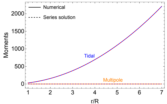
FIG. 2. Overlap between series expansion at infinity (dashed lines) and numerical solutions (solid lines) for the tidal (blue and red) and multipole (orange and purple) moments. For illustrative purposes we choose a quadrupolar configuration with WFF1 EoS, M = 1.16M_\odot , R = 10.16\text{km} , \beta = -4.5 and \varphi_\infty = 10^{-3} ; results for other configurations are similar.
