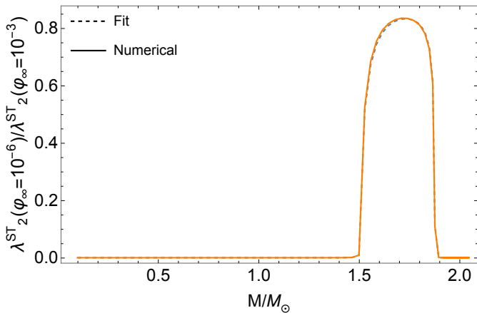
FIG. 9. Ratio of scalar-tensor tidal deformabilities computed for \varphi_\infty = 10^{-6} and \varphi_\infty = 10^{-3} . The solid line is the numerical result and the dashed line is the ratio using the linear fit to the polynomial w(\varphi_\infty, q) .
