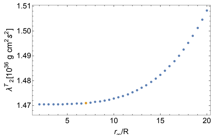
FIG. 3. Quadrupolar tensor tidal deformability \lambda_2^T in the Einstein frame as a function of r_\infty . The orange point is the chosen one for the integration. For illustrative purposes we choose a configuration with WFF1 EoS, M = 1.16M_\odot , R = 10.16\text{km} , \beta = -4.5 and \varphi_\infty = 10^{-3} ; other choices yield similar results.
