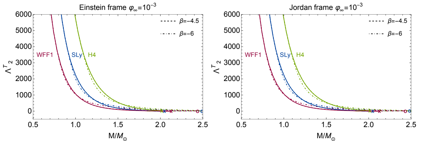
FIG. 17. Quadrupolar tensor adimensional tidal deformabilities \Lambda_2^T in the Einstein and Jordan frames for three equations of state (WFF1, SLy and H4). The Jordan frame plots use the Jordan frame mass. The solid lines represent the GR configurations \beta = 0 and the dashed and dot-dashed lines are the scalarized configurations with \beta = -4.5 and \beta = -6 , respectively. The cross represents the maximum mass configuration for \beta = 0, -4.5 , and the circle for \beta = -6 . Both plots correspond to a scalar field at infinity \varphi_{0\infty} = 10^{-3} .
