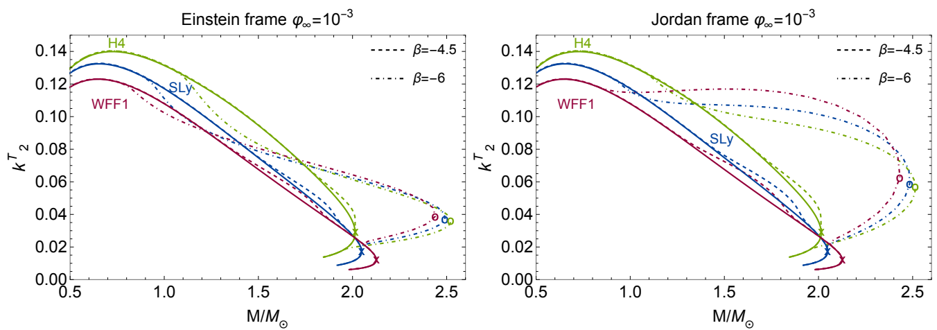
FIG. 20. Quadrupolar tensor Love numbers k_2^T in the Einstein and Jordan frames for three equations of state (WFF1, SLy and H4). The Jordan frame plots use the Jordan frame mass. The solid lines represent the GR configurations \beta = 0 and the dashed and dot-dashed lines are the scalarized configurations with \beta = -4.5 and \beta = -6 , respectively. The cross represents the maximum mass configuration for \beta = 0, -4.5 , and the circle for \beta = -6 . Both plots correspond to a scalar field at infinity \varphi_{0\infty} = 10^{-3} .
