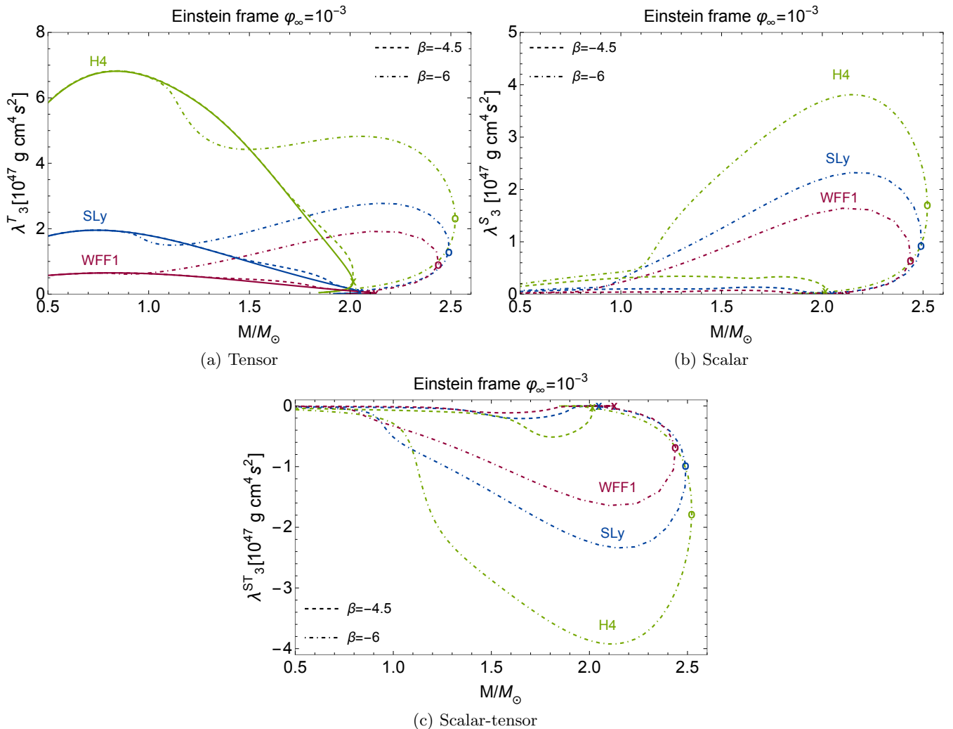
FIG. 8. Octupolar tensor tidal deformability \lambda_3^T in the Einstein frame for three equations of state (WFF1, SLy and H4). The solid lines represent the GR configurations \beta = 0 and the dashed and dot-dashed lines are the scalarized configurations with \beta = -4.5 and \beta = -6 , respectively. The cross represents the maximum mass configuration for \beta = 0, -4.5 , and the circle for \beta = -6 . The plot corresponds to a scalar field at infinity \varphi_{0\infty} = 10^{-3} . The corresponding results in the Jordan frame shown in Appendix D are qualitatively similar, the tensor Love numbers are the same in both frames (see (3.28a)), while the scalar and scalar-tensor ones are about two orders of magnitude smaller in the Jordan frame.
