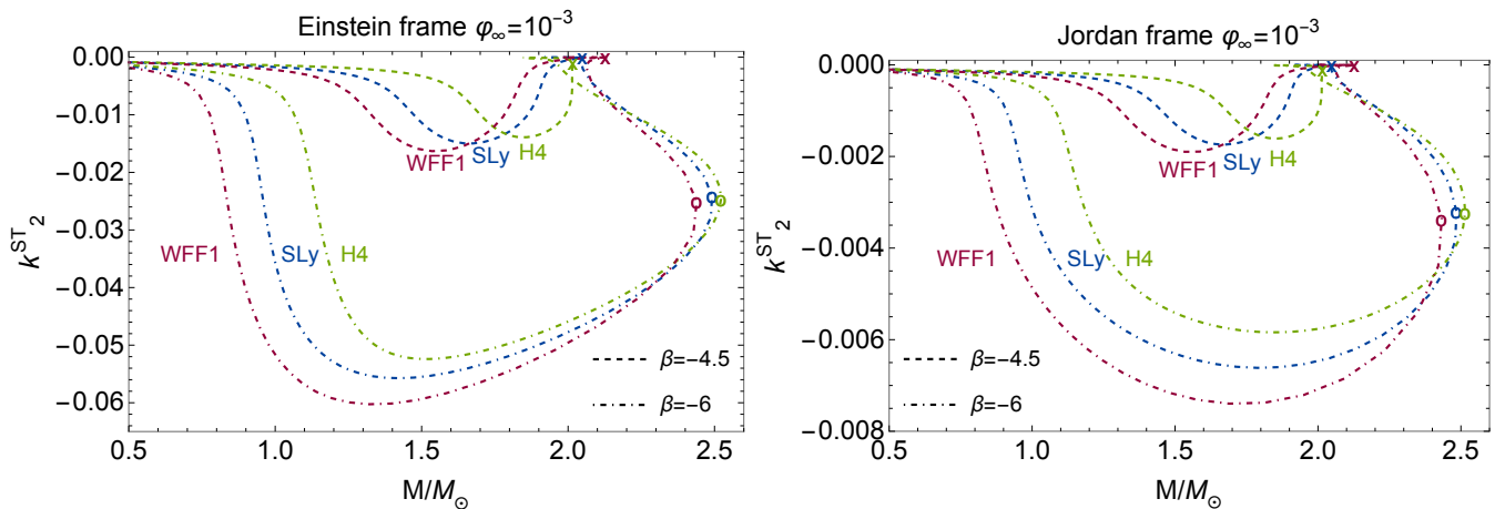
FIG. 22. Quadrupolar scalar-tensor Love numbers k_2^{ST} in the Einstein and Jordan frames for three equations of state (WFF1, SLy and H4). The Jordan frame plots use the Jordan frame mass. The solid lines represent the GR configurations \beta = 0 and the dashed and dot-dashed lines are the scalarized configurations with \beta = -4.5 and \beta = -6 , respectively. The cross represents the maximum mass configuration for \beta = 0, -4.5 , and the circle for \beta = -6 . Both plots correspond to a scalar field at infinity \varphi_{0\infty} = 10^{-3} .
