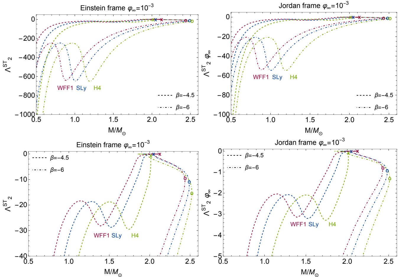
FIG. 19. Quadrupolar scalar-tensor adimensional tidal deformabilities \Lambda_2^{ST} in the Einstein and Jordan frames for three equations of state (WFF1, SLy and H4). The Jordan frame plots use the Jordan frame mass. The solid lines represent the GR configurations \beta = 0 and the dashed and dot-dashed lines are the scalarized configurations with \beta = -4.5 and \beta = -6 , respectively, and the plots in the bottom panels are zoomed with respect to their counterparts in the top panels. The cross represents the maximum mass configuration for \beta = 0, -4.5 , and the circle for \beta = -6 . All plots correspond to a scalar field at infinity \varphi_{0\infty} = 10^{-3} .
