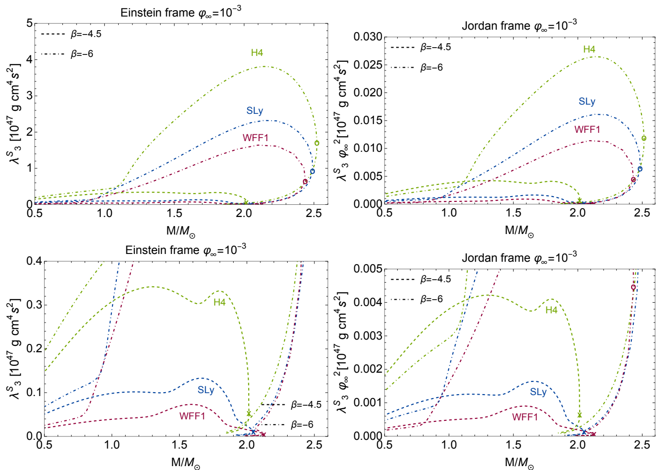
FIG. 13. Octupolar scalar tidal deformabilities \lambda_3^S in the Einstein and Jordan frames for three equations of state (WFF1, SLy and H4). The Jordan frame plots use the Jordan frame mass. The dashed and dot-dashed lines are the scalarized configurations with \beta = -4.5 and \beta = -6 , respectively, and the plots in the bottom panels are zoomed with respect to their counterparts in the top panels. The cross represents the maximum mass configuration for \beta = 0, -4.5 , and the circle for \beta = -6 . All plots correspond to a scalar field at infinity \varphi_{0\infty} = 10^{-3} .
