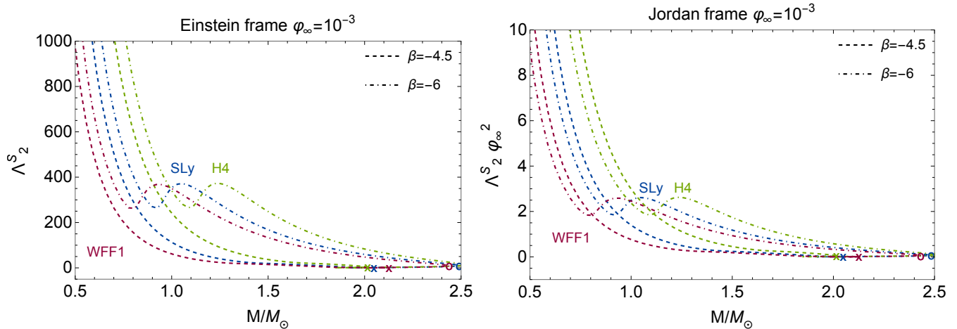
FIG. 18. Quadrupolar scalar adimensional tidal deformabilities \Lambda_2^S in the Einstein and Jordan frames for three equations of state (WFF1, SLy and H4). The Jordan frame plots use the Jordan frame mass. The dashed and dot-dashed lines are the scalarized configurations with \beta = -4.5 and \beta = -6 , respectively. The cross represents the maximum mass configuration for \beta = 0, -4.5 , and the circle for \beta = -6 . Both plots correspond to a scalar field at infinity \varphi_{0\infty} = 10^{-3} .
