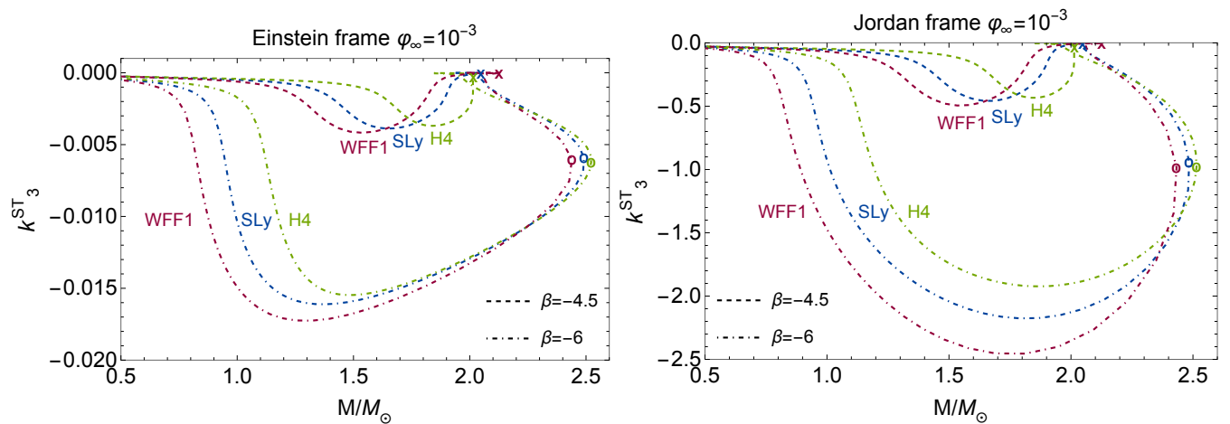
FIG. 28. Octupolar scalar-tensor Love numbers k_3^{ST} in the Einstein and Jordan frames for three equations of state (WFF1, SLy and H4). The Jordan frame plots use the Jordan frame mass. The solid lines represent the GR configurations \beta = 0 and the dashed and dot-dashed lines are the scalarized configurations with \beta = -4.5 and \beta = -6 , respectively. The cross represents the maximum mass configuration for \beta = 0, -4.5 , and the circle for \beta = -6 . Both plots correspond to a scalar field at infinity \varphi_{0\infty} = 10^{-3} .
