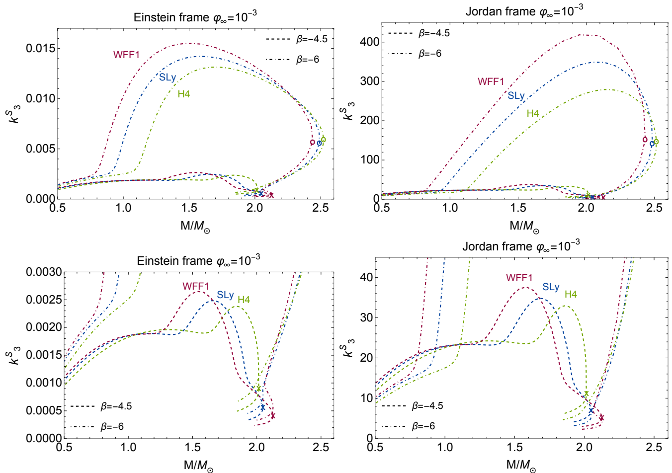
FIG. 27. Octupolar scalar Love numbers k_3^S in the Einstein and Jordan frames for three equations of state (WFF1, SLy and H4). The Jordan frame plots use the Jordan frame mass. The solid lines represent the GR configurations \beta = 0 and the dashed and dot-dashed lines are the scalarized configurations with \beta = -4.5 and \beta = -6 , respectively, and the plots in the bottom panels are zoomed with respect to their counterparts in the top panels. The cross represents the maximum mass configuration for \beta = 0, -4.5 , and the circle for \beta = -6 . All plots correspond to a scalar field at infinity \varphi_{0\infty} = 10^{-3} .
