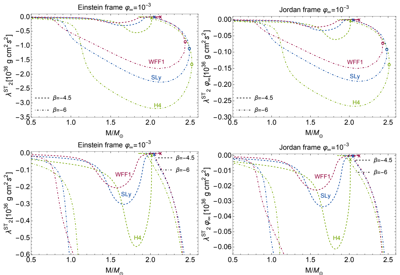
FIG. 12. Quadrupolar scalar-tensor tidal deformabilities \lambda_2^{ST} in the Einstein and Jordan frames for three equations of state (WFF1, SLy and H4). The Jordan frame plots use the Jordan frame mass. The dashed and dot-dashed lines are the scalarized configurations with \beta = -4.5 and \beta = -6 , respectively, and the plots in the bottom panels are zoomed with respect to their counterparts in the top panels. The cross represents the maximum mass configuration for \beta = 0, -4.5 , and the circle for \beta = -6 . The bottom plots are zoomed with respect to their top counterparts. All plots correspond to a scalar field at infinity \varphi_{0\infty} = 10^{-3} .
