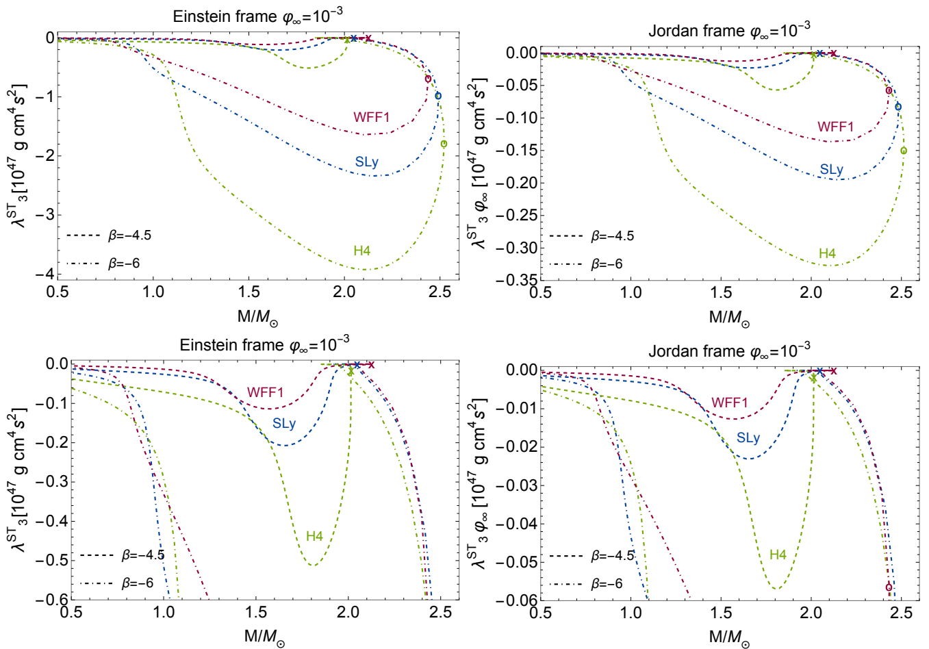
FIG. 14. Octupolar scalar-tensor tidal deformabilities \lambda_3^{ST} in the Einstein and Jordan frames for three equations of state (WFF1, SLy and H4). The Jordan frame plots use the Jordan frame mass. The dashed and dot-dashed lines are the scalarized configurations with \beta = -4.5 and \beta = -6 , respectively, and the plots in the bottom panels are zoomed with respect to their counterparts in the top panels. The cross represents the maximum mass configuration for \beta = 0, -4.5 , and the circle for \beta = -6 . All plots correspond to a scalar field at infinity \varphi_{0\infty} = 10^{-3} .
