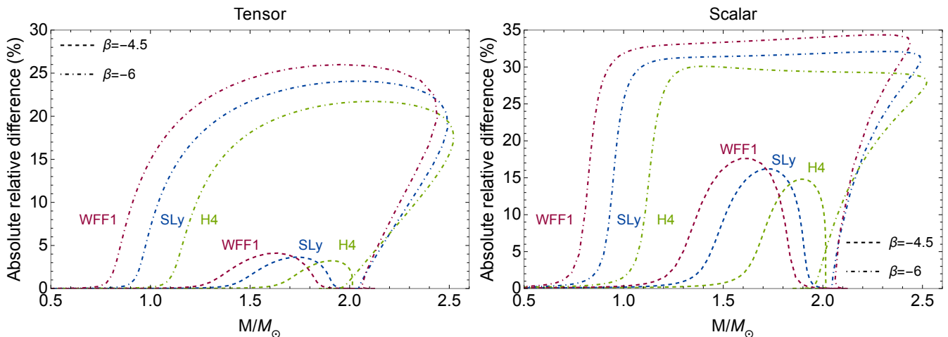
FIG. 29. Absolute relative difference between the tensor (left) and scalar (right) quadrupolar tidal deformabilities computed with and without setting the source term in the perturbation equations of motion to zero. The mass is the ADM mass in the Einstein frame. We consider three equations of state (WFF1, SLy and H4) and the dashed and dot-dashed lines are the scalarized configurations with \beta = -4.5 and \beta = -6 , respectively. We set a scalar field at infinity \varphi_{0\infty} = 10^{-3} .
