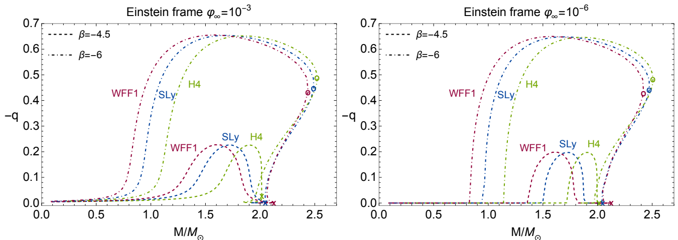
FIG. 5. Charge-Mass curves in the Einstein frame for three equations of state (WFF1, SLy and H4) and a scalar field at infinity \varphi_{0\infty} = (10^{-3}, 10^{-6}) . The dashed and dot-dashed lines are the scalarized configurations with \beta = -4.5 and \beta = -6 , respectively. The cross represents the maximum mass configuration for \beta = 0, -4.5 , and the circle for \beta = -6 .
