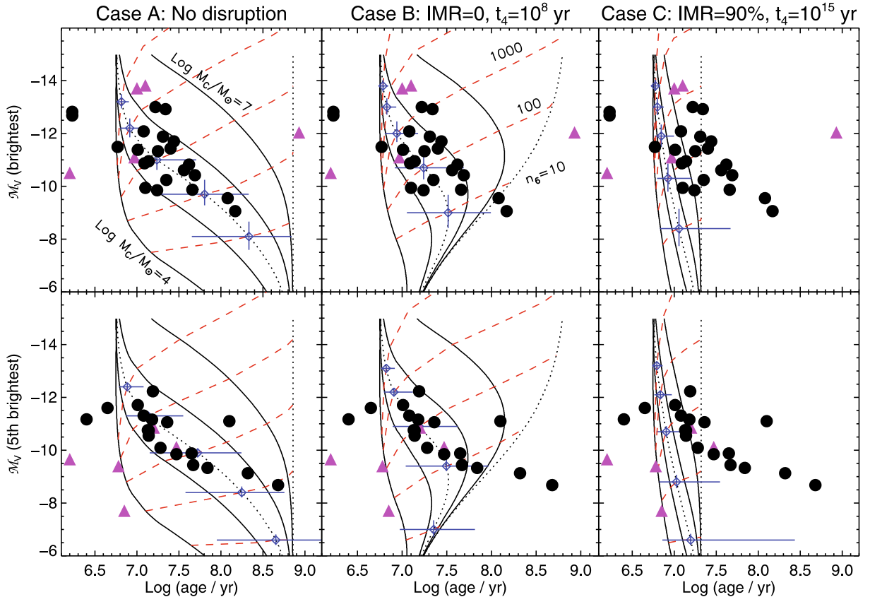
Fig. 4. The median absolute magnitude of the brightest ( top ) and 5th brightest ( bottom ) cluster versus median age. Results are shown for Schechter mass functions with M_c = 10^4, 10^5, 10^6 and 10^7 M_\odot and \alpha = -2 (solid curves), as well as for M_c = 3 \times 10^5 M_\odot and M_c = 10^{15} M_\odot (dotted curves). The (red) dashed lines are for constant total number of clusters ( n_6 = 10^1, 10^2, \dots, 10^5 ) brighter than M_V = -6 . The error bars mark the median absolute deviation of \log(\text{age}) and M_V for fixed M_c and n_6 . The triangles mark clusters in irregular galaxies while circles are for spirals (see Table 1).
