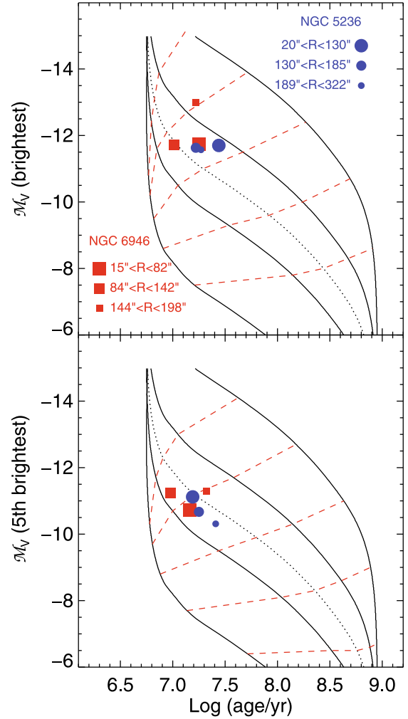
Fig. 5. M_V versus log age for the brightest and 5th brightest clusters in radial sub-samples in NGC 5236 and NGC 6946. In each galaxy, each radial bin contains an equal number of clusters. The model lines are the same as for the Case A scenario in Fig. 4.
