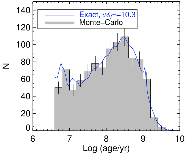
Fig. 3. Age distribution of the brightest cluster for M_c = 10^6 M_\odot and N = 10^4 . The histogram is for the N = 10^4 Monte-Carlo simulation in Fig. 2 while the solid (blue) curve shows the exact relation according to Eq. (7) for M_V = -10.3 mag.
