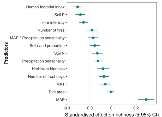
Figure 1. Determinants of tree species richness in the woodlands of eastern and southern Africa. Standardised effect sizes are shown for each variable included in the negative binomial regression model. Points and lines show the mean and 95% credible intervals (CI) respectively. Points to the left of the dashed line had a negative effect on species richness, whilst those to the right had a positive effect.
