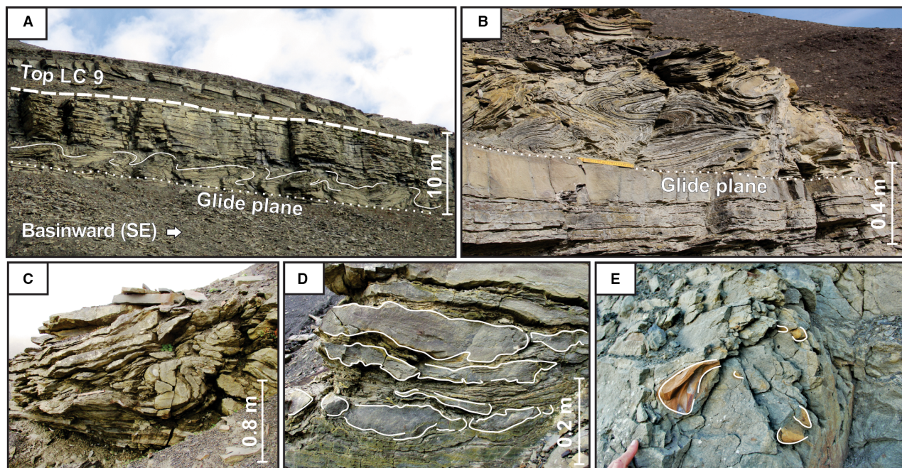
Fig. 11. Representative pictures of mass-transport deposits (MTD). (A) Typical expression of several metre-scale basinward-directed folds within thin-bedded heterolithic lobe fringe deposits of LC 9 at Storvola (MTD1). These MTD represent local slide events, which apparently did not evolve into a full-scale slump. (B) Decimetre-scale slump folds occur locally within thin-bedded heterolithic fringe and distal fringe deposits, and in proximity to channel margins (MTD2). These deposits record minor slides and slumps (of very limited run-out) associated with instability promoted by local relief. The example is from the channel-lobe transition zone of LC 10 at Storvola. (C) to (E) Examples of a laterally complex and chaotic MTD within LC 12 at Hyrnestabben. This particular MTD exhibits multiple lateral transitions between segments that record sliding with limited deformation (mostly folding; C), via units that contain abundant disintegrated and faulted strata due to increased shear-related deformation (D) to fully disintegrated debris-flow deposits (E). Bed type details are given in Fig. 7D.
