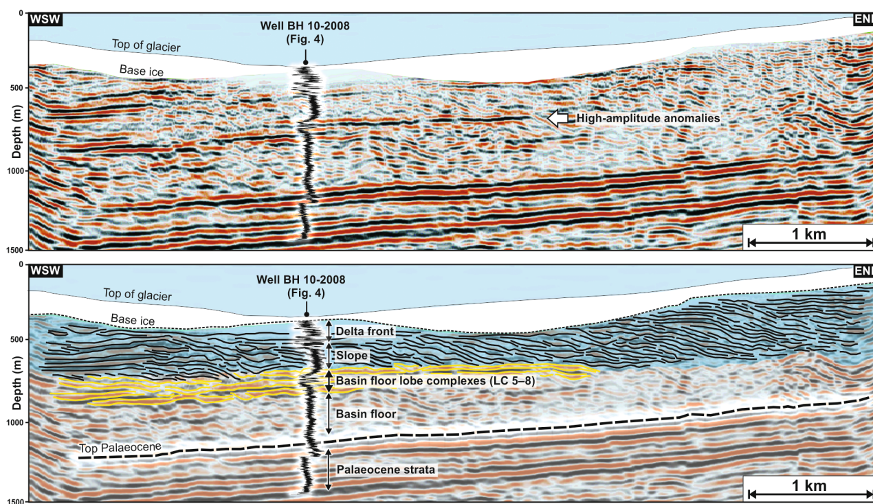
Fig. 5. Two-dimensional reflection seismic data from Sysselmannbreen. The line crosses Well BH 10-2008. See Fig. 1C for location. (A) Uninterpreted seismic line tied to the gamma-ray log of Well BH 10-2008. Note the presence of high-amplitude reflection anomalies exhibiting an offset stacking pattern towards the ENE (i.e. basinward), and how these anomalies correlate to an interval of serrated and blocky gamma ray signatures in the well (details shown in Fig. 4B). (B) Interpreted seismic line, showing a basinward-prograding slope succession, which partly connects with and overlies the progradationally-stacked series of lobe complexes. The interpretation is modified from Grundvåg et al. (2014a), based on Johannessen et al. (2011). The seismic data is from Johansen et al. (2011).
