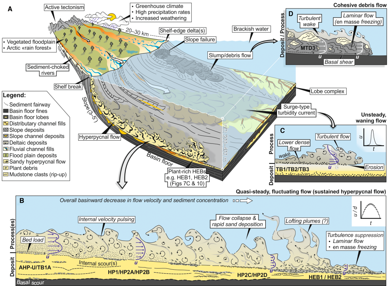
Fig. 18. (A) Palaeogeographical reconstruction highlighting the most important allogenic forcing factors that facilitated the establishment of a hyperpycnal flow-dominated supply system. Collectively, favourable climatic conditions (leading to high rates of sediment supply), shelf-edge positioned river mouths, brackish water conditions in the basin and steep slopes promoted transfer of sand onto the deep-water basin floor, foremost via river-derived hyperpycnal flows. Turbidity currents triggered by other mechanisms, such as delta front failure, as well as slope instability-related slumping, played subordinate roles. WSFTB: West Spitsbergen fold-and-thrust belt. (B) Conceptual model showing the main components of a river-derived hyperpycnal flow and the composite character of its depositional product. See main text for explanation and Fig. 7 for more details on the different bed types. (C) Main components of a surge-type, waning turbidity current. These currents deposit ‘classical’ Bouma-type turbidites (i.e. TB1 to TB3, Fig. 7). (D) The main characteristics of a slump-derived cohesive debris flow and the resultant deposit (MTD3; Fig. 7). Deposition occurs via en masse freezing of the flow plug. Abbreviations: c – concentration, d – discharge, t – time, u – velocity.
