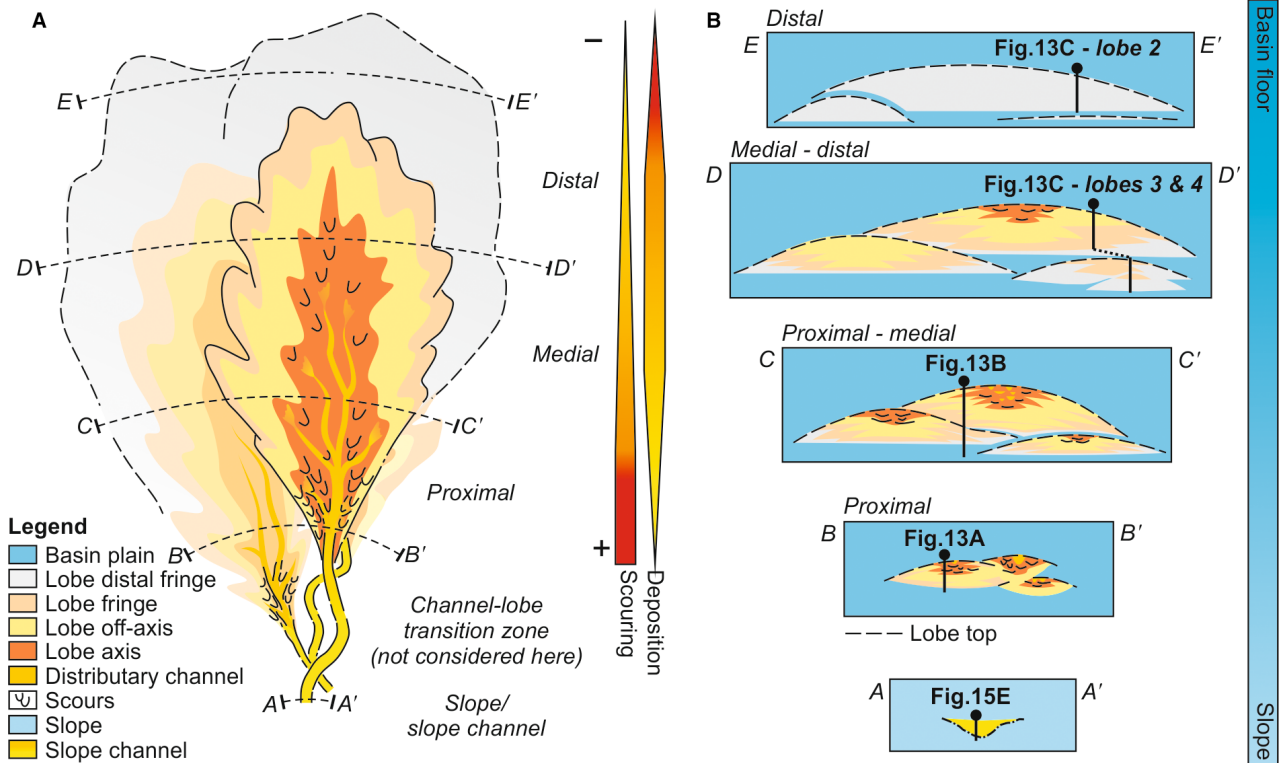
Fig. 12. Schematic illustration of a lobe complex. (A) Plan-view architecture of a lobe complex showing the aerial distribution of lobe axis, lobe off-axis, lobe fringe and lobe distal fringe deposits. Scouring is most evident in the lobe axis. (B) Cross-sections showing the internal distribution of bed type associations from proximal to distal within a lobe complex consisting of a series of progradationally stacked lobes. The relative position of the logs shown in Figs 13 and 15 are indicated.
