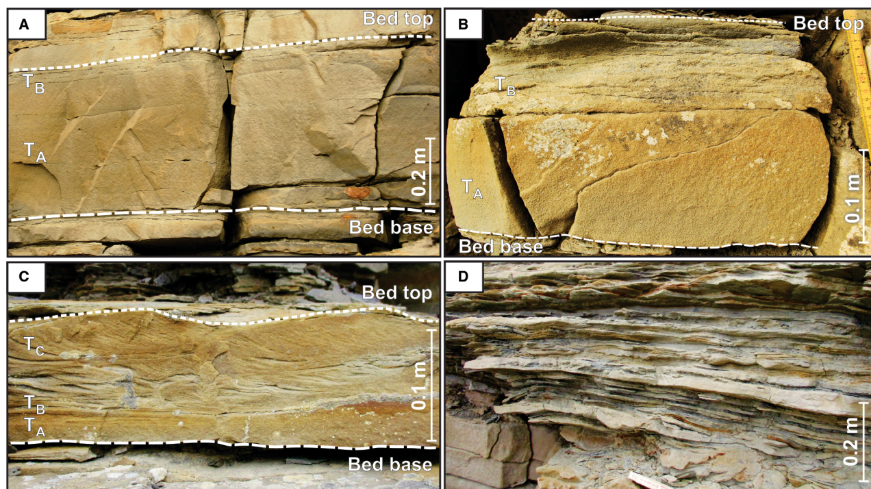
Fig. 9. Representative pictures of turbidite beds (TBs) exhibiting classical Bouma-type facies arrangements pointing to deposition under waning flow conditions. (A) A thick-bedded sandstone bed dominated by a massive lower division overlain by a thin, laminated upper division (bed type TB1C). (B) A medium-bedded sandstone exhibiting normal grading and a clear two-fold division with a plane parallel stratified upper division overlying a massive division (bed type TB2B). (C) A thin-bedded sandstone characterized by a poorly developed massive division, successively overlain by a plane parallel and a current-ripple cross-laminated division (bed type TB2C). (D) A heterolithic unit composed of interbedded mudstones and very thin sandstones beds exhibiting normal grading and occasionally plane parallel lamination to current-ripple cross-lamination (bed type TB3D). All photographs are from the Hyrnestabben lobe complexes. Bed type details are given in Fig. 7B.
