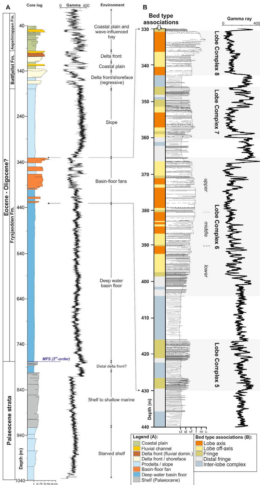
Fig. 4. Overview of the stratigraphy recorded in fully cored Well BH 10-2008 at Sysselmannbreen. The four investigated lobe complexes (LC 5 to LC 8) are embedded within the shales of the Frysjaodden Formation and show a clear progradational stacking trend (see Grundvåg et al., 2014a, for more details).
