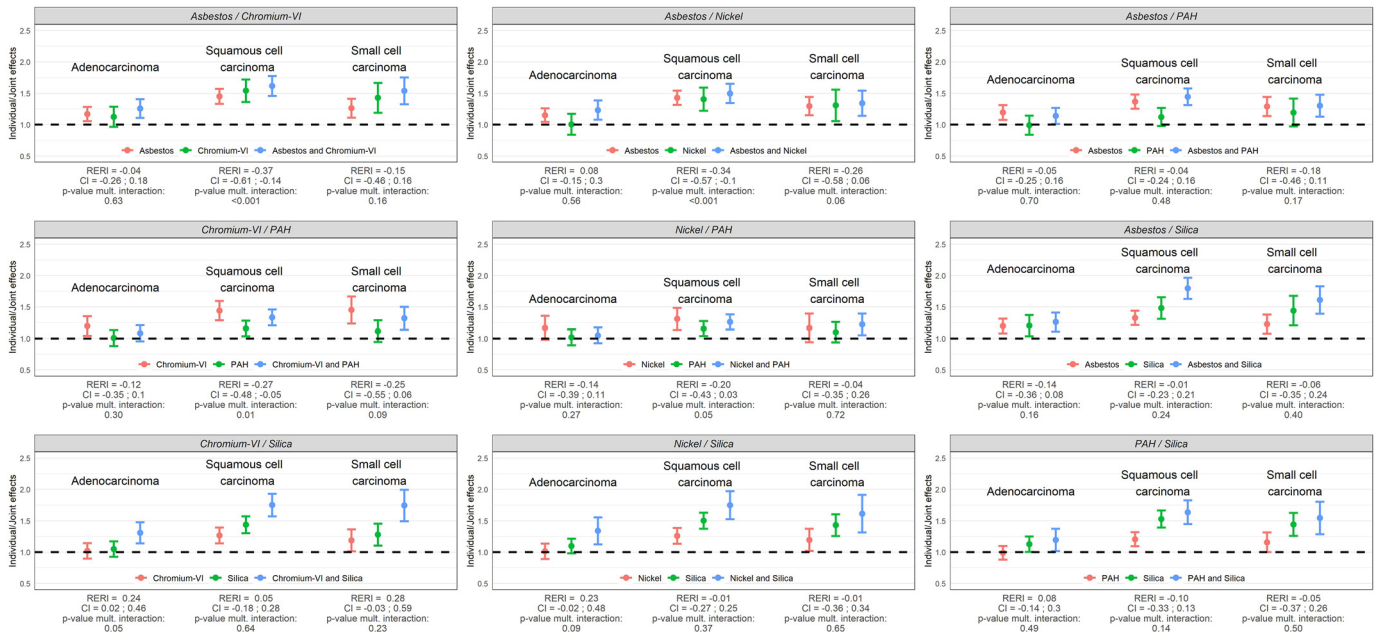
Figure 3. Individual and joint effects (ORs) of occupational exposures, RERIs, and tests for multiplicative interaction ( p -values) between occupational exposures in relation to major histological subtypes of lung cancer in SYNERGY for men ( n = 11,353 lung cancer cases and n = 16,451 control subjects). Note: CI, confidence interval; OR, odds ratio; PAH, polycyclic aromatic hydrocarbons; RERI, relative excess risk due to interaction.
