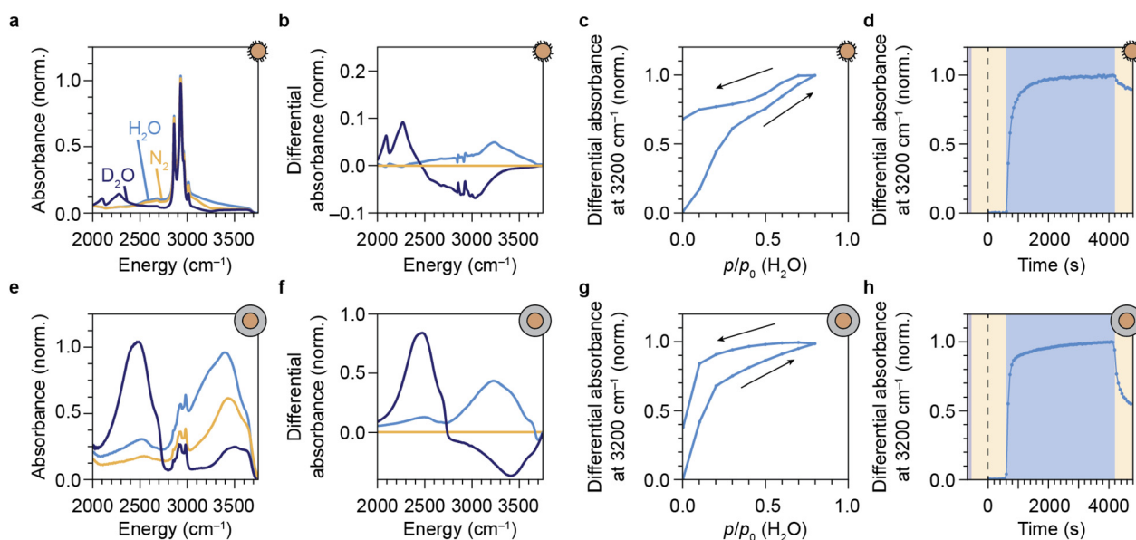
Fig. 4 Monitoring the adsorption of water vapor with ATR-FTIR spectroscopy. (a) Infrared absorption spectra of a layer of oleic-acid-coated \text{NaYF}_4 : \text{Er}^{3+} (2%), \text{Yb}^{3+} (18%) NCs, under dry \text{N}_2 flow (yellow), and under flows of p/p_0 = 0.20 \text{H}_2\text{O} (blue) and \text{D}_2\text{O} (purple). (b) Differential infrared absorption spectra, relative to the absorption under dry \text{N}_2 flow. (c) Differential absorbance at 3200\text{ cm}^{-1} as a function of the relative water pressure p/p_0 ( \text{H}_2\text{O} ). Arrows indicate the adsorption and desorption isotherms. (d) Normalized differential absorbance at 3200\text{ cm}^{-1} , measured under dry nitrogen flow (yellow-shaded areas) or in the presence of water vapor ( p/p_0 = 0.17 ; blue-shaded area). The sample was purged with \text{D}_2\text{O} vapor before starting the experiment. (e–h) Same as a–d, but for \text{SiO}_2 -coated NCs.
