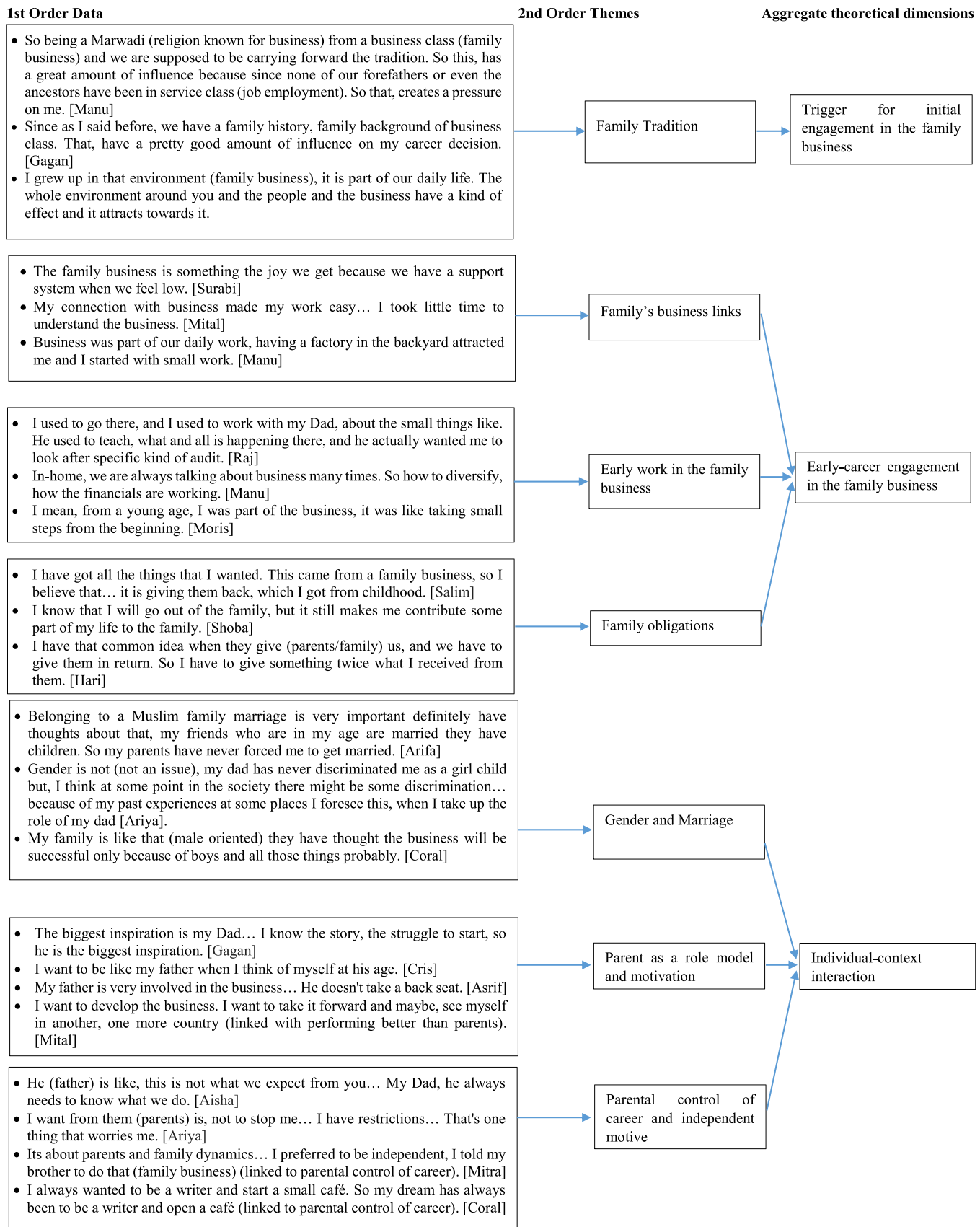
Fig. 1. Data Structure.
