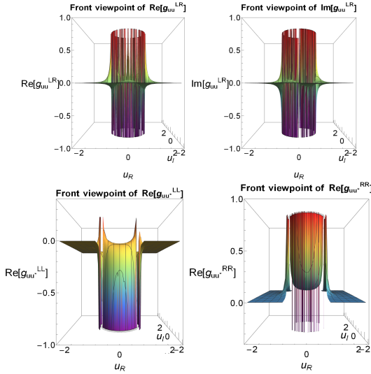
FIG. 9. \text{Re}[g_{uu}^{LR}] , \text{Im}[g_{uu}^{LR}] , \text{Re}[g_{uu}^{LL}] and \text{Re}[g_{uu}^{RR}] in the parameter space u_R, u_I \in \mathbb{R} for N = 200 . \text{Im}[g_{uu}^{LL}] \approx 0 and \text{Im}[g_{uu}^{RR}] \approx 0 due to finite-size effects.
