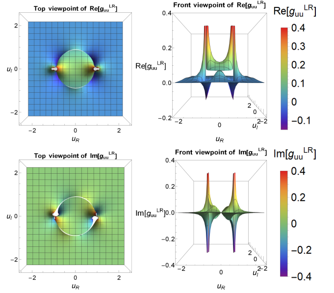
FIG. 7. Real and imaginary parts of the QMT component g_{uu}^{LR} in the parameter space \{u_R, u_I\} \in \mathbb{R} for N \rightarrow \infty .
