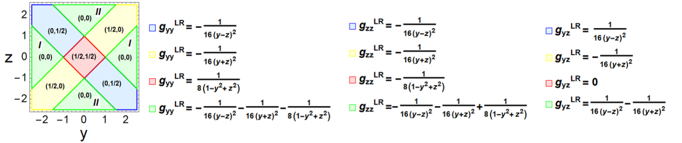
FIG. 5. The phase diagram with associated metric components g_{yy}^{LR} , g_{zz}^{LR} and g_{yz}^{LR} in the parameter space y, z \in \mathbb{R} . The symmetry by exchanging x^\mu \rightarrow -x^\mu relies on the metric equation ds^2 = g_{\mu\nu}^{LR} d\lambda^\mu d\lambda^\nu , where the line element also has the negative sign, instead of the QMT itself. This domain matches perfectly with the topological phase diagram found by using a more conventional method in Refs. [14, 37]. Different topological phases are distinguished by colours and the two-component winding number (\nu_1, \nu_2) . Hermitian topological phases have \nu_1 = \nu_2 , while \nu_1 \neq \nu_2 only happens for NH regimes. Specifically, (0, 0) represents a Hermitian trivial phase, while (1/2, 1/2) is a Hermitian topological phase, and (0, 1/2) and (1/2, 0) represent NH topological phases. Notice that the Hermitian phase diagram is recovered when z = 0 .
