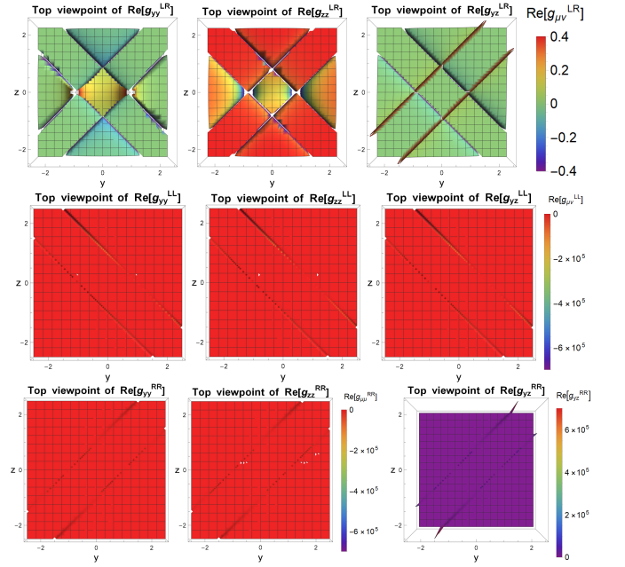
FIG. 8. \text{Re}[g_{\mu\nu}^{\alpha\beta}] with \alpha, \beta \in \{L, R\} in the parameter space \lambda^\mu, \lambda^\nu \in \{y, z\} \in \mathbb{R} for N = 200 . Top viewpoint.
