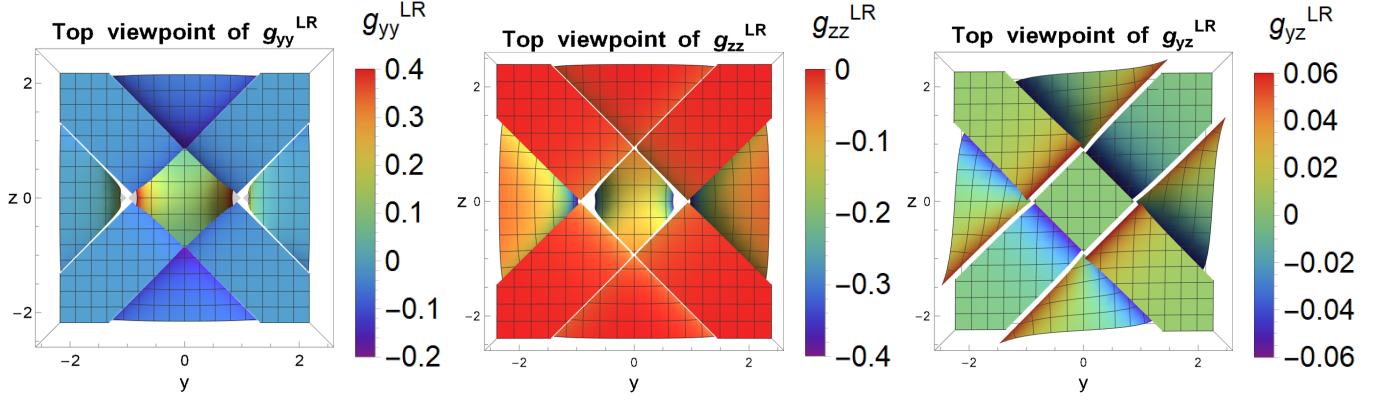
FIG. 4. QMT components \text{Re}[g_{\mu\nu}^{LR}] with x^\mu, x^\nu \in \{y, z\} in the parameter space y, z \in \mathbb{R} for N \rightarrow \infty . Top viewpoint. Their imaginary parts are zero: \text{Im}[g_{\mu\nu}^{LR}] = 0 \forall \lambda^\mu, \lambda^\nu \in \{y, z\} . Therefore g_{\mu\nu}^{LR} = \text{Re}[g_{\mu\nu}^{LR}] .
