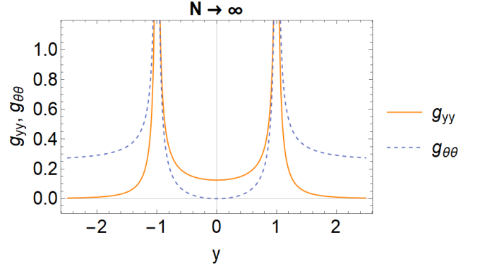
FIG. 6. g_{yy} and g_{\theta\theta} in the parameter space \{y \equiv t/t_2, \theta\} for N \rightarrow \infty (i.e. thermodynamic limit). Note that both QMT components are independent of the parameter \theta .
