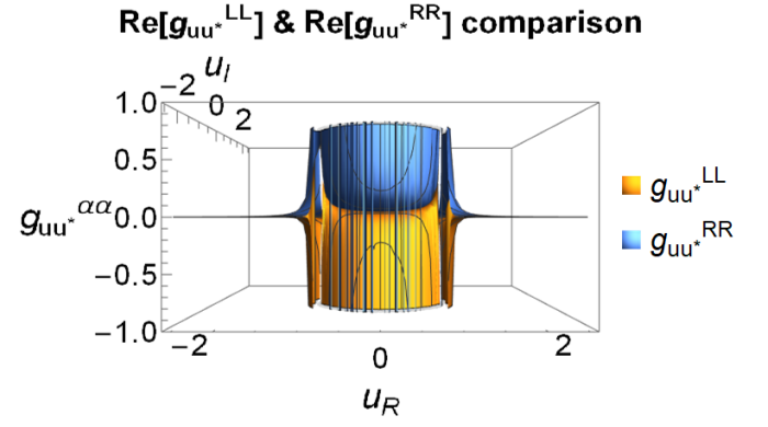
FIG. 10. Comparison between \text{Re}[g_{uu}^{LL}] and \text{Re}[g_{uu}^{RR}] in the parameter space u_R, u_I \in \mathbb{R} for N = 200 .
