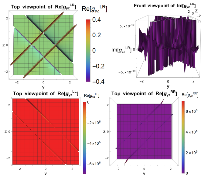
FIG. 3. The QMT components g_{yz}^{\alpha\beta} with \alpha, \beta \in \{L, R\} in the parameter space y, z \in \mathbb{R} for N = 200 . Their imaginary parts are non-zero (order 10^{-19} ) due to finite-size effects: \text{Im}[g_{\mu\nu}^{\alpha\beta}] \approx 0 \quad \forall \lambda^\mu, \lambda^\nu \in \{y, z\} . Note: keep in mind that g_{\mu\nu}^{\alpha\alpha} with \alpha \in \{L, R\} are not legitimate QMT components.
