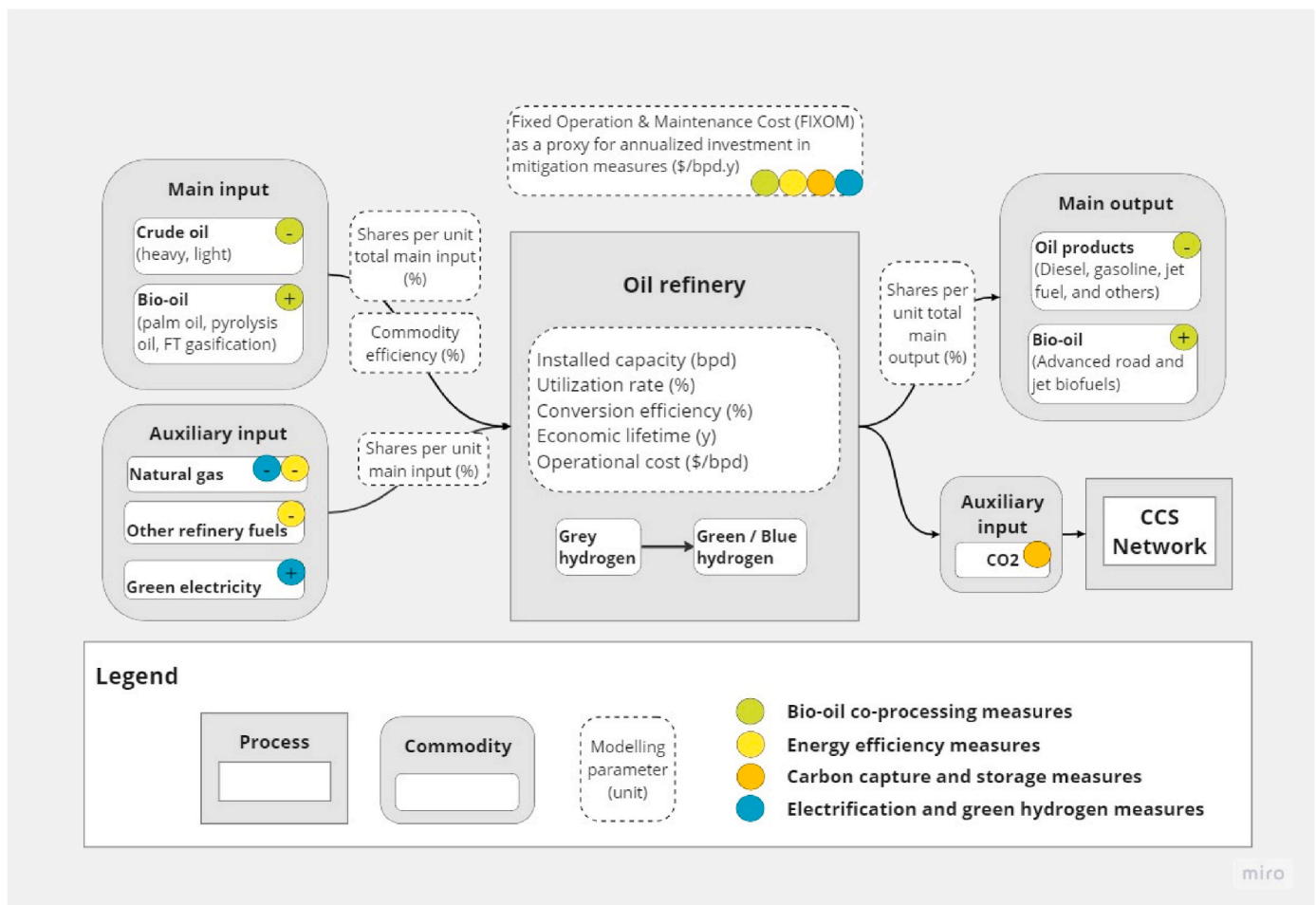
Fig. 6. Proposed parametrization to model the deployment of GHG mitigation options in an existing refinery.
