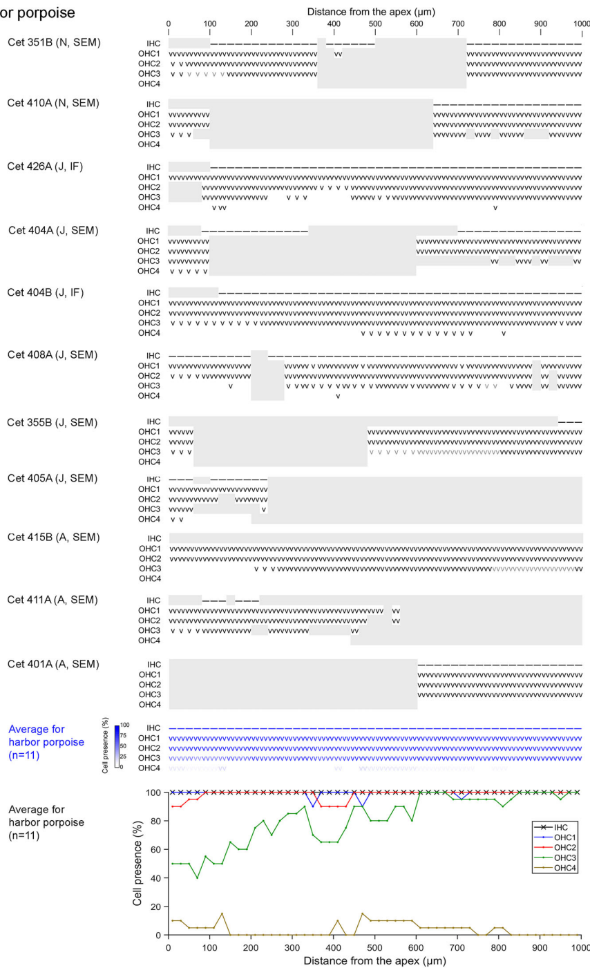
FIGURE 2 Schematic representation of the apex of the ears analyzed from harbor porpoise ( Phocoena phocoena ) and pygmy sperm whale ( Kogia breviceps ) for this study. The inner hair cells (IHCs) are labeled with a hyphen and the outer hair cells (OHCs) with a “V.” The gray shading represents regions where there was no information due to decomposition, cellular debris on the surface of the organ of Corti that impeded the visualization of the cells, or due to unintentional damage during the dissection or processing of the sample. The gray “V” represents areas where there was partial information of sensory cells, or they showed signs of decomposition making hair cell identification challenging. It is possible that there was a first region with no information of the organ of Corti in the pygmy sperm whale since it was challenging to determine its beginning. The averaged values for harbor porpoise are shown in blue and include percentages of cell presence. This representation corresponds to about half of the number of sensory cells found in the first millimeter of the apex
