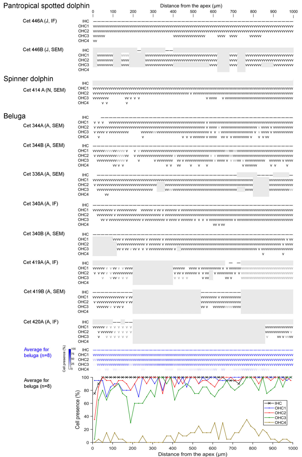
FIGURE 3 Schematic representation of the apex of the ears analyzed from pantropical spotted dolphin ( Stenella attenuata ), spinner dolphin ( Stenella longirostris ), and beluga whale ( Delphinapterus leucas ) for this study. The inner hair cells (IHCs) are labeled with a hyphen and the outer hair cells (OHCs) with a “V.” The gray shading represents regions where there was no information, due to decomposition, cellular debris on the surface of the organ of Corti that impeded the visualization of the cells, or due to unintentional damage during the dissection or processing of the sample. The gray “V” represents areas where there was partial information of sensory cells, or they showed signs of decomposition making hair cell identification challenging. The averaged values for beluga are shown in blue and include percentages of cell presence. This representation corresponds to about half of the number of sensory cells found in the first millimeter of the apex
