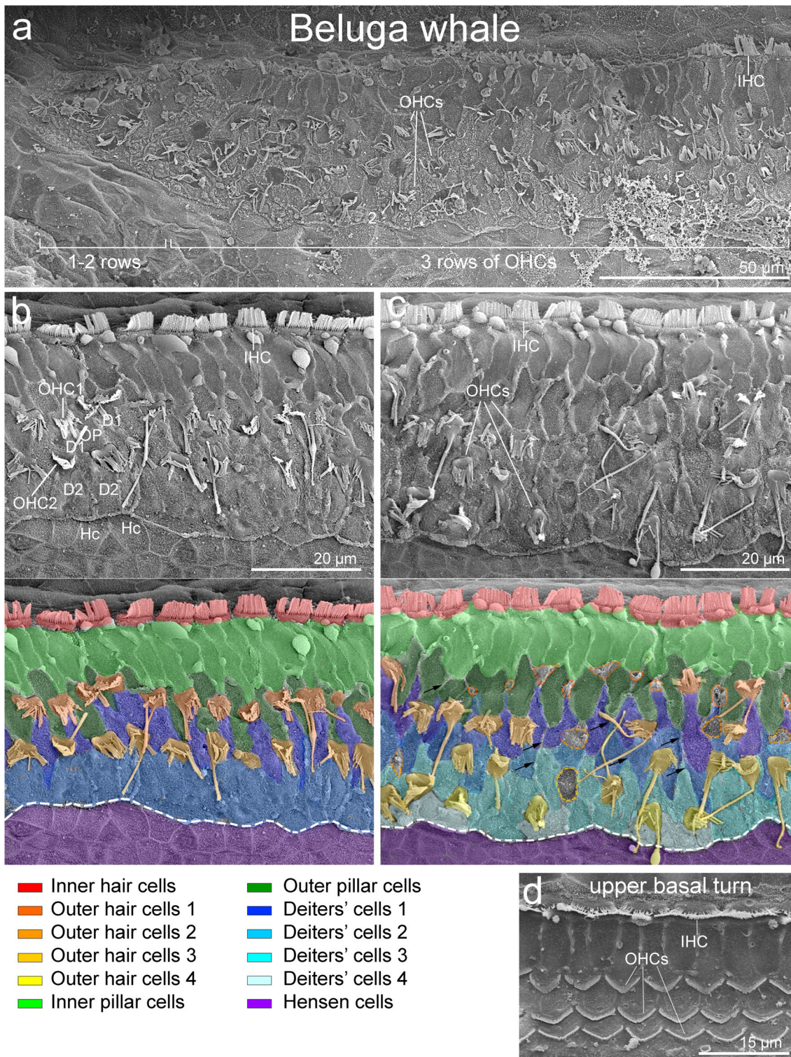
FIGURE 9 Scanning electron micrographs of the cochlea of adult belugas ( Delphinapterus leucas ) from the Canadian Arctic. (a) General image of the first 150 \mu\text{m} of the apex (located to the left) of the right ear from individual cet 336, fixed 3.25 hr postmortem and showing a pattern of one to two rows of outer hair cells (OHCs) in the first 30 \mu\text{m} , followed by a three-row pattern. (b,c) Close-up images of the left cochlea from individual cet 344, fixed between 2 and 3 hr postmortem. The narrow groove has been highlighted with a white dotted line. In (b), there is a region with two rows of OHCs, which also displays only two rows of Deiters' (D) cells. In (c), there are some missing OHCs (highlighted with arrows), which were typically observed to be missing from the third row in other species, but in the adult beluga examples, there was scattered loss of OHCs in the first and second row as well. There were potential remains of OHCs marked with a discontinued line. In (b,c), hair cells and supporting cells were colored in the panel below to highlight their arrangement within the organ of Corti. (d) Organ of Corti of the upper basal turn of the same individual as panel (a) for comparison. IHC, inner hair cell; OP, outer pillar cell
