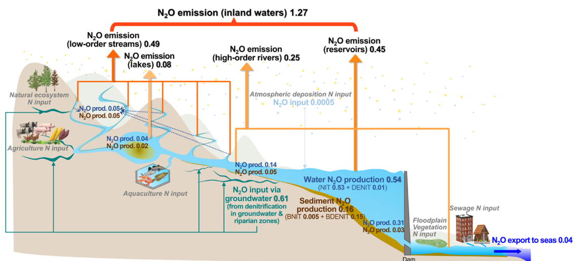
Figure 5. Global \text{N}_2\text{O} budget along the aquatic continuum from land to sea in 2010 (in \text{Tg N yr}^{-1} ). The blue and brown fonts indicate the net \text{N}_2\text{O} -production estimates in the water column and sediment, respectively. NIT and DENIT indicate the net inland-water \text{N}_2\text{O} production through nitrification and denitrification in the water column, respectively, and BNIT and BDENIT indicate those through nitrification and denitrification in sediment, respectively.
