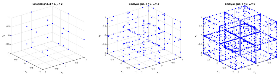
Fig. 2. Collocation points for the d = 3 case with varying level parameter \mu = 2, 4, 6 .
