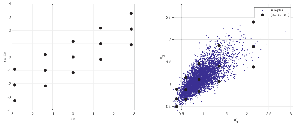
Fig. 8. LHS: 2D collocation points \hat{x}_{i_1} and \hat{x}_{i_2}|\hat{x}_{i_1} for \rho = 0.6 . RHS: Scatter plot for two lognormal random variables X_1 \sim e^{Z_1} and X_2 \sim e^{Z_2} where Z_1 \sim \mathcal{N}(-0.1, 0.3) , Z_2 \sim \mathcal{N}(0.2, 0.2) , N_1 = 5 , N_2 = 3 and \rho_{Z_1, Z_2} = 0.6 and the corresponding collocation points x_{i_1} and x_{i_2}|x_{i_1} .
