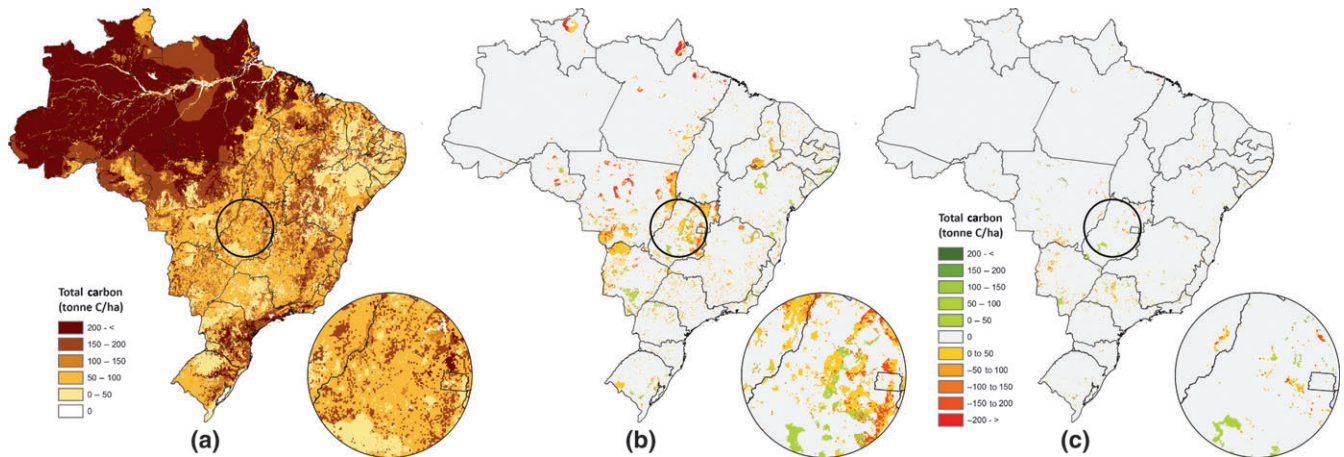
FIGURE 4 (a) Total carbon stock (above and below ground biomass and soil organic carbon) for the initial modelling year 2012, (b) the changes in carbon stock between 2012 and 2030 in the reference scenario without additional ethanol demand, and (c) the additional changes in carbon stock in 2030 in the reference scenario due to the additional ( +26 \times 10^9 L) ethanol demand (compared to 2030 without ethanol)
