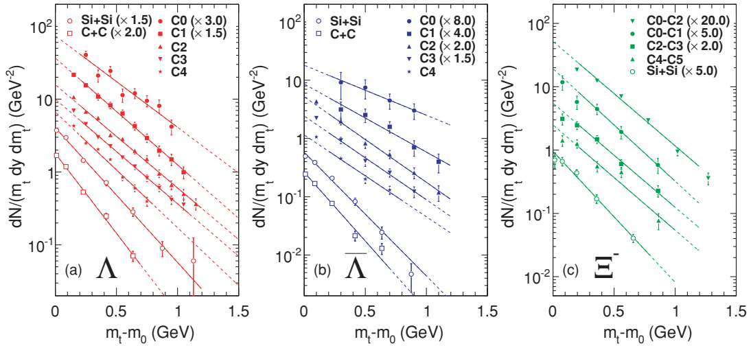
FIG. 5. (Color online) The transverse mass spectra of \Lambda (a), \bar{\Lambda} (b), and \Xi^- (c) at midrapidity ( \Lambda/\bar{\Lambda} : |y| < 0.4 , \Xi^- : |y| < 0.5 ) for Pb + Pb reactions at 158A GeV in different centrality bins, and in near-central C + C and Si + Si collisions at 158A GeV. Some of the data points are scaled for clarity. Only statistical errors are shown. The solid/dashed lines represent fits with an exponential, where the solid parts denote the m_t ranges in which the fits were performed. The \Lambda spectra for C + C and Si + Si are taken from Ref. [9].
