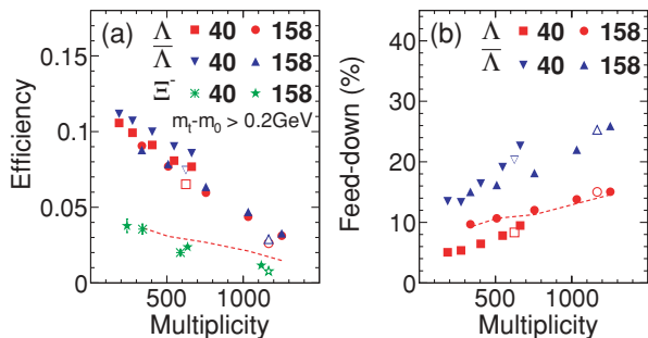
FIG. 2. (Color online) The p_t -integrated reconstruction efficiency (a) and feed-down contribution (b) at midrapidity ( \Lambda, \bar{\Lambda} : |y| < 0.4 , \Xi^- : |y| < 0.5 ) as a function of centrality as characterized by the measured charged track multiplicity for minimum bias Pb + Pb reactions at 40A and 158A GeV. Open symbols correspond to the values for central Pb + Pb collisions [8]. The dashed lines represent the \Lambda efficiency or feed-down contribution, respectively, at 158A GeV, resulting from a different analysis strategy (see text).
