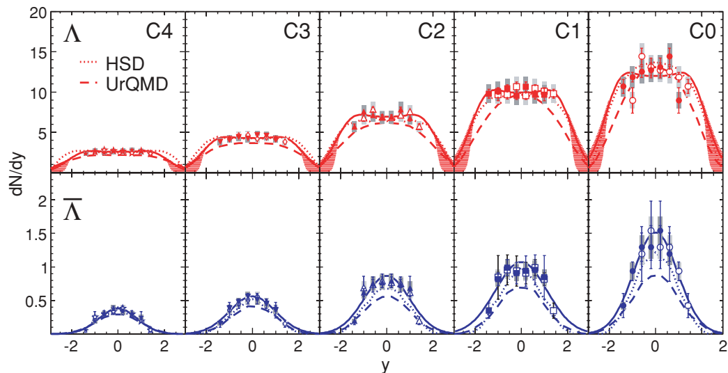
FIG. 8. (Color online) The rapidity spectra of \Lambda and \bar{\Lambda} for Pb + Pb collisions at 158A GeV in five different centrality bins C0–C4. The open symbols show data points reflected around midrapidity. The systematic errors are represented by the gray boxes. Solid lines are fits to the data points, used to extrapolate the measurements in order to extract total yields. The shaded areas in the \Lambda spectra sketches the uncertainty due to the different extrapolations. Also included are calculations with the HSD model [30–32] (dotted lines) and the UrQMD2.3 model [33–35] (dashed lines).
