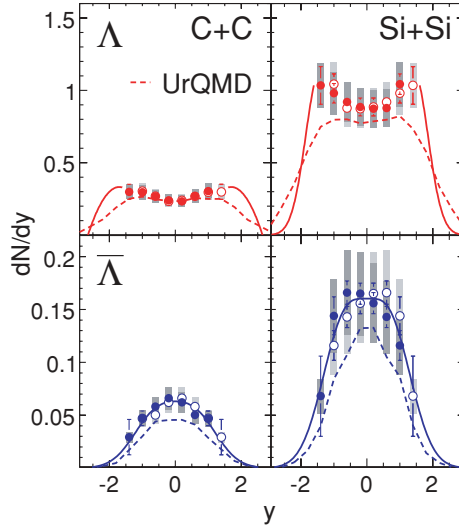
FIG. 9. (Color online) The rapidity spectra of \Lambda and \bar{\Lambda} for near-central C + C and Si + Si collisions at 158A GeV (the \Lambda spectra have already been published in Ref. [9]). Open symbols show data points reflected around midrapidity, while the systematic errors are represented by the gray boxes. Solid lines are fits to the data points, used to extrapolate the measurements to extract total yields. Also included are calculations with the UrQMD2.3 model [33–35] (dashed lines).
