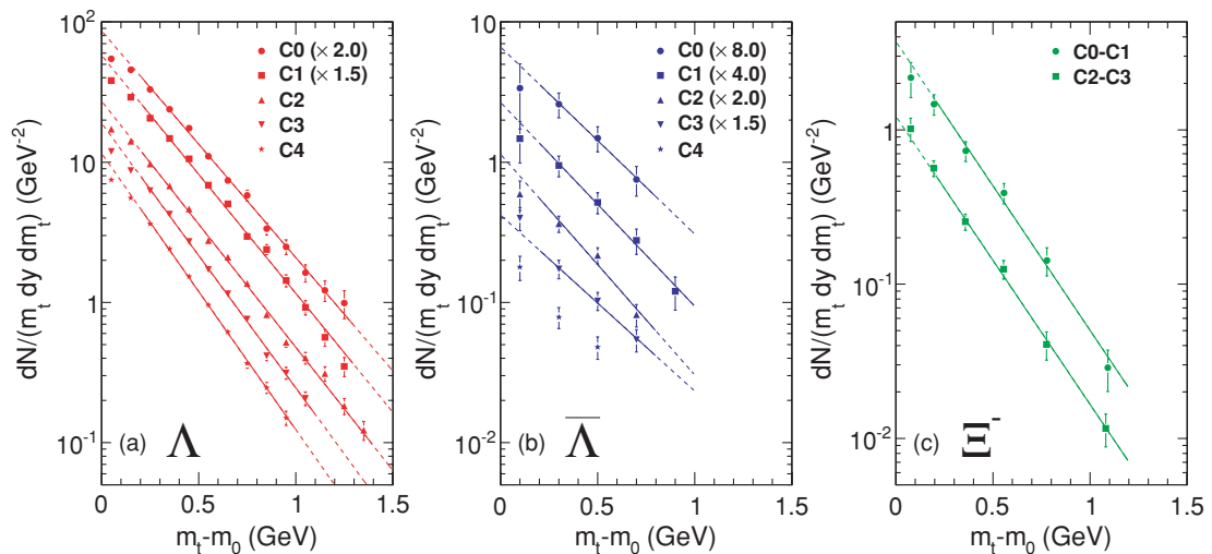
FIG. 4. (Color online) The transverse mass spectra of \Lambda (a), \bar{\Lambda} (b), and \Xi^- (c) at midrapidity ( \Lambda/\bar{\Lambda} : |y| < 0.4 , \Xi^- : |y| < 0.5 ) for Pb + Pb reactions at 40A GeV in different centrality bins. Some of the data points are scaled for clarity. Only statistical errors are shown. The solid/dashed lines represent fits with an exponential, where the solid parts denote the m_t ranges in which the fits were performed.
