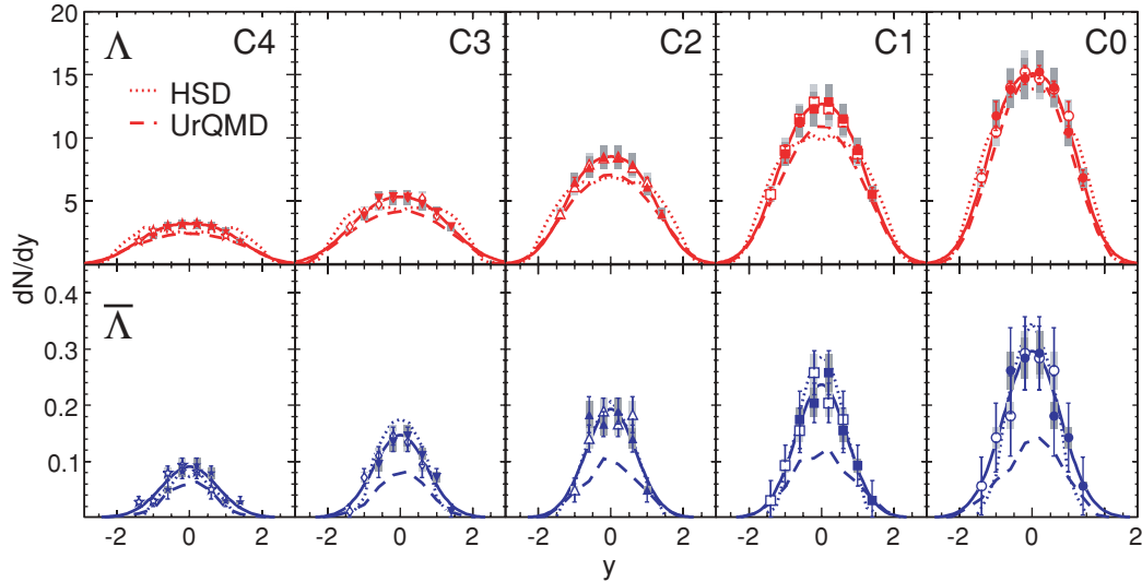
FIG. 7. (Color online) The rapidity spectra of \Lambda and \bar{\Lambda} for Pb + Pb collisions at 40A GeV for the five different centrality bins C0–C4. The open symbols show data points reflected around midrapidity. The systematic errors are represented by the gray boxes. Solid lines are fits to the data points, used to extrapolate the measurements to extract total yields. Also included are calculations with the HSD model [30–32] (dotted lines) and the UrQMD2.3 model [33–35] (dashed lines).
