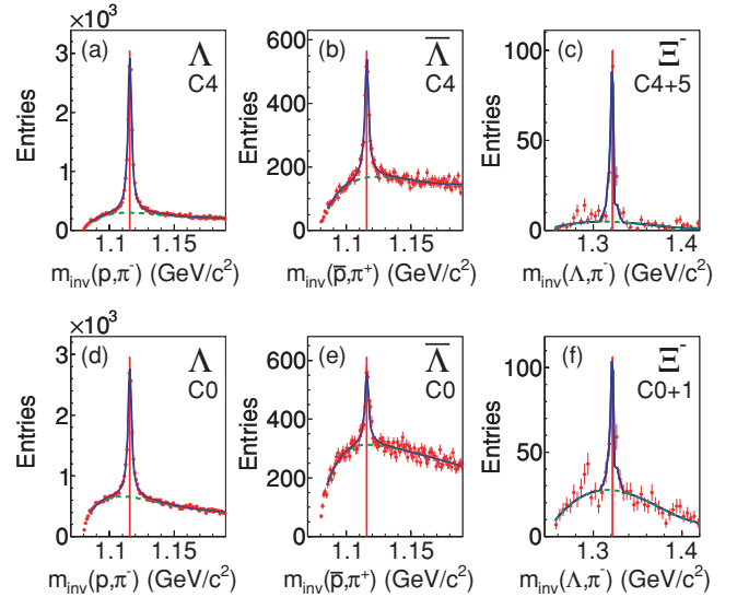
FIG. 1. (Color online) The invariant mass distributions of all measured \Lambda , \bar{\Lambda} , and \Xi^- candidates in two centrality classes of Pb + Pb collisions at 158A GeV. The upper row [(a)–(c)] shows the most peripheral centrality class and the lower row [(d)–(f)] the most central one. The full curves represent a fit to signal and background as described in the text, whereas the dashed curves show the background only. The vertical lines denote the literature values of the masses [21].
