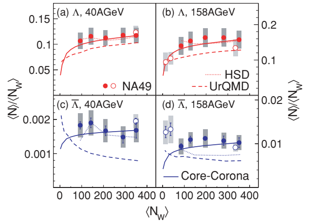
FIG. 12. (Color online) The total multiplicities \langle N \rangle divided by the average number of wounded nucleons \langle N_w \rangle of \Lambda and \bar{\Lambda} for Pb + Pb collisions at 40A and 158A GeV, as well as for near-central C + C and Si + Si reactions at 158A GeV, as a function of \langle N_w \rangle . The systematic errors are represented by the gray boxes. Filled symbols correspond to the minimum bias trigger, while the open ones represent online triggered (near-)central reaction systems. Also shown are calculations with the HSD model [30–32] (dotted lines), the UrQMD2.3 model [33–35] (dashed lines), and the core-corona approach (solid lines).
