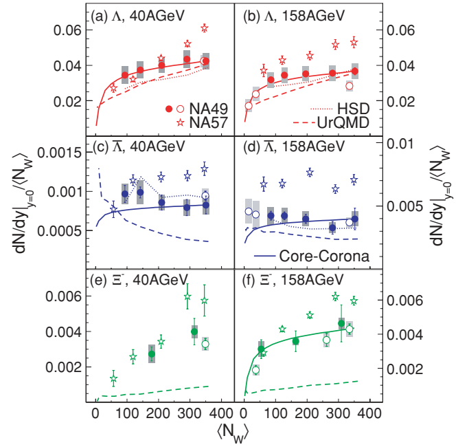
FIG. 11. (Color online) The rapidity densities dN/dy divided by the average number of wounded nucleons \langle N_w \rangle of \Lambda , \bar{\Lambda} , and \Xi^- at midrapidity ( \Lambda/\bar{\Lambda} : |y| < 0.4 , \Xi^- : |y| < 0.5 ) for Pb + Pb collisions at 40A and 158A GeV, as well as for near-central C + C and Si + Si reactions at 158A GeV, as a function of \langle N_w \rangle . The systematic errors are represented by the gray boxes. Filled symbols correspond to the minimum bias trigger, while the open ones represent the online triggered (near-)central reaction systems. Also shown are data of the NA57 Collaboration [5,36] (open stars) and calculations with the HSD model [30–32] (dotted lines), the UrQMD2.3 model [33–35] (dashed lines), and the core-corona approach (solid lines).
