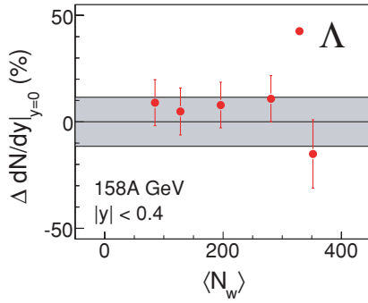
FIG. 3. (Color online) The differences between the fully corrected dN/dy values at midrapidity for \Lambda at 158A GeV as extracted with the standard procedure and the alternative analysis strategy (see Sec. II) for the different centrality bins. The gray area illustrates the systematic error estimate.
