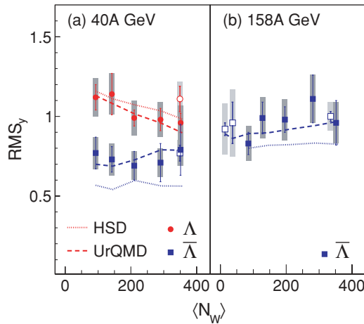
FIG. 10. (Color online) The RMS widths of the rapidity distributions RMS_y of \Lambda and \bar{\Lambda} at 40A and 158A GeV as a function of the number of wounded nucleons \langle N_w \rangle . The systematic errors are represented by the gray boxes. Filled symbols correspond to centrality selected data, obtained with a minimum bias trigger, while the open ones represent the reaction systems measured with a (near-)central trigger. Also included are calculations with the HSD model [30–32] (dotted lines) and the UrQMD2.3 model [33–35] (dashed lines).
