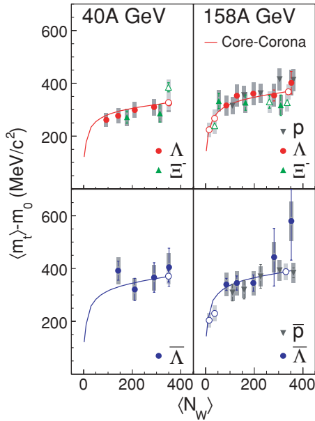
FIG. 6. (Color online) The \langle m_t \rangle - m_0 values at midrapidity ( p/\bar{p} : -0.5 < y < -0.1 , \Lambda/\bar{\Lambda} : |y| < 0.4 , \Xi^- : |y| < 0.5 ) for Pb + Pb collisions at 40A and 158A GeV, as well as for near-central C + C and Si + Si reactions at 158A GeV. The systematic errors are represented by the gray boxes. The filled symbols correspond to the results obtained from the minimum bias data sets, whereas the open ones represent the (near-)central reaction systems. The (anti-)proton data are taken from Ref. [27]. Also shown are the results from a fit for \Lambda and \bar{\Lambda} with the core-corona approach (solid lines).
