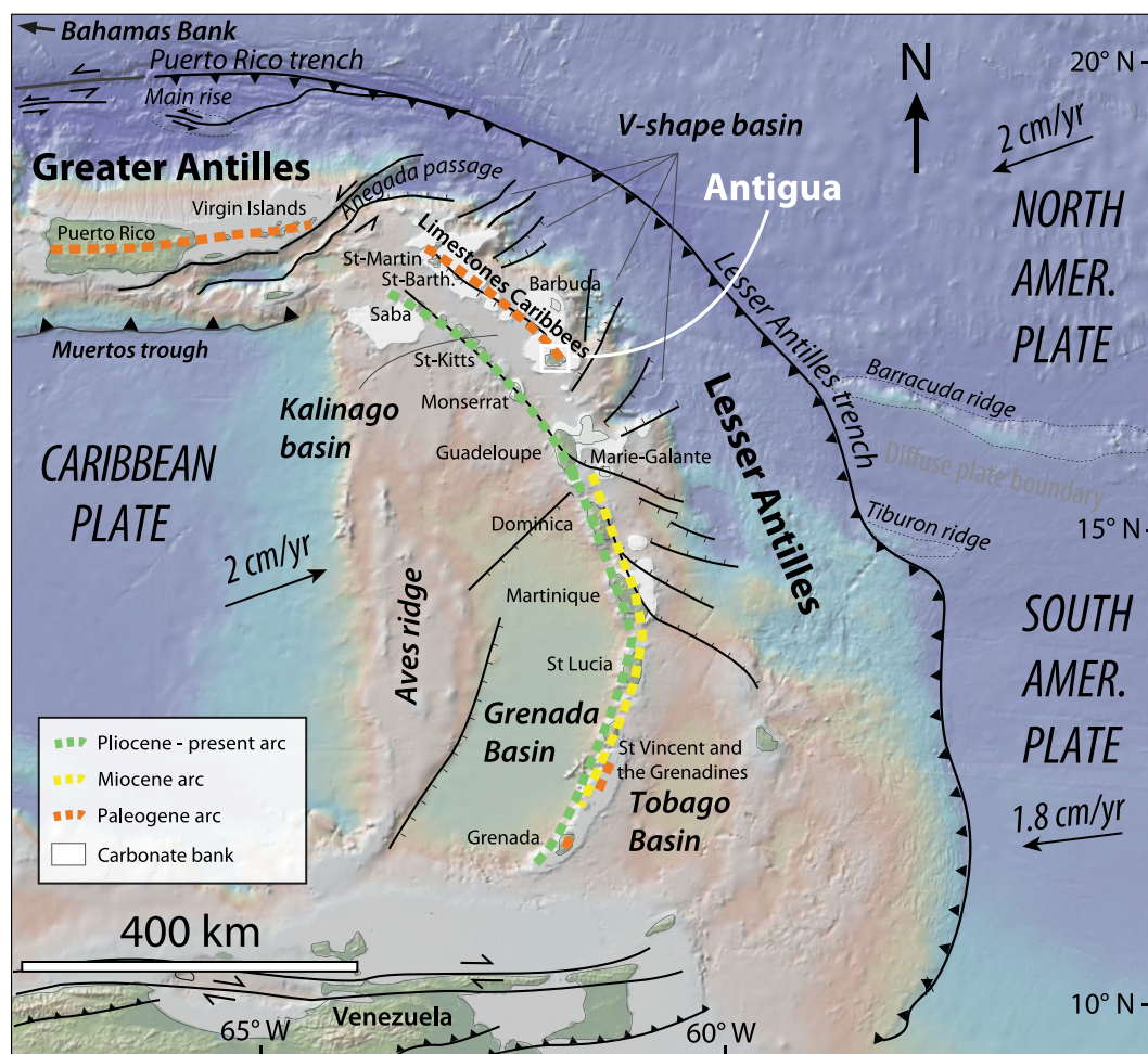
Figure 1. Bathymetric map shows tectonic and volcanic settings of the Lesser Antilles subduction zone. The main faults are drawn from Cornée et al. (2021). The study area (Antigua) is outlined by the white square. Velocity vectors of the Caribbean and North and South American plates are from Symithe et al. (2015).
