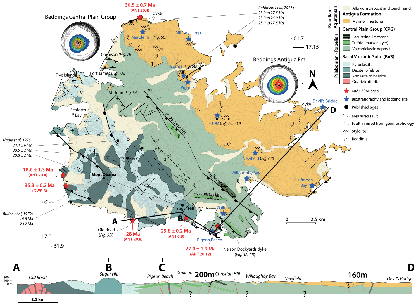
Figure 3. Revised geological map and synthetic cross-section of Antigua are shown. The map was constructed based on the maps of Martin-Kaye (1959, 1969) and Christman (1973) and completed and updated with fieldwork observations, lithostratigraphy, and structural measurements. The cross-section is located by a gray line crosscutting the island from NE to SW, with tipping point marked by the letters A, B, C, and D. The tuffite layer (light green) was used as a marker layer in the construction of the cross-section. Beddings are plotted on the lower hemisphere. The K-Ar ages (Nagle et al., 1976; Briden et al., 1979) and the Sr-Sr ages (Robinson et al., 2017) are represented in italic.
