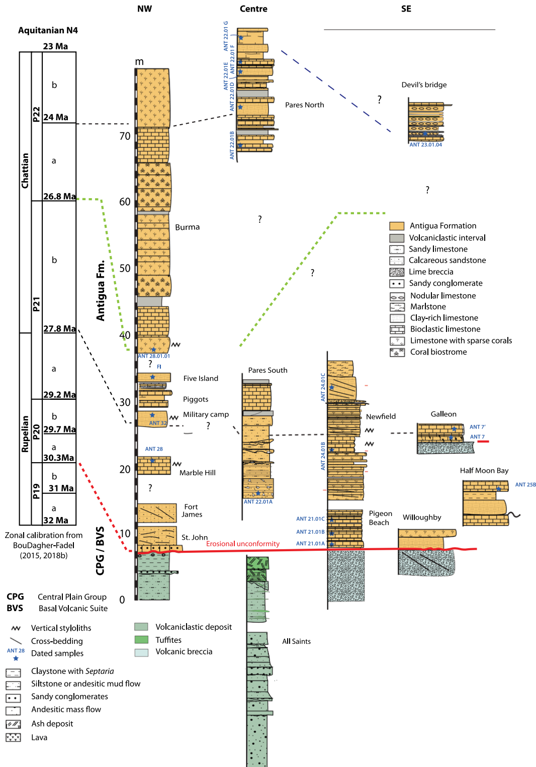
Figure 4. Stratigraphic synthesis and lithological successions of the Antigua units are shown. The locations of the sections are presented in Figure 3. See Supplemental Material 1 for a detailed description of each section (see text footnote 1). CPG/BVS—Central Plain Group/Basal Volcanic Suite.
