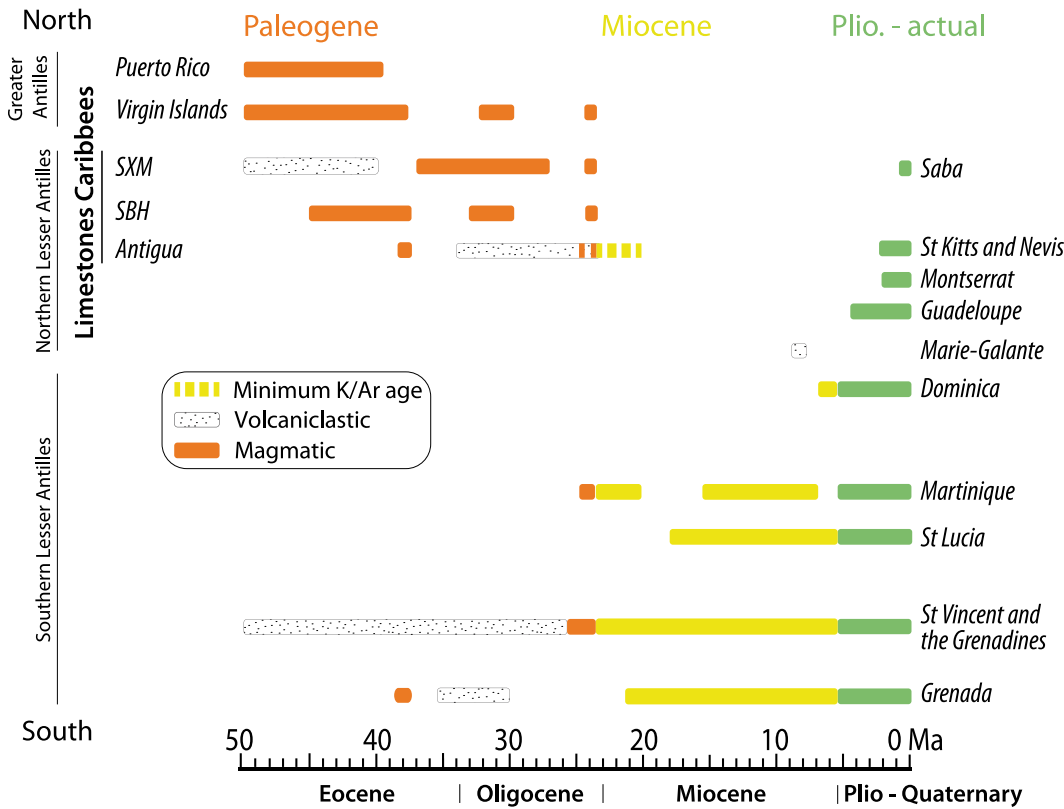
Figure 2. Schematic representation shows the dated magmatic and volcanoclastic onshore evidence of the Lesser Antilles arc, from Eocene to present. The references used to construct this sketch are noted in Table 1. SXM—Saint-Martin; SBH—St-Barthelemy.
