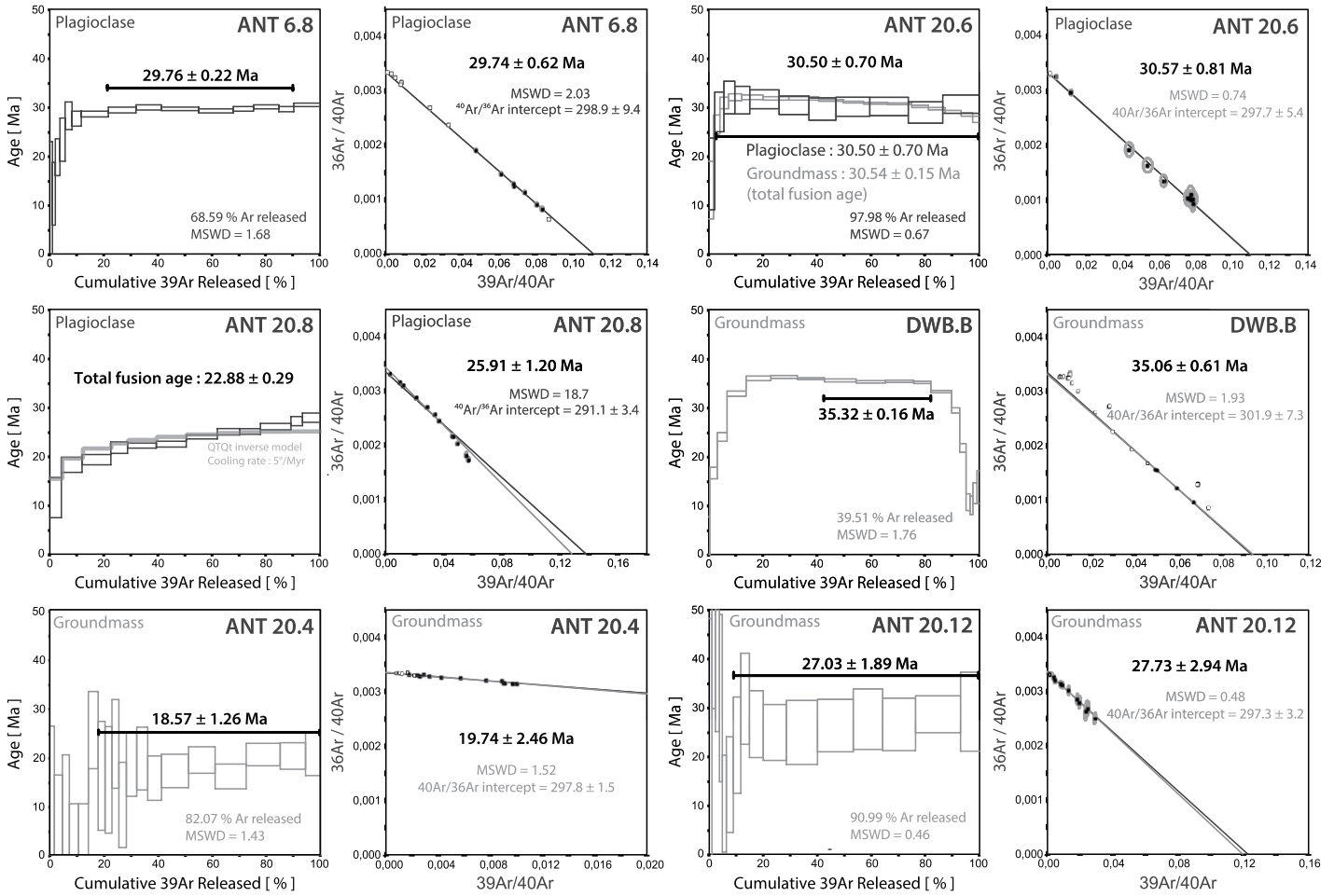
Figure 6. ^{40}\text{Ar}/^{39}\text{Ar} spectra and inverse isochrons are shown for the samples from Antigua. MSWD—mean square weighted deviation. The thick gray line in the spectra of ANT 20.8 corresponds to the spectrum modeled using QTQt software (Gallagher, 2012).
