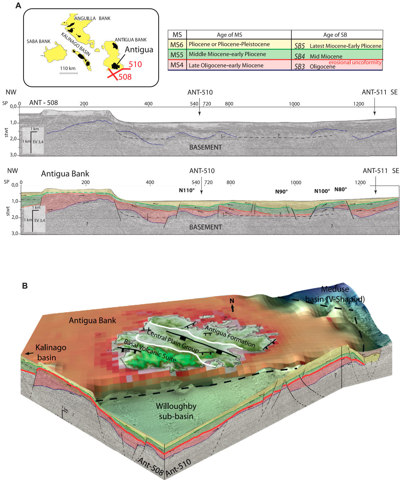
Figure 11. (A) Time-calibrated seismic stratigraphic analysis of the seismic profiles CPEM 508 and 510 (in red; ARCANTE 3 Cruise, Bouysse et al., 1985; Bouysse and Mascle, 1994) from Cornée et al., 2021. Top: uninterpreted; below: interpreted. The definition and time calibration follow the seismic stratigraphic chart defined by Cornée al. (2021) in the northeastern Lesser Antilles. MS—megasequence; SB—sequence boundary. (B) Three-dimensional block with seismic profiles 508 and 510 shows the onshore and offshore structures in Antigua, Willoughby basin, and the V-shaped Méduse basin. Note the erosional character of the SB4 unconformity that seals prior faults affecting MS4.
