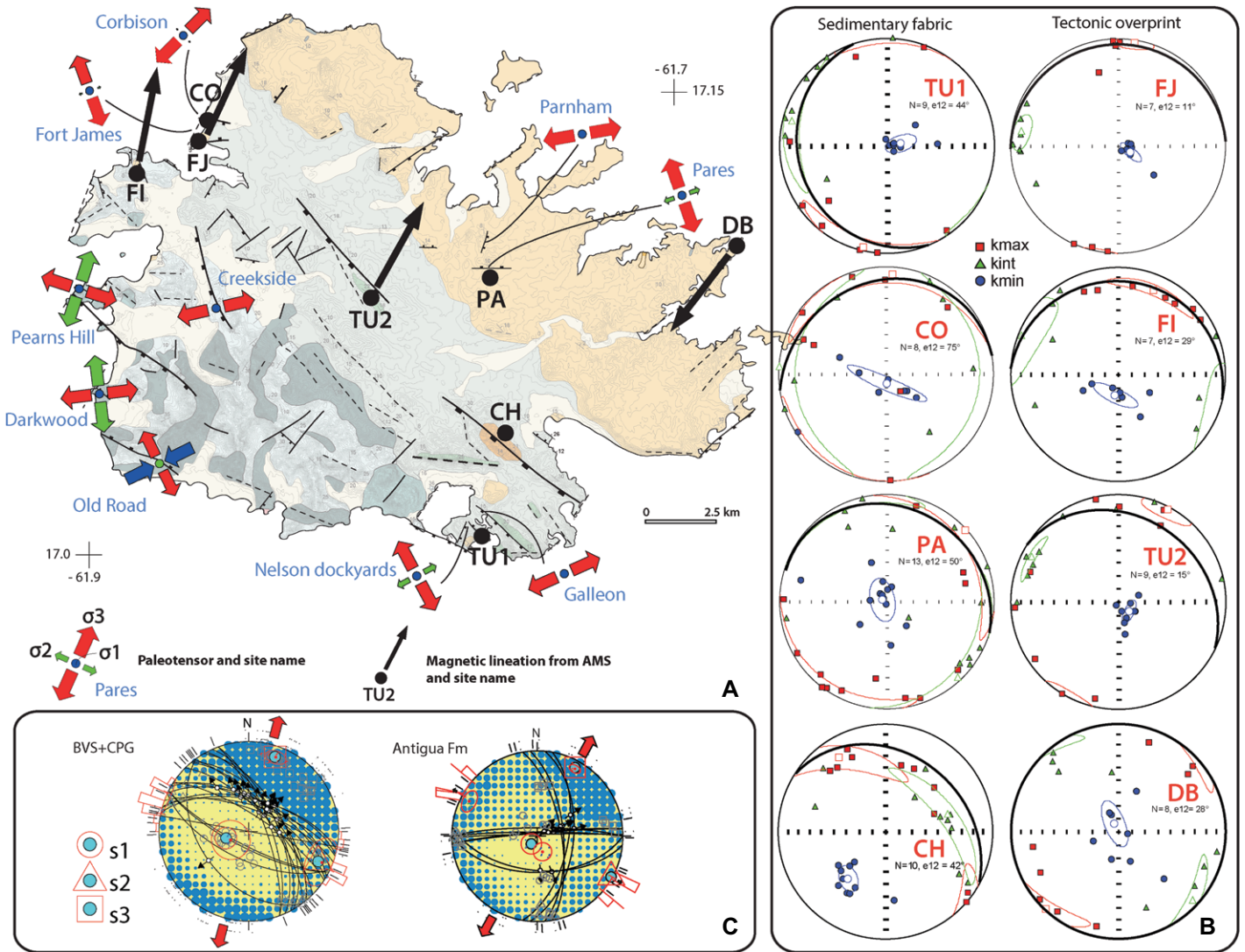
Figure 10. (A) Kinematic map shows Antigua with paleotensors (colored arrows) estimated per fault and magnetic lineation (black arrows) estimated from anisotropy of magnetic susceptibility (AMS) analysis. (B) Schmidt equal area projections of the AMS ellipsoid principal axis for all sampled sites in geographic coordinates; 95% confidence ellipses and associated mean values for each axis are represented by colored lines and empty symbols, respectively. Bold black arc represents the mean bedding plane of the site. (C) Paleostress tensor obtained from the field data (faults with kinematic criteria and fractures) for the NW-SE-trending faults within the Basal Volcanic Suite (BVS) and the Central Plain Group (CPG; to the left) and for the E-W- and N-S-trending faults of the Antigua Formation (to the right).
