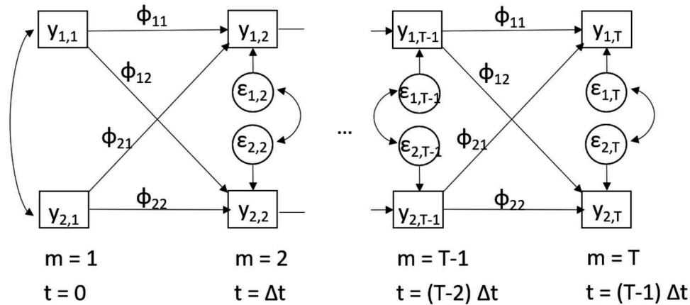
FIGURE 1 Bivariate relationship between y_1 (e.g., child health) and y_2 (e.g., maternal health) for time points t = 0, \dots, (T - 1)\Delta t with autoregression parameters \phi_{11} and \phi_{22} , and cross-lagged parameters \phi_{12} and \phi_{21} . In case of a symmetric relationship, the cross-lagged/reciprocal parameters are equal, that is, \phi_{12} = \phi_{21} .
