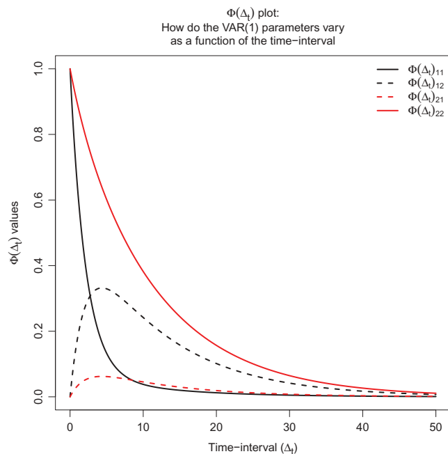
FIGURE 2 \Phi(\Delta t) plot: A bivariate example of how the parameter values (i.e., the elements in \Phi(\Delta t) ) change as a function of the time-interval \Delta t .
