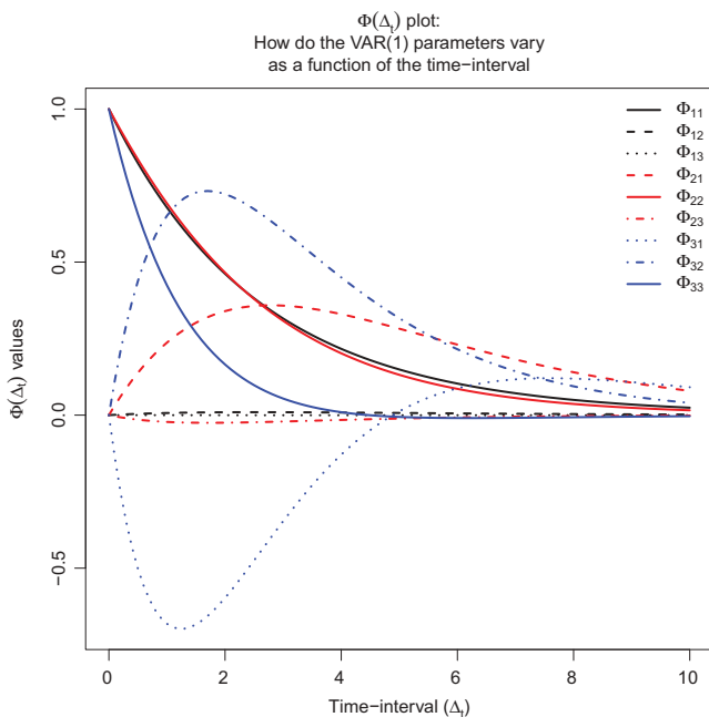
FIGURE 5 The \Phi(\Delta t) plot for a trivariate \Phi(\Delta t) , with change in dominance and sign, that is, where conclusions I to III may differ per time-interval \Delta t .
