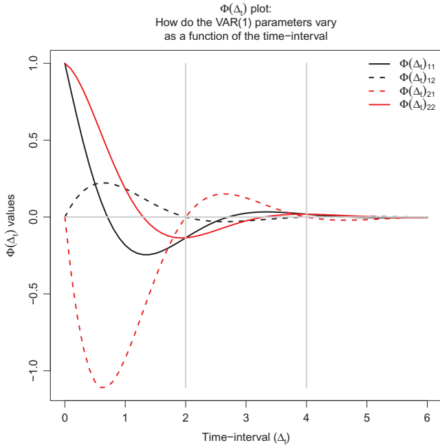
FIGURE 3 The \Phi(\Delta t) plot for a bivariate \Phi(\Delta t) with complex eigenvalues, where conclusions I to III may differ per time-interval \Delta t .
