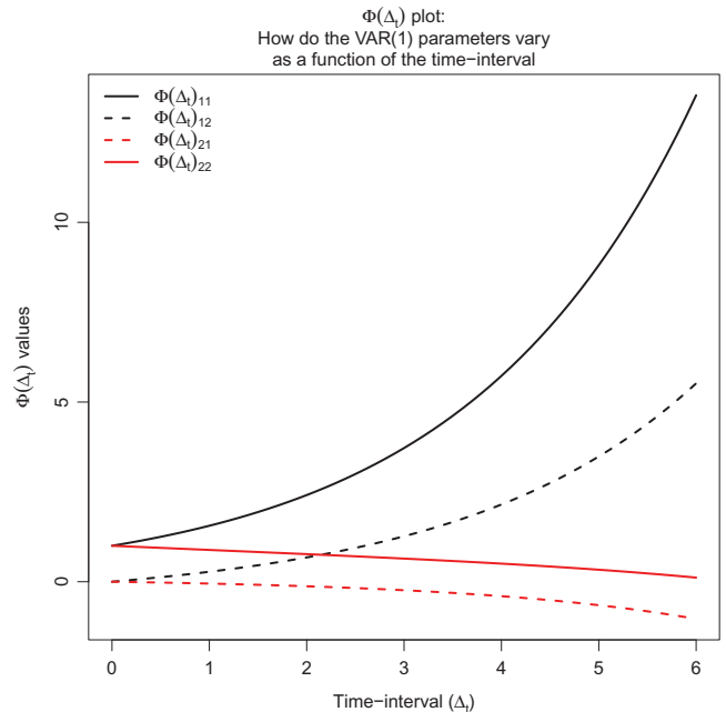
FIGURE 4 The \Phi(\Delta t) plot for an unstable, bivariate \Phi(\Delta t) with one negative and one positive real eigenvalue, where conclusions I to III may differ per time-interval \Delta t .
