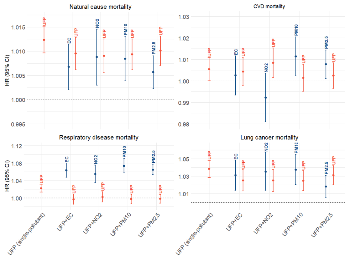
Fig. 2. Two-pollutant models of UFP adjusted for NO 2 , PM 2.5 , PM 10 and EC with natural and cause-specific mortality a,b .
