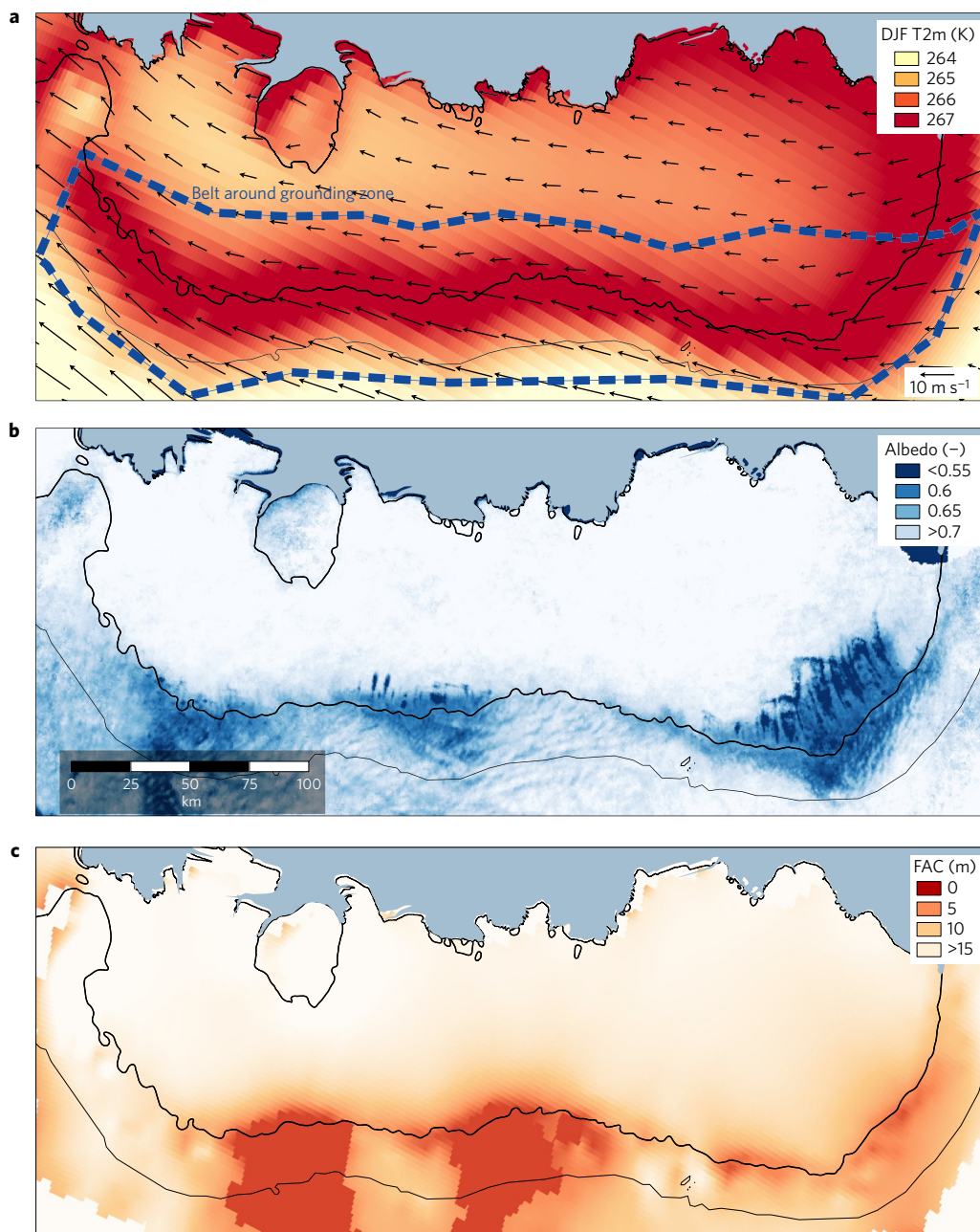
Figure 2 | Summer near-surface climate and surface conditions of the RBIS. a , Simulated 1979–2015 mean summer (December, January, February (DJF)) near-surface temperature (colours) and near-surface wind speed (vectors). b , Summer albedo (lowest 5% percentile value) derived by MODIS imagery. c , Mean FAC for the period 1979–2015. FAC equals the total air content of the firn layer (that is, the vertically integrated difference between the ice density and the actual density), and is expressed as the thickness of the equivalent air column contained in the firn in metres. The extent of the grounding zone for which the surface melt was calculated (Supplementary Fig. 5) is drawn with the dashed blue line in a .
