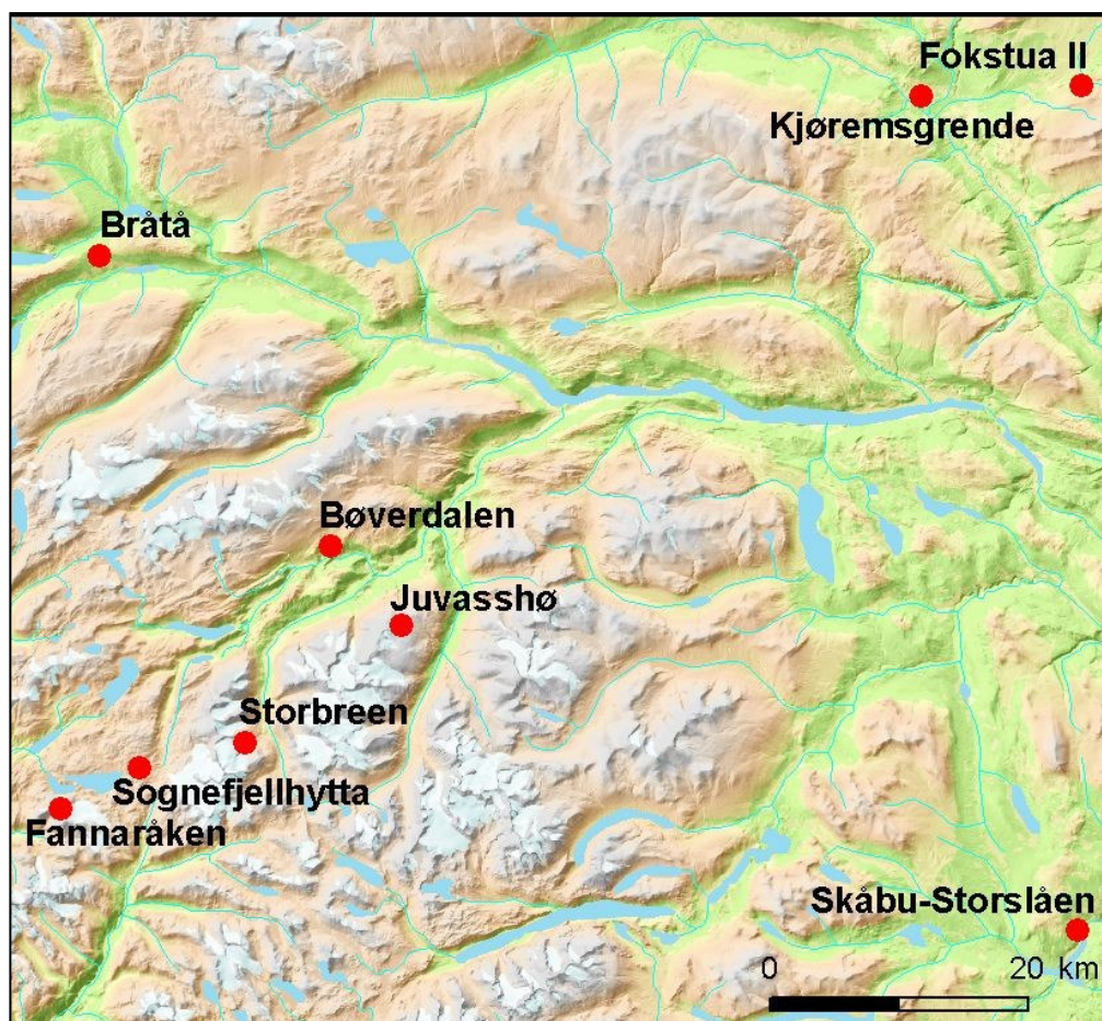
Figure 2-7. Meteorological stations used as input data or for calibration for the mass balance model of Storbreen.
