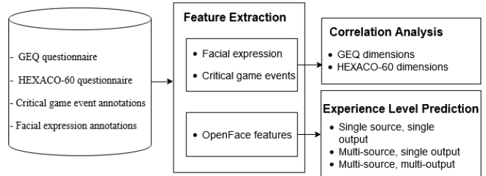
Figure 4. Methodology Pipeline.
