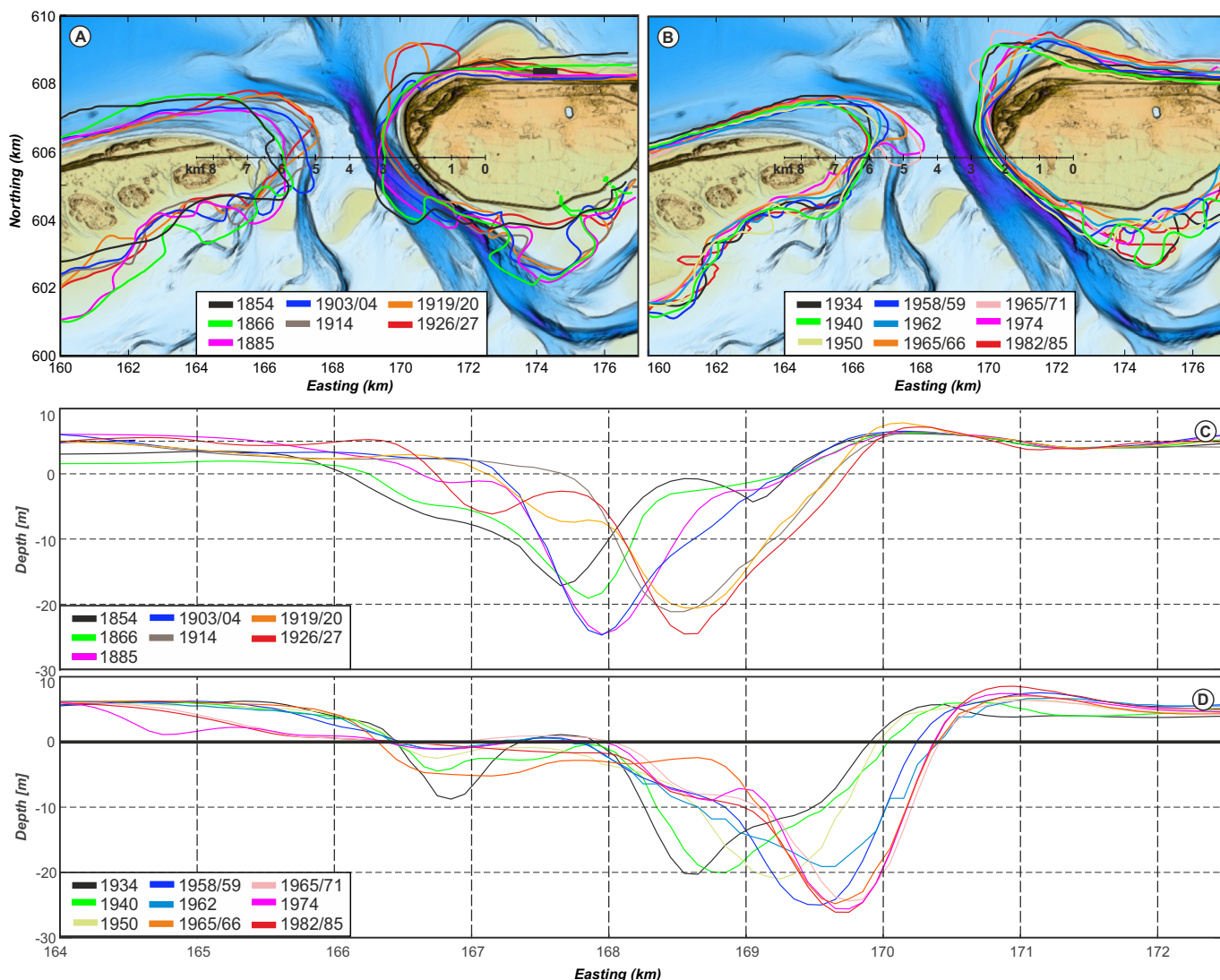
Fig. 12. Coastline position of the islands Terschelling and Ameland based on digitized charts over the time-frame (A) 1854–1926/27 and (B) 1934–1982/1985. (C–D) Cross-sections illustrating the depths of the inlet gorge; scale bar in figs. A and B provides the location of the transect.
