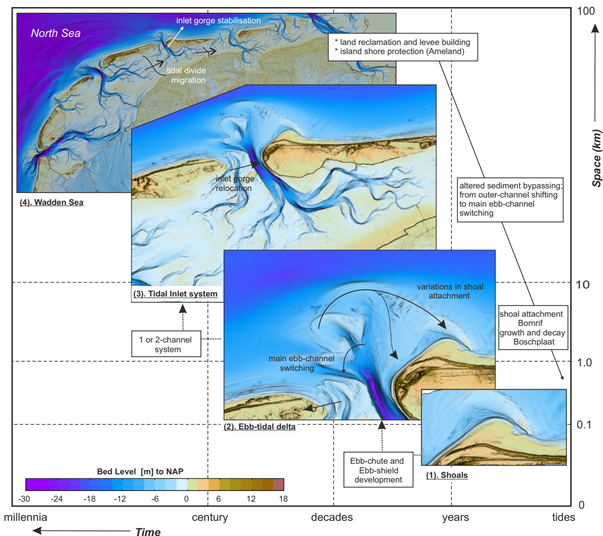
Fig. 13. A cascade of scales and relevant processes to describing the change in inlet dynamics over various scales for Ameland Inlet.
