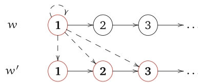
FIGURE 1 Haecceitistic differences between w and w' assuming P5
