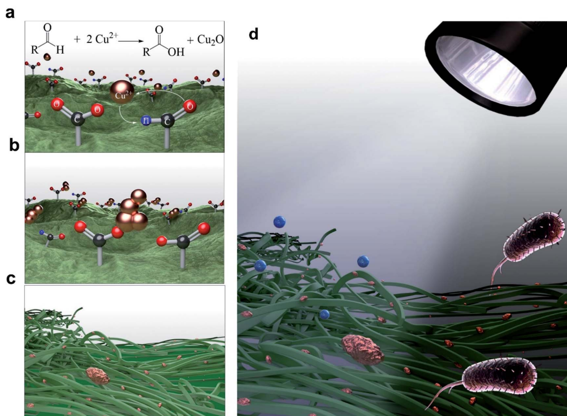
Fig. 6 Mineralization of copper oxide nanoparticles on TOCNF films. (a) Reduction of \text{Cu}^{2+} ions to \text{Cu}^+ by the aldehyde groups on TOCNF. (b) Growth of copper oxide nanoclusters. (c) Coalescence of nanoclusters to form \text{Cu}_2\text{O} nanoparticles. (d) Schematic representation showing the antibacterial/photocatalytic activity of the resultant hybrid membrane. 49
