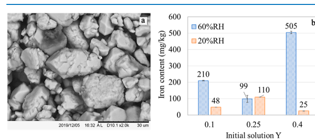
Figure 6. (a) SEM picture of the precipitated crystals while the solution was continuously stirred during evaporation and (b) iron content of NaCl crystals formed at 60 rpm stir rate for two evaporation conditions.
