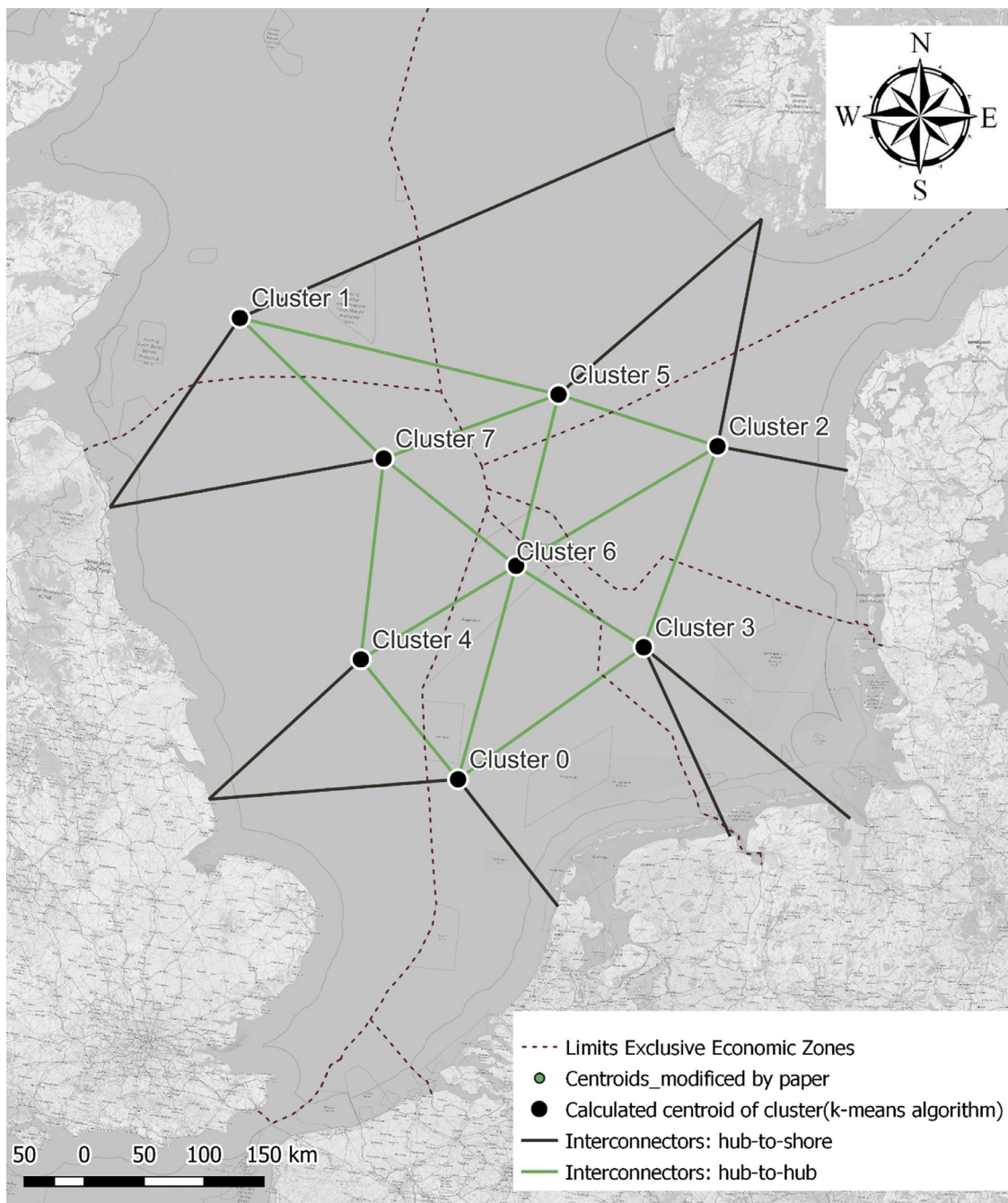
Fig. 11. NSOG interconnectors allowed, divided in hub-to-hub interconnectors (green) and hub-to-shore interconnectors (black). (For interpretation of the references to colour in this figure legend, the reader is referred to the web version of this article.)
