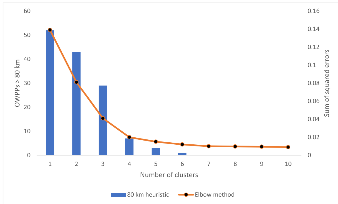
Fig. 6. Elbow method and 80 km heuristic results.
