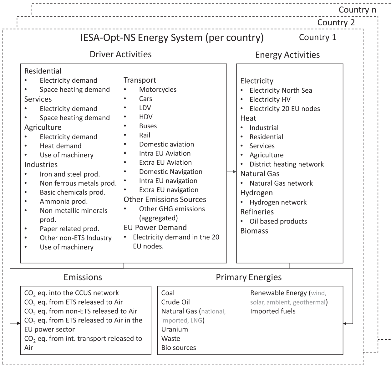
Fig. 26. Energy system representation of activities considered within the IESA-NS framework.
