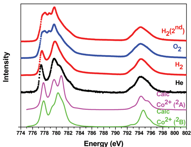
Figure 3. Co L_{2,3} -edge XAS, from bottom to top, a multiplet calculation of \text{Co}^{2+} with 10Dq = 2.3 , Dt = 0.2 , and Ds = 0.7 eV (green, {}^2B ), a multiplet calculation of \text{Co}^{2+} with 10Dq = 2.3 , Dt = 0.2 , and Ds = 0.5 eV (pink {}^2A ), experimental spectra of CoPc pellet in helium (He, black), hydrogen ( \text{H}_2 , red), oxygen ( \text{O}_2 , blue) and for the second time in hydrogen ( \text{H}_2(2\text{nd}) , red) environment with gas pressures of 0.5 mbar.
