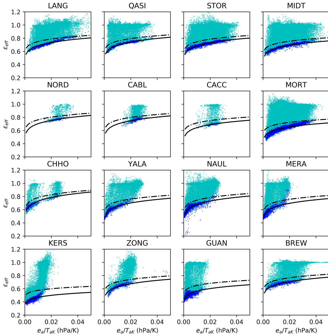
Figure A3. Observed \varepsilon_{\text{eff}} (points) and calculated \varepsilon_{\text{cs}} (solid line) fitted to lowest 10% of LWIn in 30e_a/T_{a,K} bins (shown in blue). Calculated \varepsilon_{\text{eff}} at clear-sky limit of N_{\varepsilon} = 0.2 (dash-dotted line).
