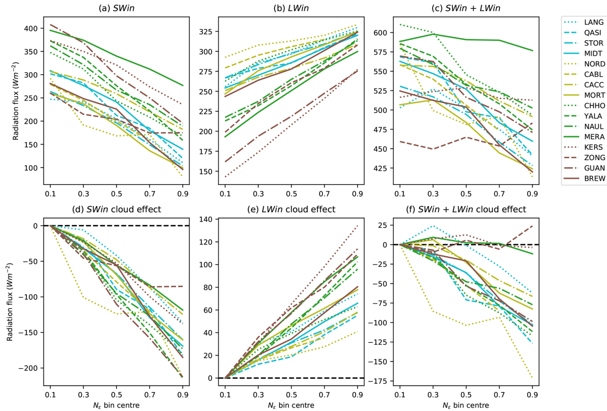
Figure 6. (a–c) Average melt-season incoming radiation fluxes (SWin, LWin) for different daily average cloud conditions ( N_\epsilon ). (d–f) As for (a–c) expressed as change from clear-sky conditions ( N_\epsilon \leq 0.2 ). Note that the y-axis range differs between panels.
