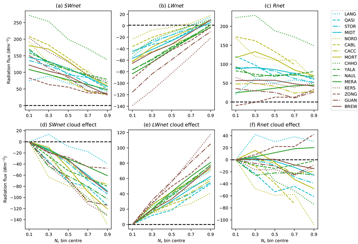
Figure 7. (a–c) Average melt-season net radiation fluxes (SWnet, LWnet, Rnet) for different daily average cloud conditions ( N_{\varepsilon} ). (d–f) As for (a–c) expressed as change from clear-sky conditions ( N_{\varepsilon} \leq 0.2 ). Note that the y-axis range differs between panels.
