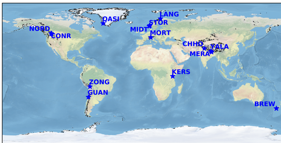
Figure 1. Map showing the location of study sites with short names (see Table 1 for full names) along with glacier areas from the Randolph Glacier Inventory (black outlines; RGI Consortium, 2017). Note that the two Conrad Glacier sites (CABL, CACC) are shown as CONR and the two Mera Glacier sites (MERA, NAUL) are shown as MERA. The background map is Natural Earth shaded relief.
