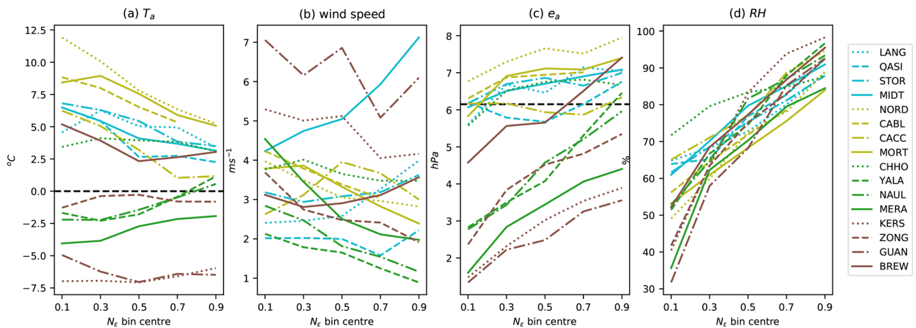
Figure 8. Average melt-season near-surface meteorology for different daily average cloud conditions ( N_{\varepsilon} ). Dashed lines indicate melting point temperature in (a) and saturation vapour pressure in (c).
