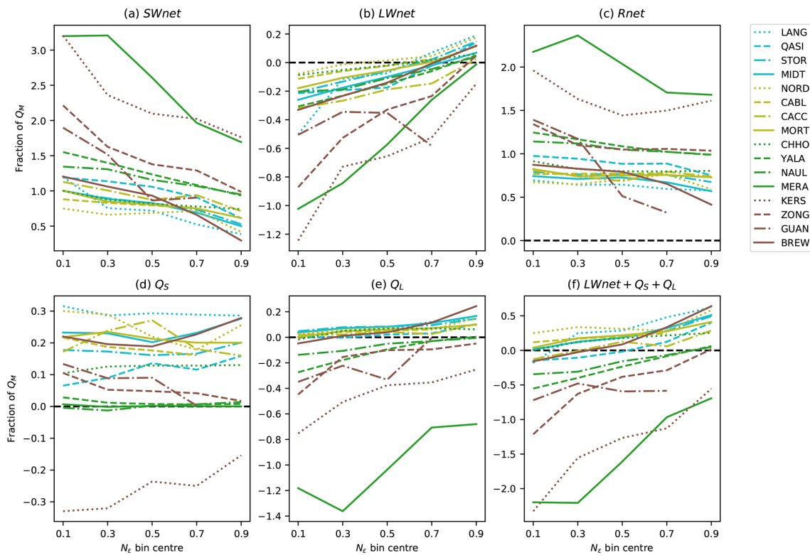
Figure 11. Average melt-season SEB terms during hours with surface melt for different cloud conditions ( N_\epsilon ). Variables are shown as a fraction of average Q_M during hours with surface melt in each respective cloud condition ( N_\epsilon ). Note that the y-axis range differs between panels.
