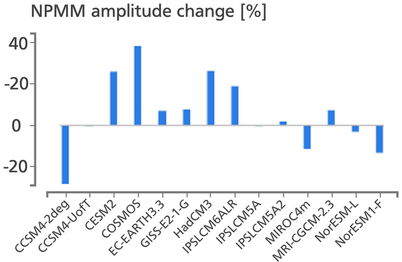
Extended Data Fig. 7 | North Pacific Meridional Mode amplitude change. Simulated change in the amplitude of the North Pacific Meridional Mode.
