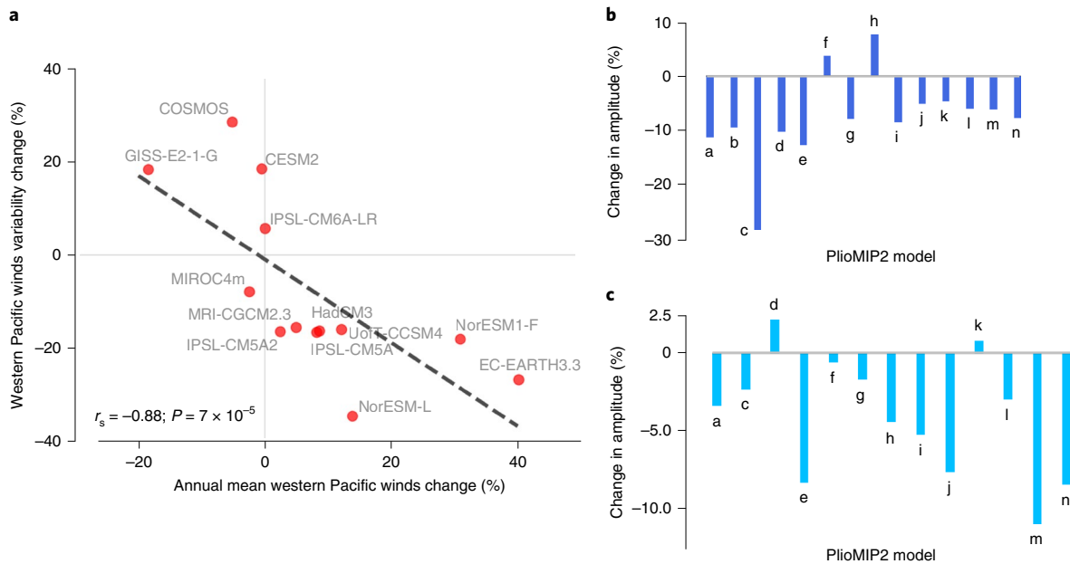
Fig. 4 | Changes to potential ENSO triggers. a , Intermodel relationship between the change in the intensity of the western Pacific trade winds ( 10^{\circ} S– 10^{\circ} N; 160^{\circ} E– 150^{\circ} W) and the amplitude (standard deviation) of its monthly variability. To ideally examine changes in the western wind bursts, we would need high-frequency output, which is not available for the PlioMIP models. b , Change in the amplitude (standard deviation) of the SPMM time series, defined as the mean SST anomaly between 15^{\circ} S and 25^{\circ} S and between 110^{\circ} W and 120^{\circ} E. c , Change in the amplitude (standard deviation) of the meridional wind variability over the SHB region ( 10^{\circ} S– 30^{\circ} S; 140^{\circ} E– 170^{\circ} E). PlioMIP2 models in b and c : a , CCSM4-UofT; b , CCSM4-2deg; c , CESM2; d , COSMOS; e , EC-EARTH3.3; f , GISS-E2-1-G; g , HadCM3; h , IPSL-CM6A-LR; i , IPSL-CM5A; j , IPSL-CM5A2; k , MIROC4m; l , MRI-CGCM2.3; m , NorESM-L; n , NorESM1-F.
