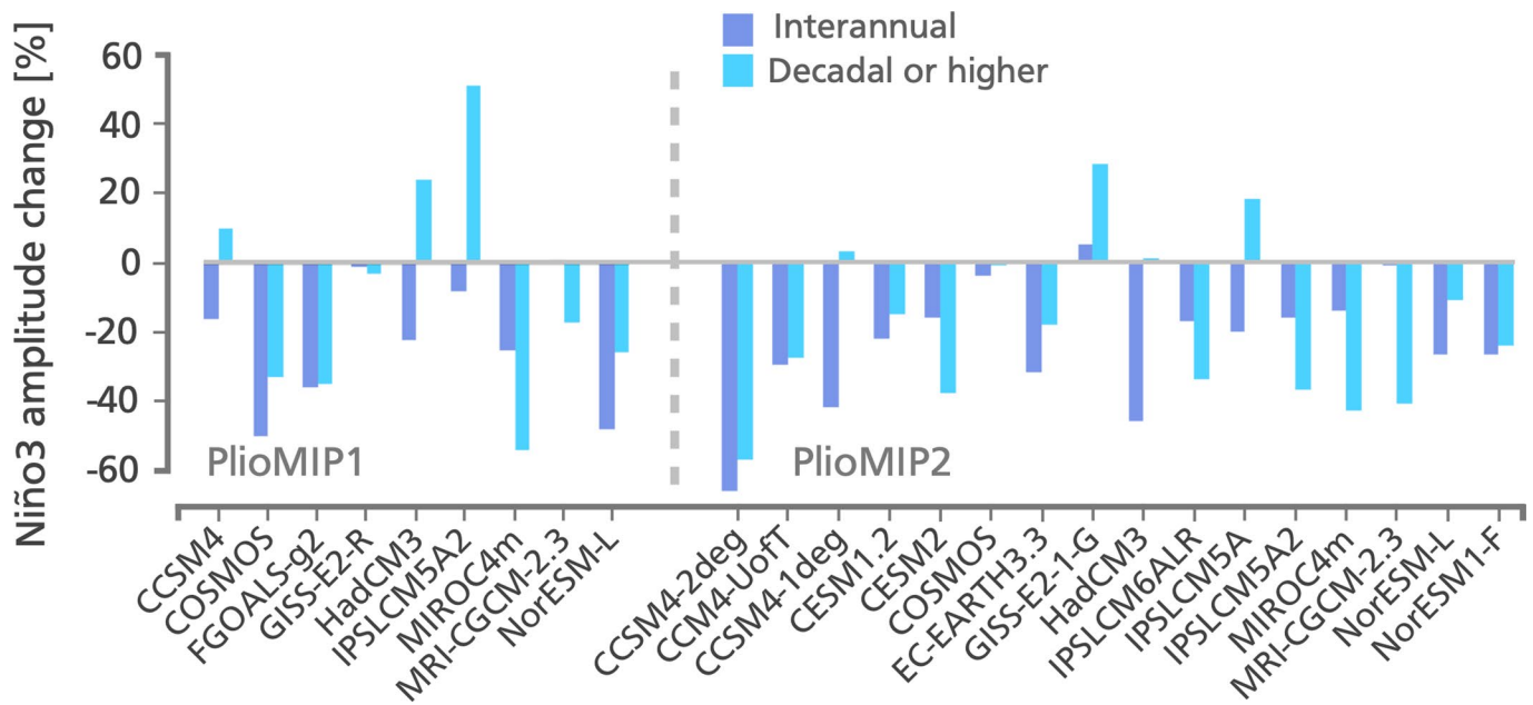
Extended Data Fig. 2 | Mid-Pliocene changes in eastern Pacific SST variability by frequency bands. Percentage change in Niño3 (5°N-5°S; 150°-90°W) standard deviation separated by interannual (dark blue) and low-frequency (>10 yr; light blue) variability. The amplitude of low-frequency oscillations is evaluated through the variance of the 11-year running mean Niño3 time series in each model. The amplitude of the interannual period is estimated as the variance of the residual time series, that is, original Niño3 timeseries subtracted from the Niño3 decadal timeseries.
