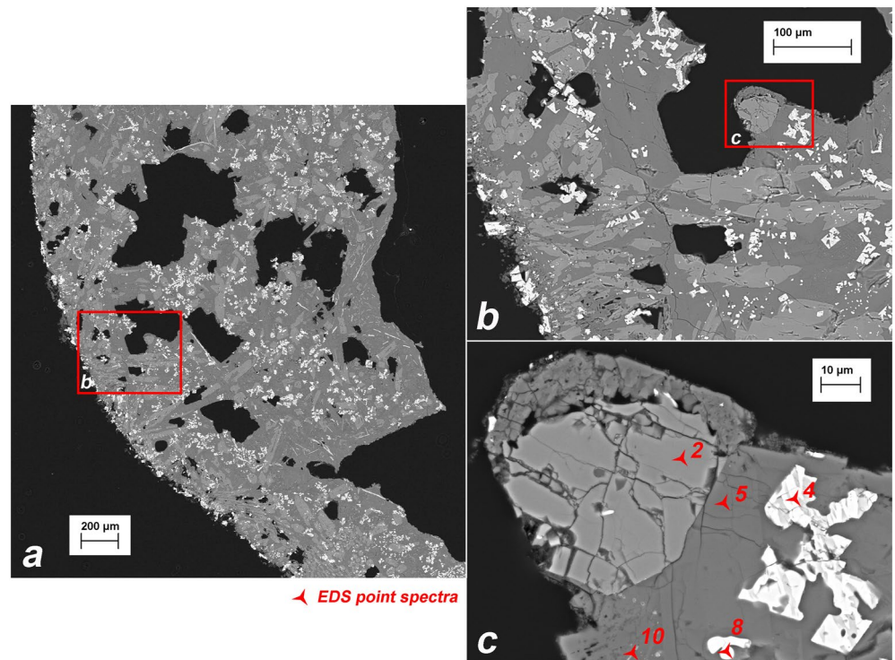
Figure 7. Igneous mineralogy. (a–c) Backscattered electron (BSE) images of sample H7 thin section, showing clear, angular grains indicating largely unaltered basalt. (c) Energy-dispersive X-ray spectroscopy (EDS) point spectra taken of spots marked in red, revealing typical basaltic mineralogy: augitic clinopyroxene (2), dendritic titanomagnetite, (oxy-) exsolved into a fine intergrowth of Ti-poor magnetite (white) and ilmenite (slightly less bright) (4), plagioclase (5), magnetite (8), and apatite growth, indicating a highly evolved interstitial melt pocket (10). The spectra can be seen in Supporting Information S1.
