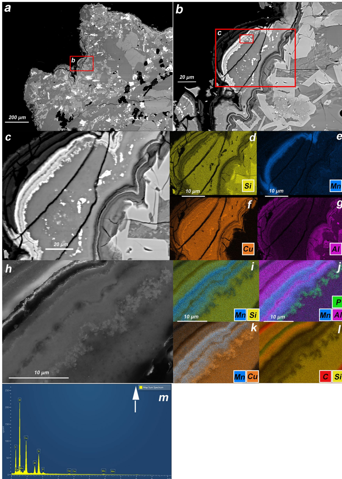
Figure 9. Complex secondary mineral precipitate. (a–c) backscattered electron (BSE) image of a secondary mineral crust deposited on the edge of the igneous rock in sample B5 thin section. (d–g) Elemental maps of silicon, manganese, copper, and aluminum. (h) BSE image of close-up of secondary mineral crust. (i–l) Composite elemental maps of manganese and silicon (i), phosphorus, manganese, and aluminum (j), manganese and copper (k), and carbon and silicon (l). (m) energy-dispersive X-ray spectroscopy (EDS) sum spectrum of (h) showing copper, phosphorus, and manganese enrichment. The EDS sum spectrum of (c) can be seen in Supporting Information S1.
