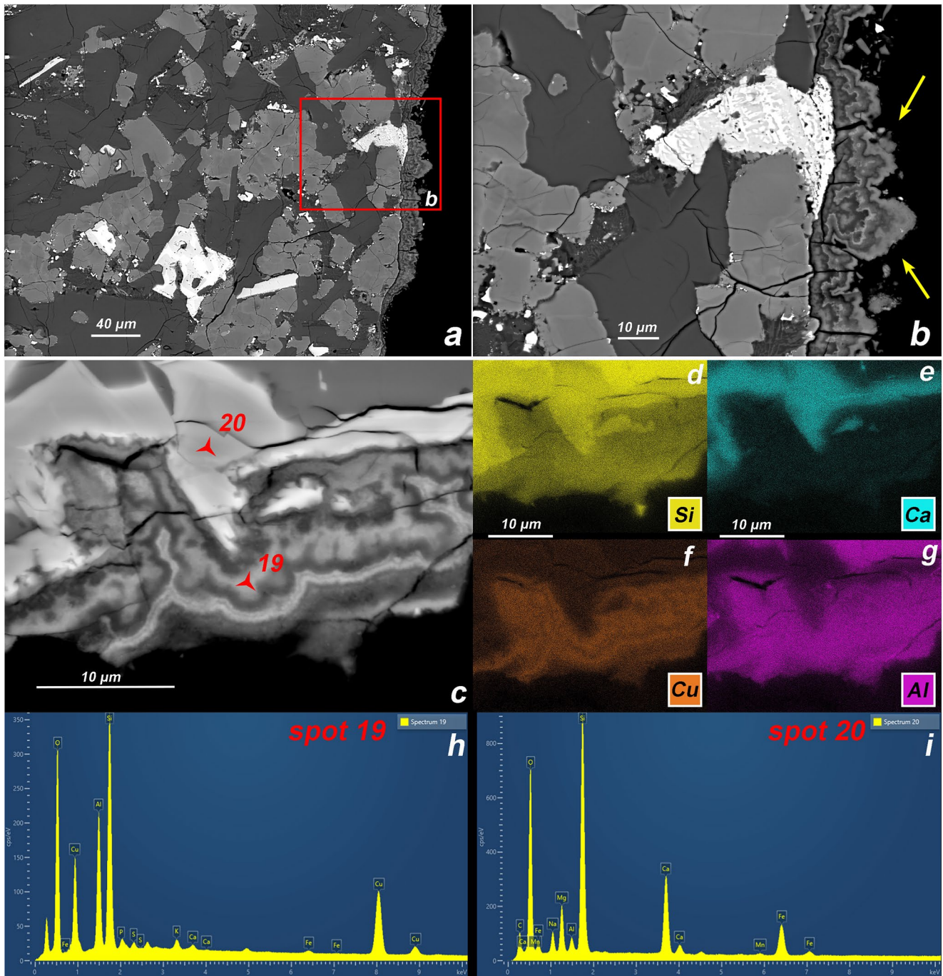
Figure 8. Botryoidal secondary mineral precipitate. (a) Backscattered electron (BSE) image of a botryoidal, layered secondary mineral crust deposited on the edge of the igneous rock in sample C2. (b) Zoom-in on botryoidal crust, indicated by the yellow arrows. (c) BSE image of the botryoidal mineral crust in another location in C2. (d–g) Elemental maps of silicon, calcium, copper, and aluminum present in the section presented in (c). (h) Energy-dispersive X-ray spectroscopy (EDS) spectrum of spot 19 (secondary mineral, pane c), showing copper and aluminum enrichment, possibly indicative of chrysocolla. (i) EDS spectrum of spot 20 (lava rock, pane c), showing unaltered augitic pyroxene.
