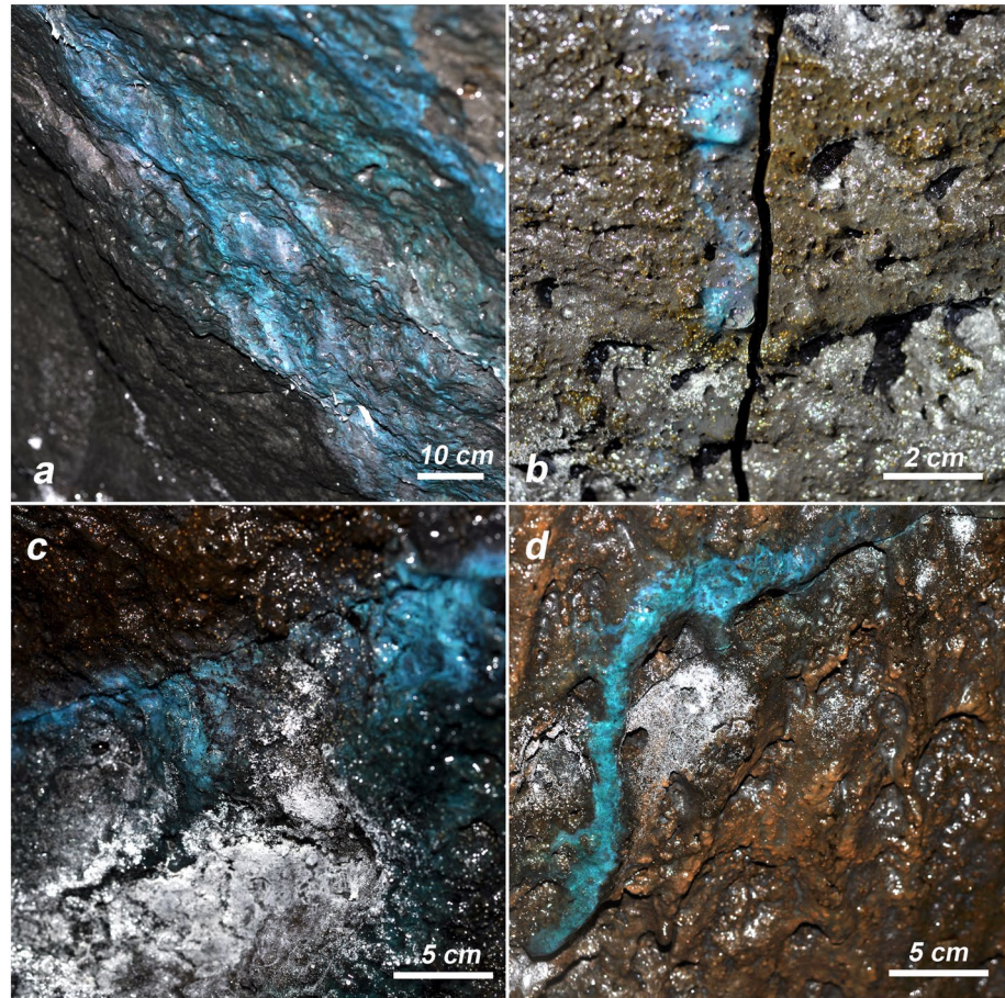
Figure 2. Examples of blue features. Blue mats and mineral precipitates are often found on surfaces of flowing water (a), or along cracks in cave walls or ceiling, where water seeps in from the ground above (b–d).
