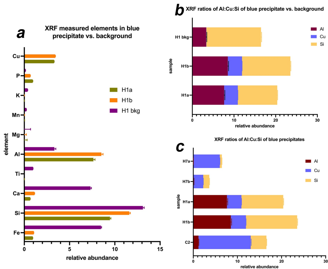
Figure 5. X-ray fluorescence (XRF) measurements of blue precipitates in sample H1 versus background. (a) Major elements were measured by pointing the XRF onto the cave wall where the mat was collected, versus the background, that is, a spot on the wall nearby not covered in mat. (b) Ratios of select elements aluminum, copper, and silicon in blue precipitate versus background. Copper is markedly absent in the background. (c) Al:Cu:Si ratios measured in all blue precipitates.
