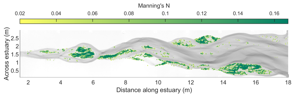
Figure 7. Example of Manning roughness values for the vegetated estuary specified as initial condition in the Nays2D flow model at 13 000 tidal cycles. The Manning roughness of the unvegetated bed is set to 0.02 in the model.
