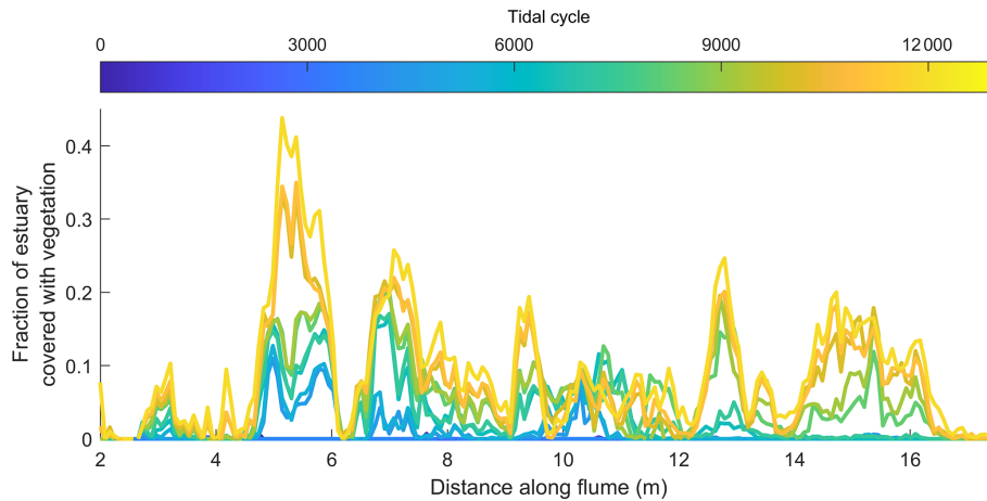
Figure 12. Development of vegetation cover as a fraction of estuary width along the estuary.
