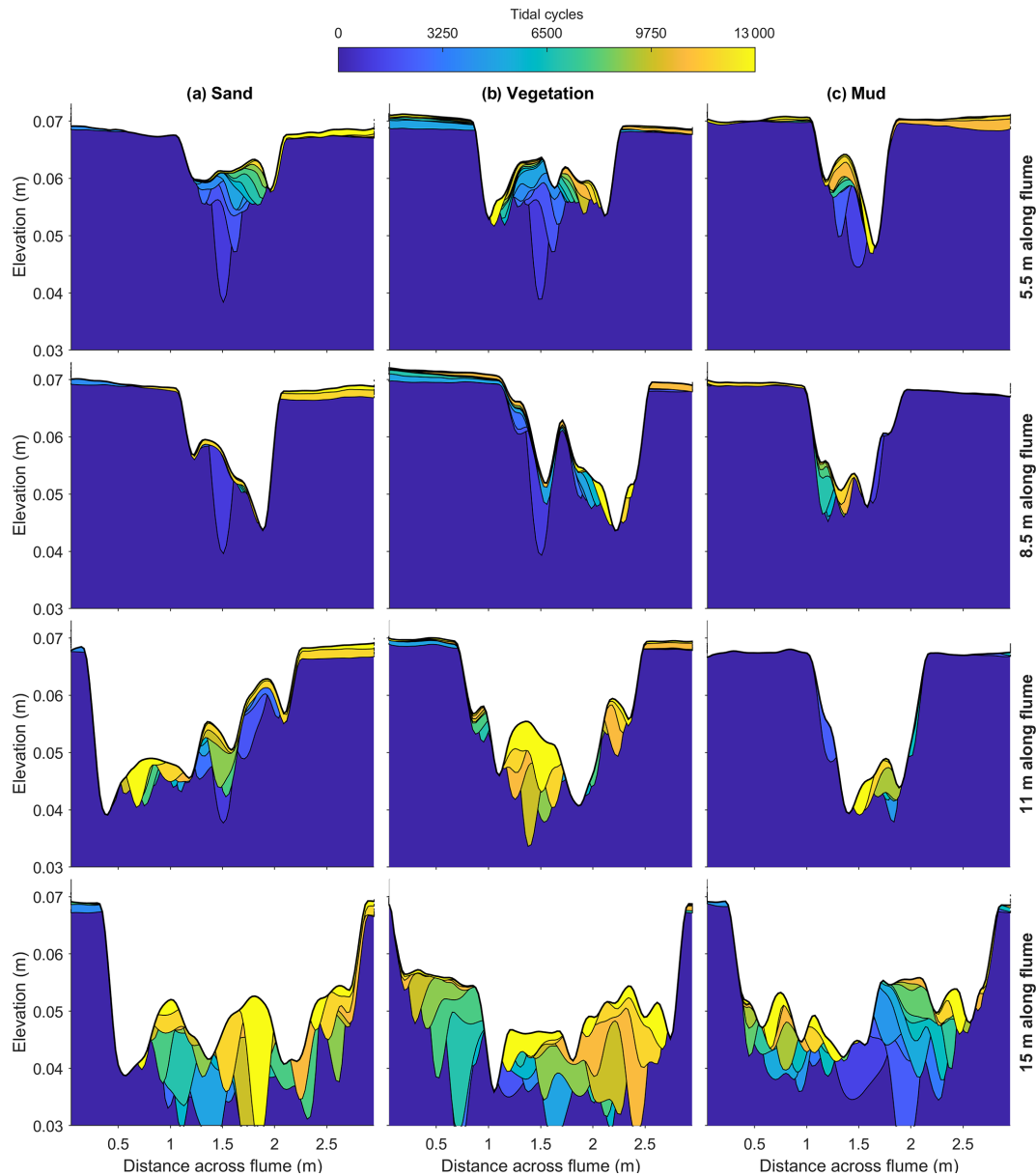
Figure 6. Cross sections with age of deposit, showing the preserved part of the morphodynamics in the experiments with (a) sand only, (b) vegetation and (c) mud for four positions along the flume. Bed level data of every 1000 cycles were used. The vertical exaggeration is a factor of 50.
