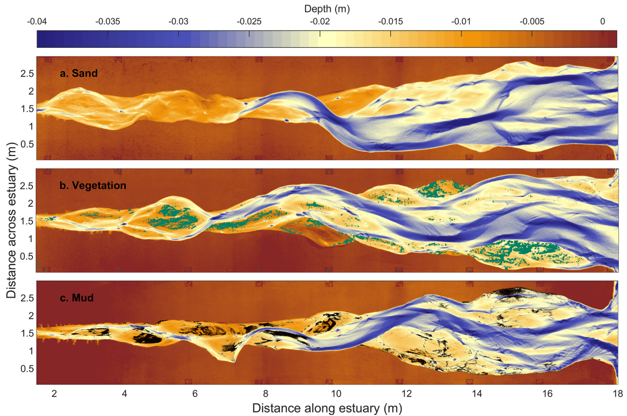
Figure 2. Bathymetry after 13 000 tidal cycles (see movie in the Supplement). (a) Control experiment with only sand. (b) Estuary with two vegetation species, with cover indicated in green. For visualisation, the binary map of vegetation was dilated by a kernel of 4 mm in MATLAB. (c) Estuary with mud simulant, with cover indicated in black (low mud experiment from Braat et al., 2019).
