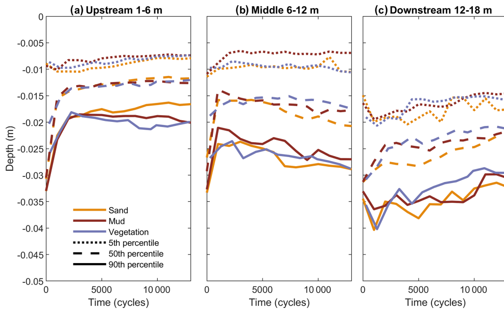
Figure 3. Time series of estuary depth below initial bed level, subdivided into an (a) upstream part (1–6 m), a (b) middle part (6–12 m) and a (c) downstream part (12–18 m). The 5th, 50th and 90th percentiles of depth represent the shoal depth, the median depth and the main channel depth.
