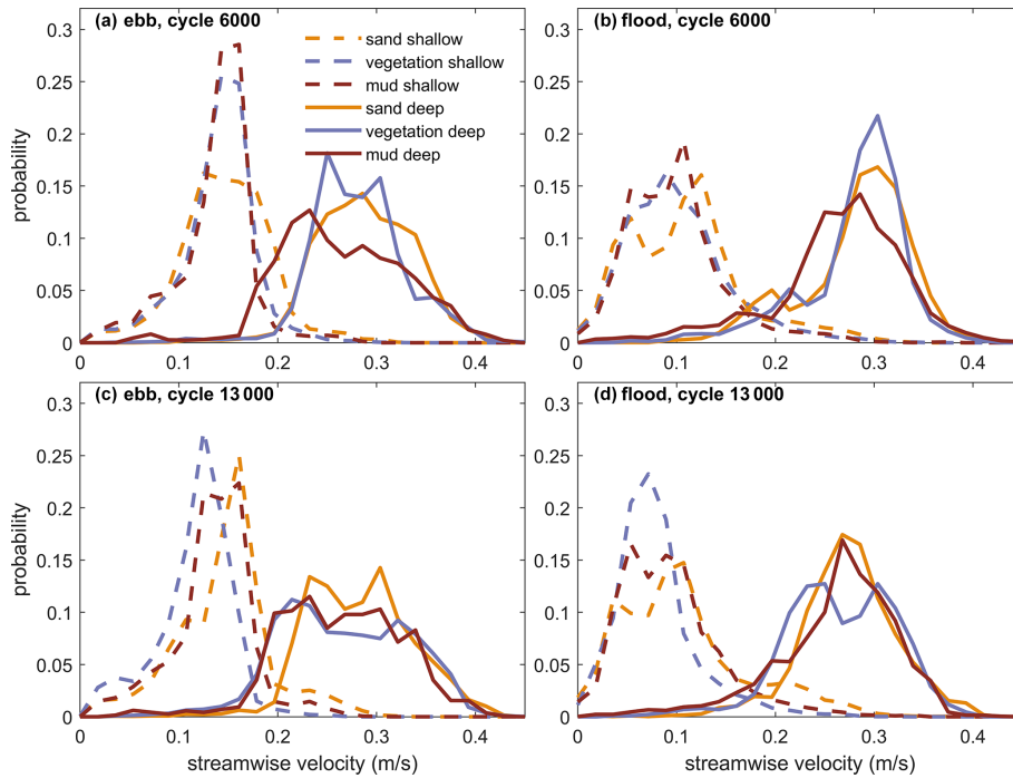
Figure 9. Distributions of maximum flow velocity calculated with the flow model for the middle (top; a, b ) and end (bottom; c, d ) of the experiment during flood (left; a, c ) and during ebb (right; b, d ). The selected depths ranges are shoal areas ( 0 > \text{depth} > -0.015 m) and channels ( -0.025 > \text{depth} > -0.050 m) for consistency with Fig. 3b.
