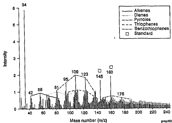
Figure 2. Py-MS spectra of Monterey-25 kerogen. For quantitation poly-4- t -butylstyrene was co-pyrolysed, which gives rise to its monomer, 4- t -butylstyrene ( m/z 160, 145).
