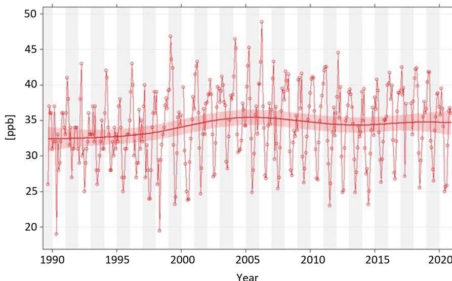
Figure 20. Monthly median concentrations of \text{O}_3 at the Zeppelin Observatory during 1989 to 2020 (ppb). Superimposed on the data is a smooth trend function (based on a generalized additive model (GAM) as provided by the smoothTrend function in the R library). Together with the trend is the 95 % confidence interval shown as a band.
