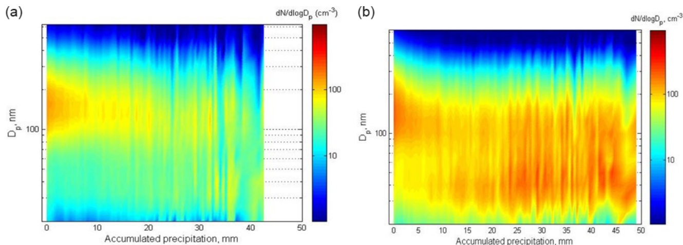
Figure 10. Evolution of aerosol number size distribution ( dN/d\log D_p ) as a function of accumulated precipitation along 240 h trajectories (a) for the dark period (October to February) and (b) for the sunlit period (March to September). All data from 2000 to 2010 (Tunved et al., 2013).
