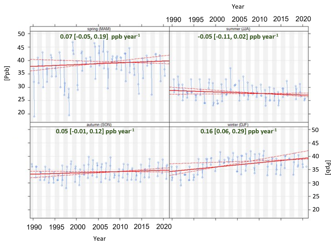
Figure 21. Theil–Sen slopes and confidence intervals for monthly median \text{O}_3 concentrations (ppb) at the Zeppelin Observatory during 1989 to 2020 for four seasons separately.
