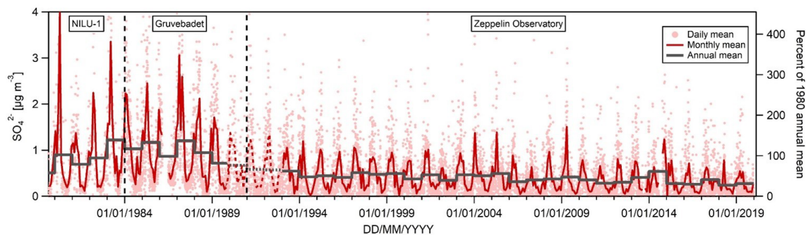
Figure 3. Sulfate ( \text{SO}_4^{2-} ) concentrations at Ny-Ålesund (NILU-1), Gruebadet, and the Zeppelin Observatory. Sulfate is sea salt corrected except for 1990–1992 where total sulfate was measured, as also indicated by the dashed line. For reference, the right axis shows levels relative to the 1980 annual mean of 0.92 \mu\text{g m}^{-3} . Daily and annual means calculated only where data coverage is \geq 75\% of the total day or year, respectively.
