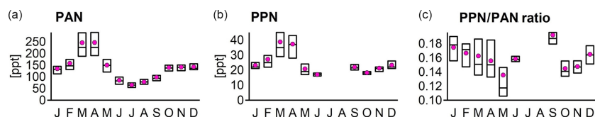
Figure 22. Boxplot of monthly variation (box top and bottom: 75th and 25th percentiles, respectively, horizontal bar: median) and monthly averages (pink) of peroxyacetyl nitrate (PAN), peroxypropionyl nitrate (PPN), and the PPN / PAN ratio at the Zeppelin Observatory in 1994 to 1996.
