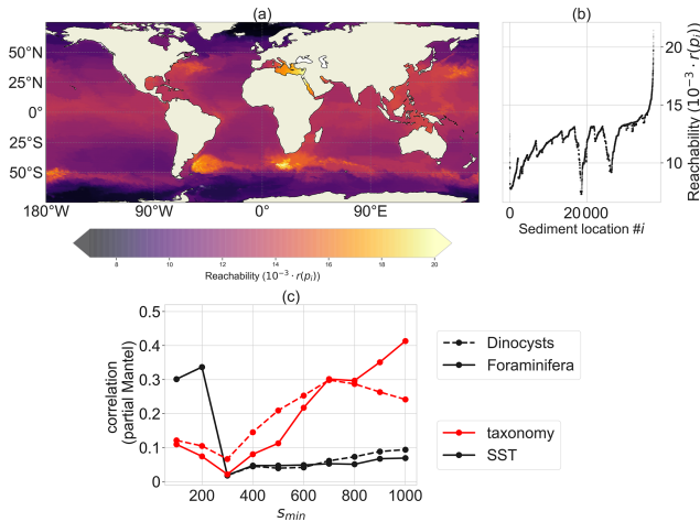
Figure 3. Reachability plot of the sedimentary particle release locations from the OPTICS algorithm. Sediment locations in dense areas (i.e. with low reachability values in a ) share a similar particle distribution of backtracked surface origin locations, while areas with high reachability values have backtracked particle distribution which are more spread out and share origin locations with a lot of other sedimentary release locations. A sinking speed of 6 \text{ m d}^{-1} is used and parameter s_{\text{min}} = 300 (i.e. OPTICS clusters will consist of a minimum of 300 sediment sites). (a) Site reachability in space: sites in dense areas with a low reachability are oceanographically isolated. (b) A scatter plot of the ordering of the sediment locations i against their reachability r(p_i) . (c) Partial Mantel correlation of the reachability distance D^r (a lower value of D^r between two sites indicates a stronger oceanographic connection between these sites; see Appendix B) with the taxonomy (red) and SST (black), both with spatial distance held constant, for different s_{\text{min}} values. A total of 999 permutations were used for every partial Mantel test; every test with respect to the taxonomy (red) is significant with p value < 0.003 .
