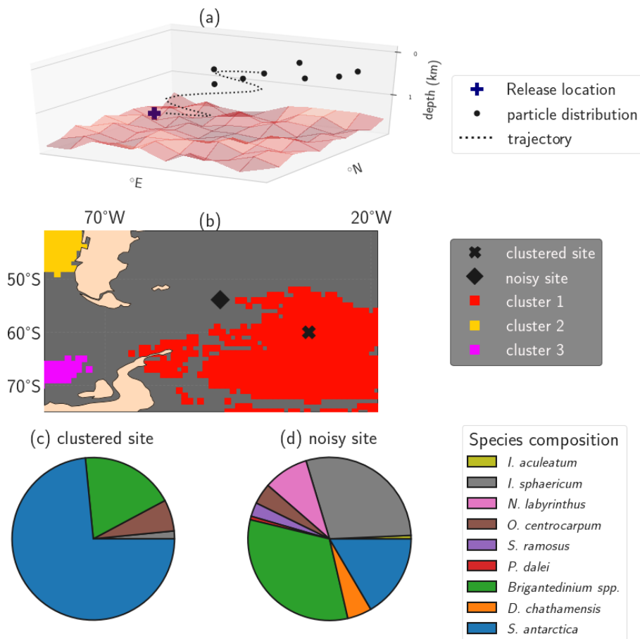
Figure 1. Illustration of the impact of isolated clusters on sedimentary microplankton composition. (a) Illustration of the particle backtrack analysis from Nootboom et al. (2019), resulting in a particle distribution of origin locations for one sediment site or release location on which the clustering methods are applied (figure adapted from Nootboom et al., 2020). (b) A (noisy) sediment sample site outside of the isolated clusters (station J299) and a site within oceanographically isolated OPTICS cluster 1 (station J285) in the South Atlantic. (c, d) Pie charts of the dinocyst species composition in the sites from (b) . The clustered site contains a species composition which is less biodiverse compared to the noisy site. The Shannon biodiversity indices of respectively the clustered and noisy site are 0.7788 and 1.6842. This illustration uses the same OPTICS clusters as are shown later in Fig. 4.
