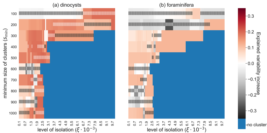
Figure 6. Increase in explained environmental variability by microplankton sediment sample sites in the CCA analyses if sediment samples outside of the oceanographically isolated OPTICS clusters are excluded, for different parameter values s_{\min} (i.e. the minimum size of clusters) and \xi (i.e. the level of isolation). (a) The dinocyst and (b) the foraminifera dataset. High and significant values indicate that sediment samples within clusters have a clearer relationship with the surface environment. Blue are configurations of s_{\min} and \xi for which no sediment sample sites are part of a cluster. Only Southern Hemisphere sedimentary microplankton data were used here. Vertical stripes indicate an insignificant randomisation test with 999 permutations at a 5 % significance level.
