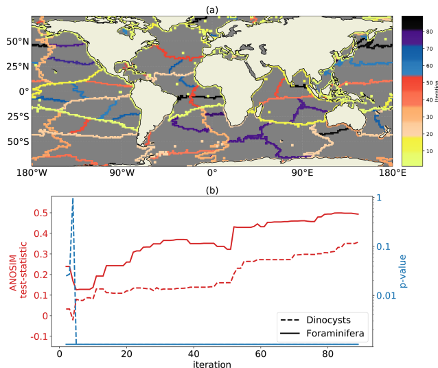
Figure 2. Edges between oceanographically disconnected clusters of sedimentary locations from the hierarchical clustering method. (a) The cluster edges after 90 iterations, where the colour indicates at which iteration number a cluster edge is created. (b) The ANOSIM test statistic (red) and p values (blue; 999 permutations; logarithmic scale) for the clusters at every iteration number, which tests whether the sedimentary microplankton composition (both dinocysts and foraminifera; sites below 65^{\circ} N) is more similar within than between clusters.
