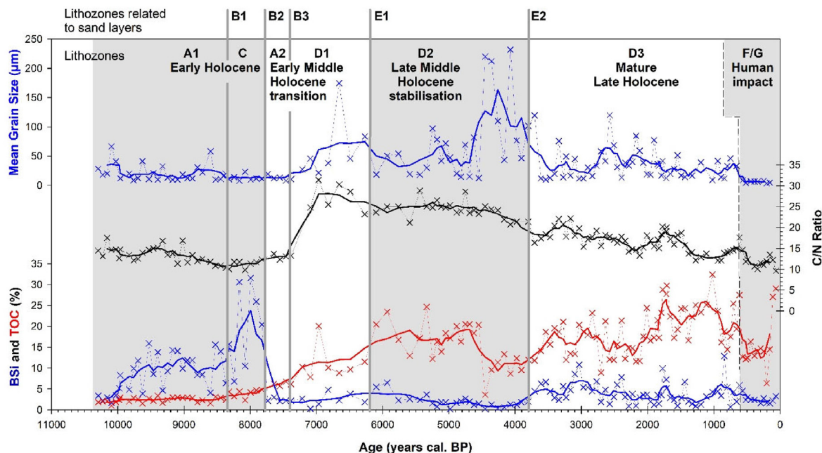
Fig. 8. Selected geochemical data (biogenic silica: BSi; total organic carbon: TOC; carbon-to-nitrogen ratio: C/N ratio) are shown together with mean grain size vs. time. Lithozones and the position of sand horizons (LZs B and E) excluded from age-depth modelling are labelled as well as stratigraphical assignments and human impact.
