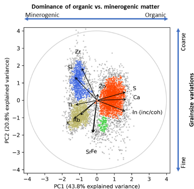
Fig. 4. PCA loadings from homogenized (clr-transformed) elemental intensities obtained by XRF core scanning. The first two principal components preserve 64.6% of the total variance. The four determined clusters (Cluster 1–4) are color-coded (for legend: cf., Fig. 2) and data points related to noise are plotted in gray. The circle indicates a value of 1 for the loadings. Interpretations in terms of grainsize variations and dominance of organic vs. minerogenic matter are indicated by blue arrows. (For interpretation of the references to color in this figure legend, the reader is referred to the Web version of this article.)
