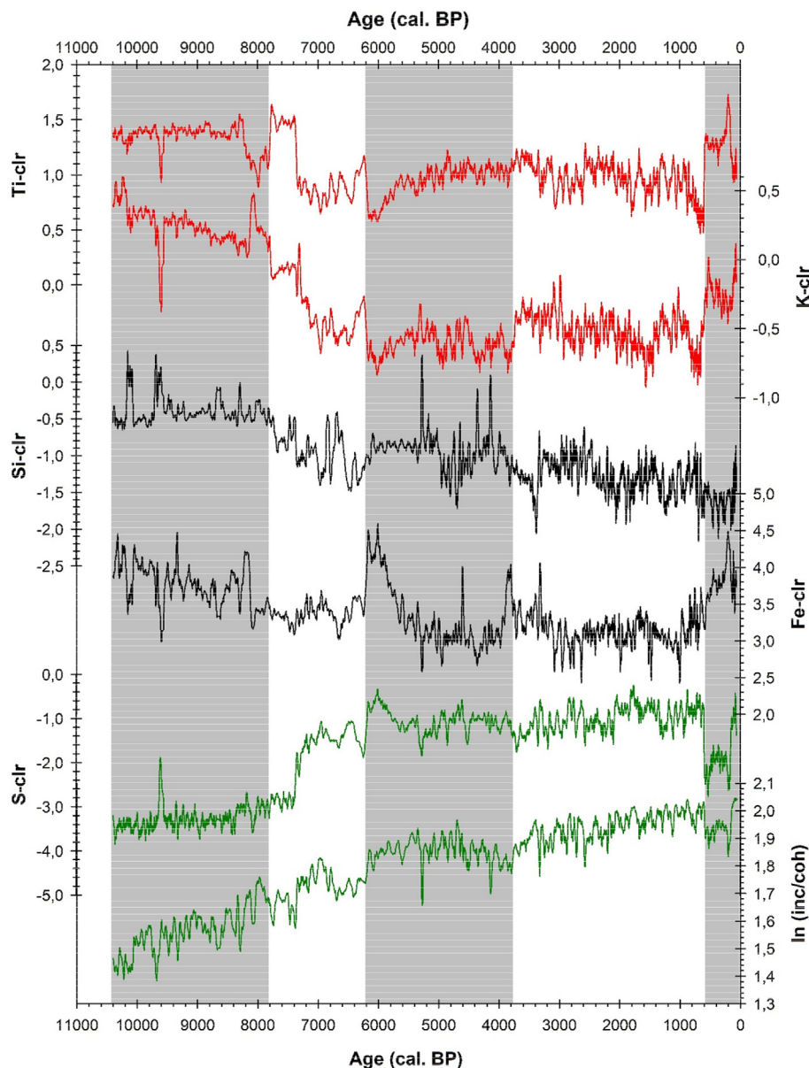
Fig. 9. Selected clr-transformed elemental data obtained by XRF core scanning. Shown are the elements sulphur (S), silica (Si), titanium (Ti), potassium (K), iron (Fe) and the log incoherent/coherent ratio ( \ln \text{inc/coh} ) vs. time. Shading as in Fig. 8.
