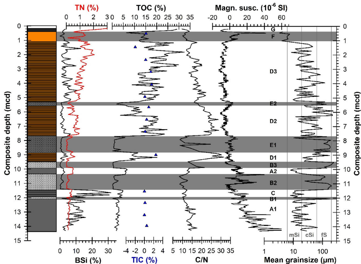
Fig. 3. Litholog with lithozones A1 through G (for legend: cf., Fig. 2) with bulk geochemistry, including total nitrogen (TN), total organic carbon (TOC), total inorganic carbon (TIC), magnetic susceptibility (Magn. susc.), biogenic silica (BSi), carbon-to-nitrogen ratio (C/N) and mean grainsize. Sand horizons (LZs B and E) and lithozone F are shaded in gray.
