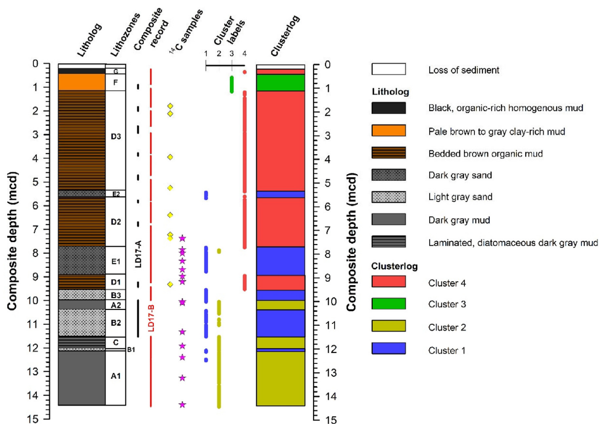
Fig. 2. Litholog (left) of the composite record based on macroscopic and microscopic observations with lithozones A1 through G, core sections used for the construction of the composite record as well as positions of samples for radiocarbon ( ^{14}\text{C} ) dating. Radiocarbon ages of terrestrial macrofossils are shown as yellow diamonds and those on bulk organic matter as pink stars. All data related to ^{14}\text{C} dating are provided with Table 1. Clusterlog (right) based on cluster analysis for comparison. (For interpretation of the references to color in this figure legend, the reader is referred to the Web version of this article.)
