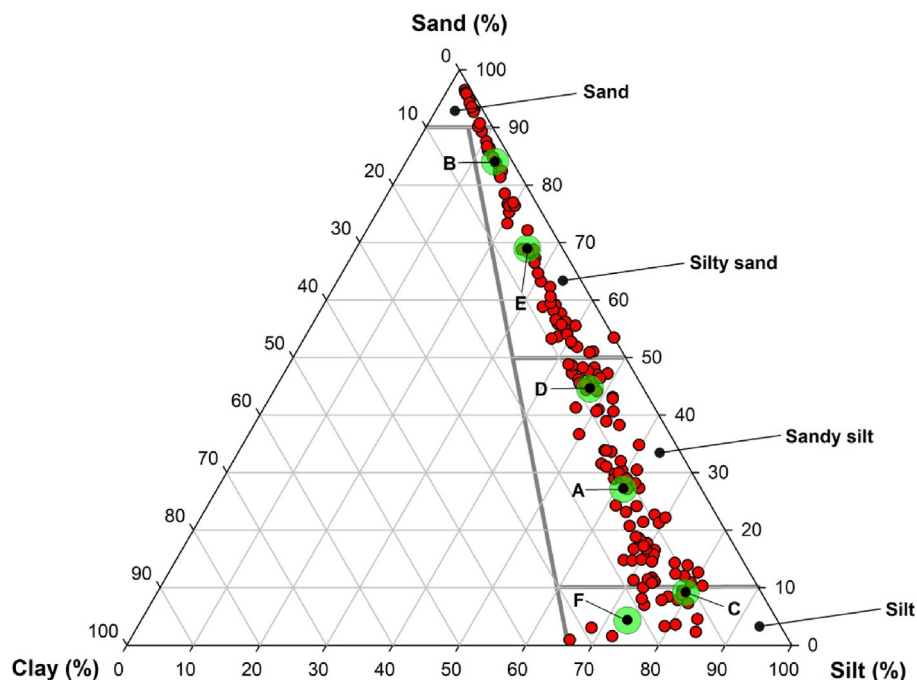
Fig. 6. Ternary grainsize diagram (red dots mark individual samples) with mean grainsize values for lithozones A-F (labelled with the corresponding letter and encircled in green color). (For interpretation of the references to color in this figure legend, the reader is referred to the Web version of this article.)
