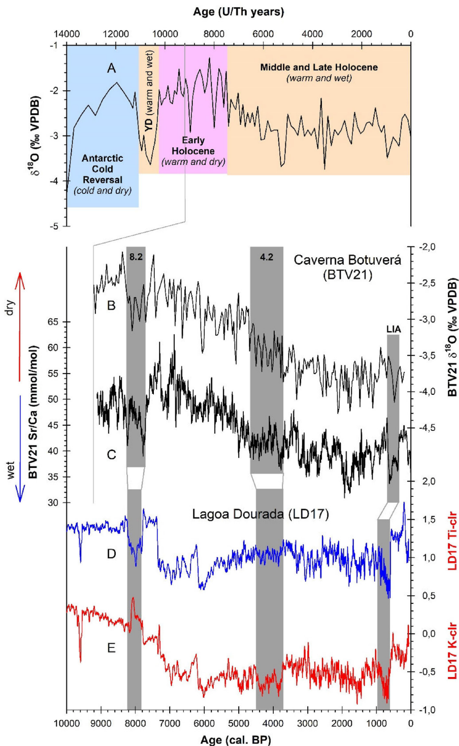
Fig. 10. Comparison of speleothem data from Caverna Botuverá with lacustrine sediment data from Lagoa Dourada, both S Brazil. A) Oxygen isotope record from Botuverá speleothem BTV2 focusing on the last 14 ka (Cruz et al., 2005a, 2005b). Climatic conditions are labelled and color-coded (YD: Younger Dryas) and derived from Novello et al. (2017). Note that this time scale is in U/Th years! B) Oxygen isotope record and C) Sr/Ca ratio from Botuverá speleothem BTV21 for the Holocene (Bernal et al., 2016a, 2016b) with hydroclimatic interpretation (arrows). Additionally, clr-transformed elemental data of D) titanium (Ti) and E) potassium (K) are shown from the sediment record of Lagoa Dourada. The three most prominent Holocene climatic events are marked by vertical gray bars. Note: the chronology for the last millennium of the Lagoa Dourada record is shown with the “rbacon” age-depth model causing a temporal offset for the last millennium – for explanation see the text. All data from Caverna Botuverá were accessed online via the NOAA Paleoclimatology Program on February 18, 2021. (For interpretation of the references to color in this figure legend, the reader is referred to the Web version of this article.)
