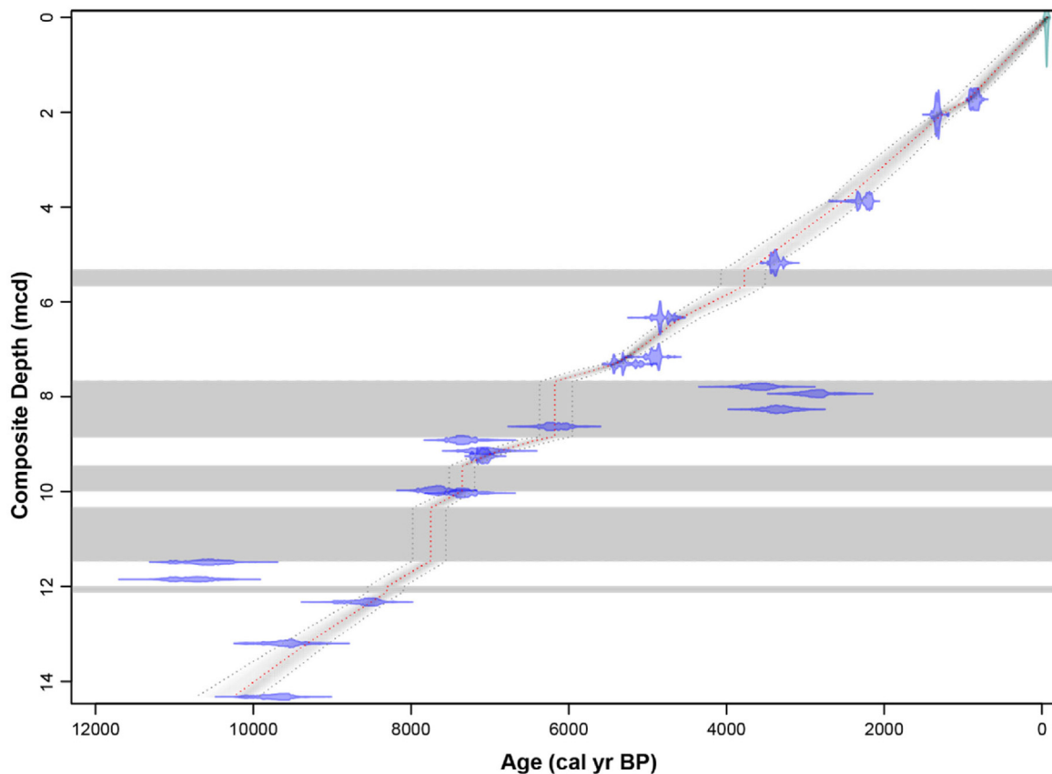
Fig. 7. Age-depth relationship (red dotted line) modelled with “rbacon” and based on 21 radiocarbon dates (in blue) with the sediment surface (in green). The 1\sigma error margins (gray dotted lines) are indicated as well as the five sand horizons (gray horizontal bars) excluded from age-depth model calculations. (For interpretation of the references to color in this figure legend, the reader is referred to the Web version of this article.)
