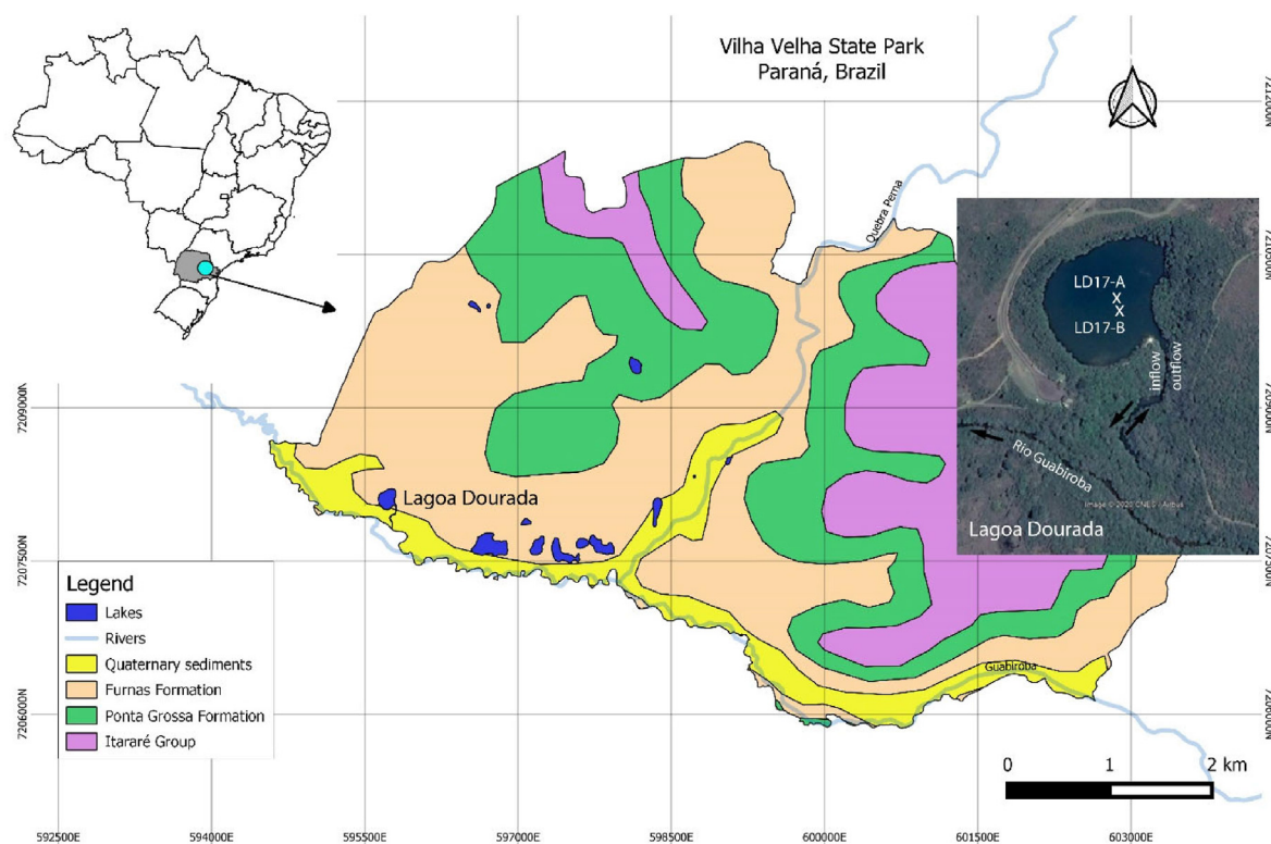
Fig. 1. Location of Lagoa Dourada in Paraná (S Brazil) with a geological map of the Vila Velha State Park based on information from “Plano de Manejo Vegetação Parque Estadual Vila Velha” (Governo do Estado de Paraná, 2004) and an aerial photography of the lake with Rio Guabirola from Google Earth. Coring locations LD17-A and LD17-B are marked (X) in the aerial photography.
