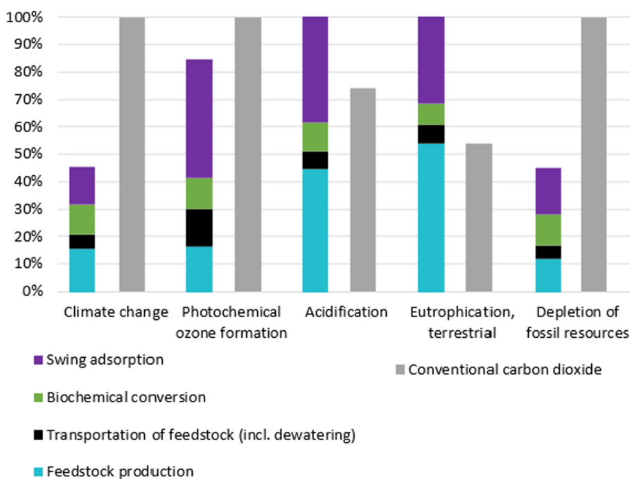
Fig. 6. Cradle-to-gate comparison between the bio-based carbon dioxide (left bar) delivered by this innovative process (with process contributions highlighted) and conventional carbon dioxide. Values are normalized taking the most impacting value per each category valued as 100%.
