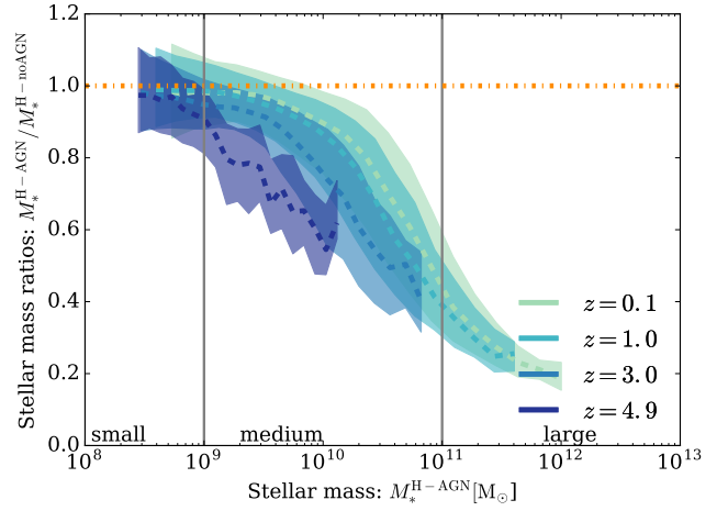
Figure 5. Quenching mass ratios, i.e. stellar mass ratios of twinned galaxies in H-AGN and H-noAGN. The twins are mass binned by stellar mass in H-AGN, M_{*}^{\text{H-AGN}} , with the median value (dashed lines) and quartile error ranges (shaded region) plotted for each bin. If AGN feedback had no effect, the quenching mass ratio would lie on the horizontal dotted line, which denotes twin galaxies having identical mass. Note the non-linear evolution of the quenching mass ratio with galaxy mass, with small galaxies ( M_{*}^{\text{H-AGN}} < 10^9 M_{\odot} ) barely affected, and large galaxies ( M_{*}^{\text{H-AGN}} > 10^{11} M_{\odot} ) being most strongly quenched. This plot also shows a redshift evolution, with smaller galaxies more affected at higher redshift.
