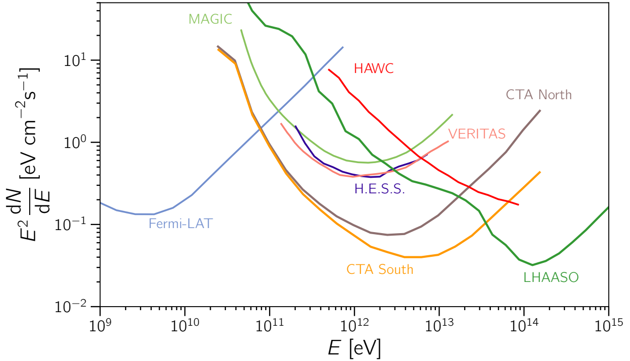
Figure 9: The differential sensitivity of several gamma-ray detectors operating in the GeV–PeV energy range. Sensitivities CTA [1119], H.E.S.S. [1123], MAGIC [1114], and VERITAS [1124] are for 50 hours of observation. The flux sensitivities for HAWC [1125] and LHAASO [1126] correspond to approximately 3000 hours and 1 years, respectively. The Fermi-LAT band includes sources at various positions in the sky, for the P8R3_SOURCE_V2 instrument response function [1127].
