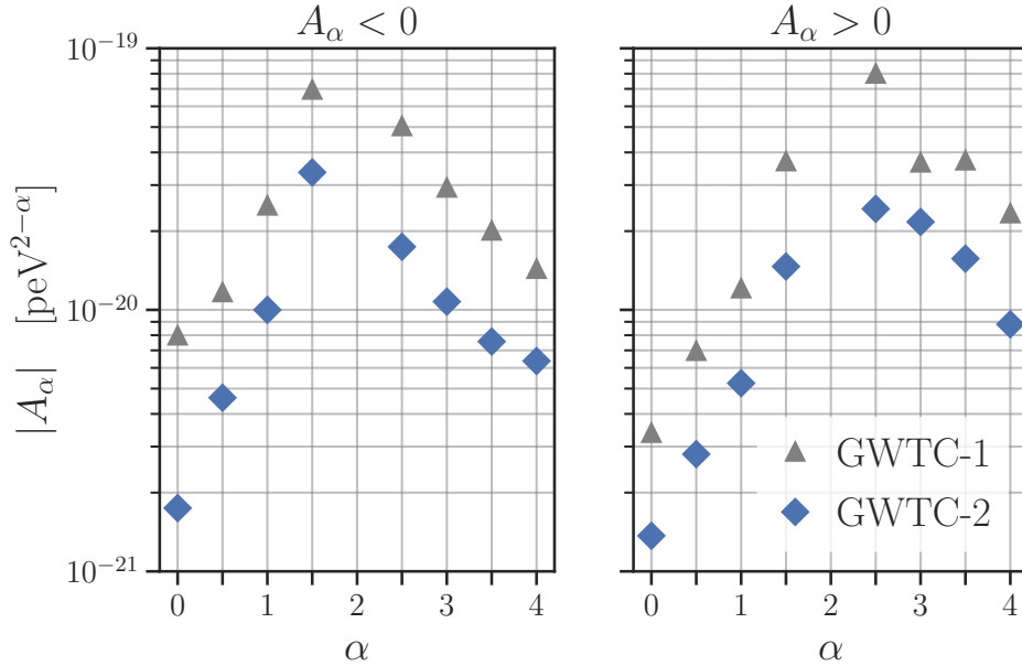
Figure 12: Bounds on MDRs from the second LIGO–Virgo Gravitational-Wave Transient Catalog [1507]. Constraints on the allowed amount of dispersion through the 90%-credible upper limits on A_\alpha (corresponding to A in the main text), computed separately for A_\alpha > 0 and A_\alpha < 0 . Marker style distinguishes the new GWTC-2 results from the previous GWTC-1 results in [1508]. Figure taken from [1507].
