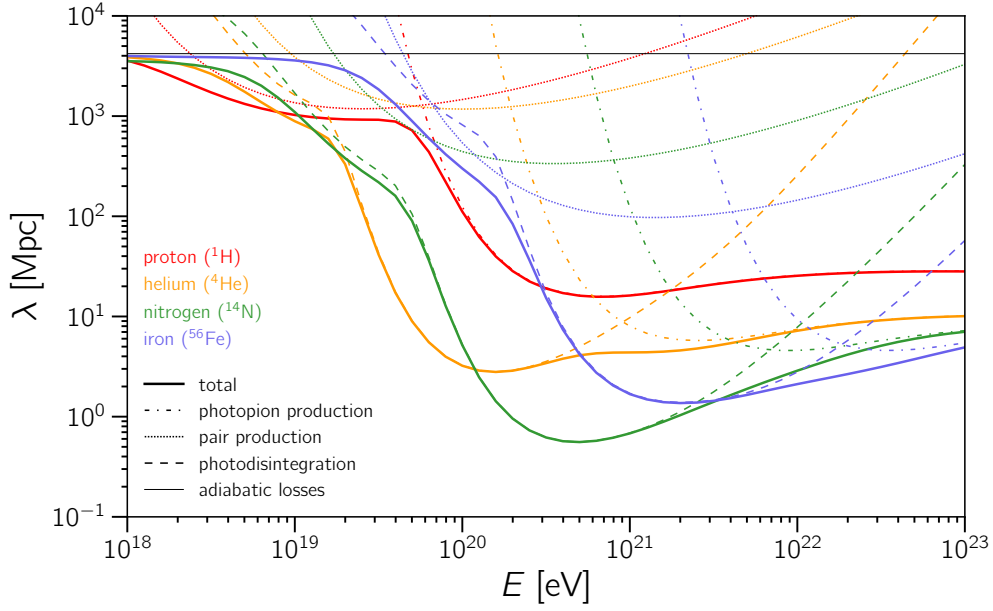
Figure 6: Energy loss length ( \lambda ) as a function of the UHECR energy ( E ), assuming the EBL model from [927] and the photodisintegration model from [939] (helium), [940] (nitrogen and iron).
