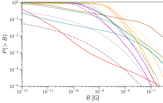
Figure 7: Left: the “filling factor” of IGMFs (i.e. the volume fraction of the universe in which the magnetic field strength is greater than the specified amount) as predicted by various models, from Ref. [644]. Right: deflections of cosmic rays with E = 20Z \text{ EeV} (squares are source positions and circles are arrival directions at Earth) by the regular GMF as predicted by various models, from Ref. [950].
