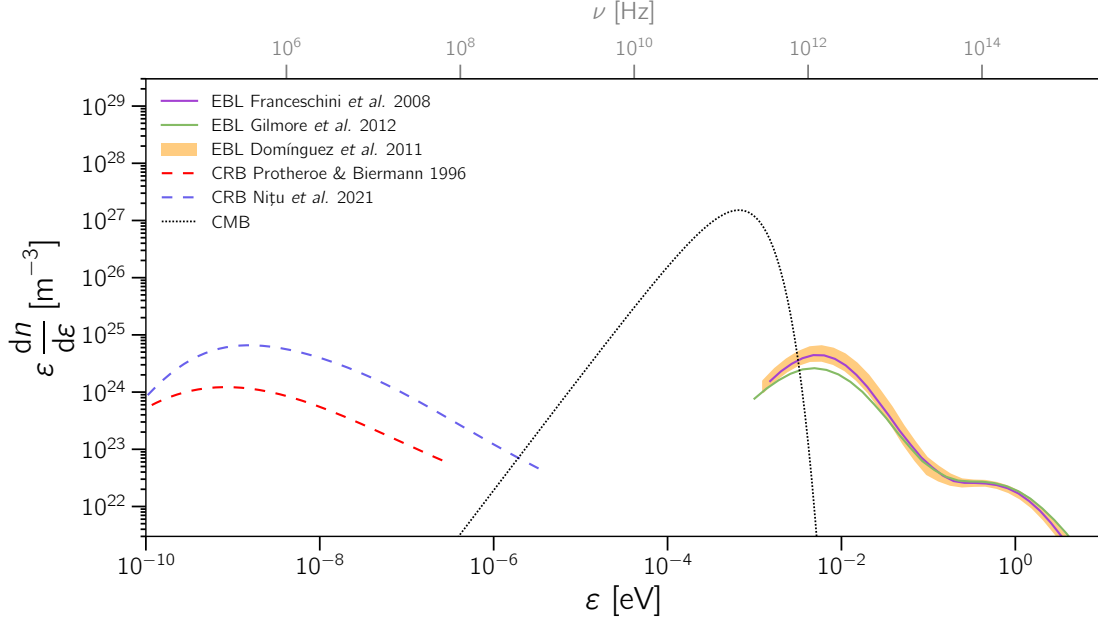
Figure 4: Compilation of the density of background photons ( n(\varepsilon) ) with different energies ( \varepsilon ) at present time for a wide range of frequencies ( \nu , shown at the top). Here the dashed lines correspond to the CRB, the dotted line to the CMB, and the EBL is represented by solid lines. Lines of different colors correspond to different models: Protheroe & Biermann [924], Nițu et al. [925], Franceschini et al. [926], Gilmore et al. [927], and the model by Domínguez et al. [928], with uncertainties.
