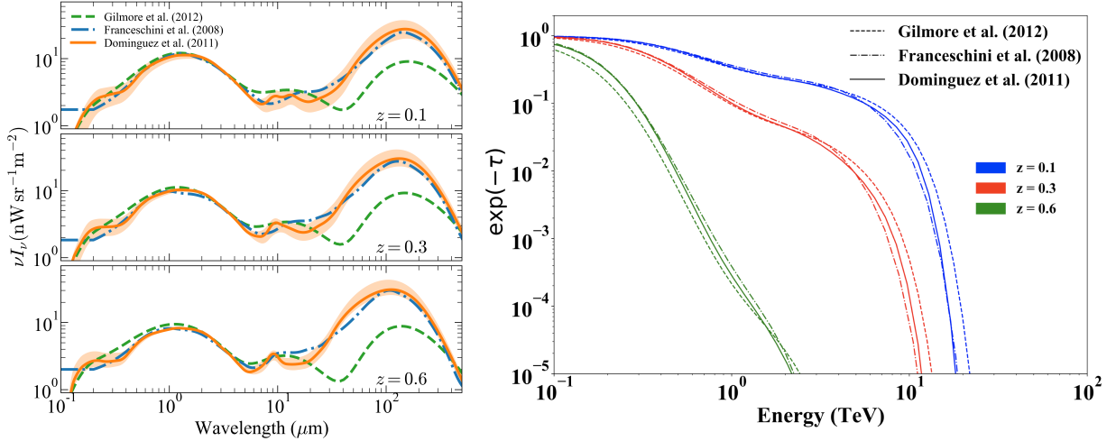
Figure 5: Left. Comparison of the EBL intensity of three models [926–928]. The orange bands represent the model uncertainties reported in [928]. Each panel considers a different redshift as indicated. Right. The absorption coefficient as a function of the observed gamma-ray energy for gamma rays coming from sources at different redshifts (indicated by different colors), obtained from three different EBL models as indicated.
