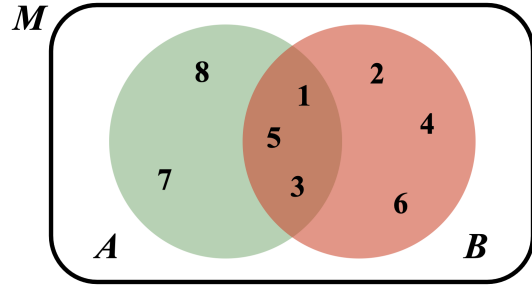
Figure 1: An example of a model of the form \mathcal{M} = \langle M, A, B, < \rangle . The numbers represent the objects in the domain and they correspond to the position of the objects in the order < . The sentence “the first 3 bicycles are red” is true in this model, as the first three objects in A (the objects with position 1, 3, and 5 in the order < over the whole domain) are also in B .
