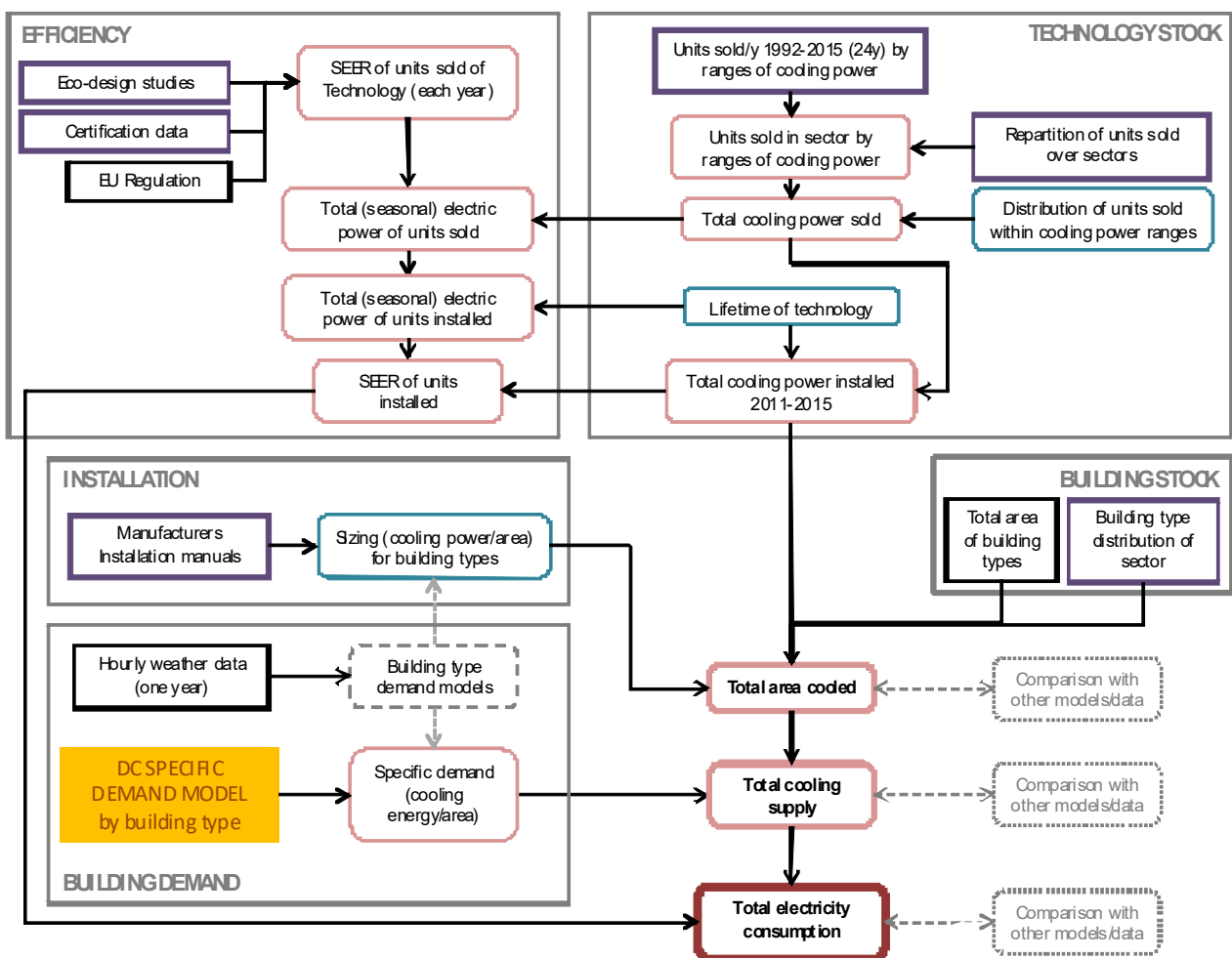
Figure 3: Overview of method for space cooling demand estimation
