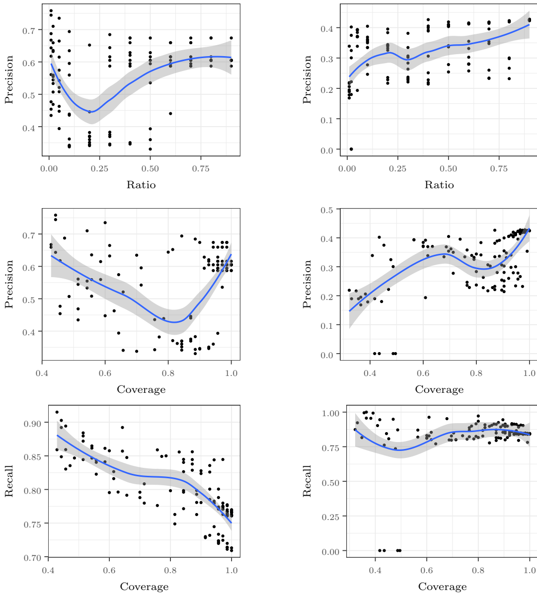
Figure 4: Plots of ratio and precision, and coverage with precision and recall for the Road Fine log (left) and the Sepsis log (right).
