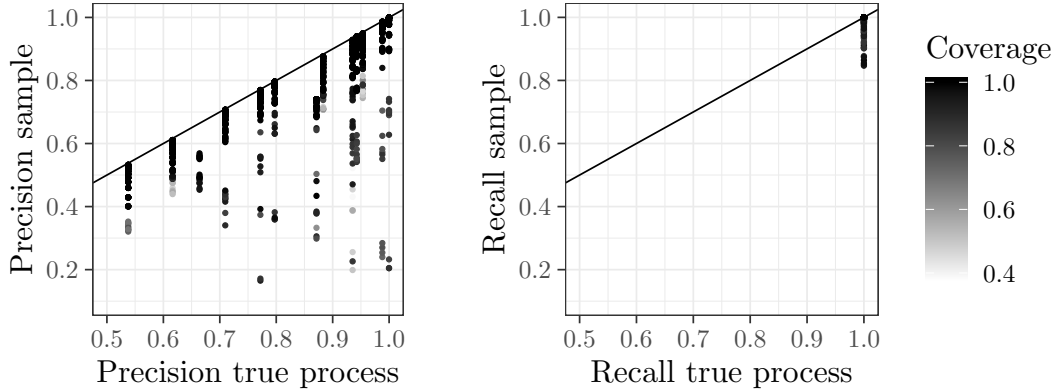
Figure 2: Relation between the quality of the true process and the quality of the discovered models, for precision (left) and recall (right). Darker points represent a higher coverage.
