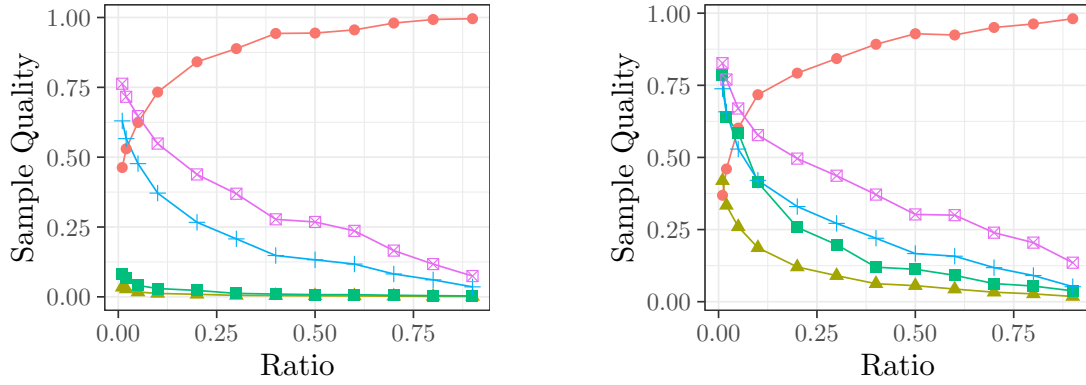
Figure 3: Plot of ratio and the sample quality measures coverage ( \bullet ), sMAPE ( + ), sRMSPE ( \boxtimes ), NRMSE ( \blacksquare ) and NMAE ( \blacktriangle ) for the Road Fine log (left) and the Sepsis log (right).
