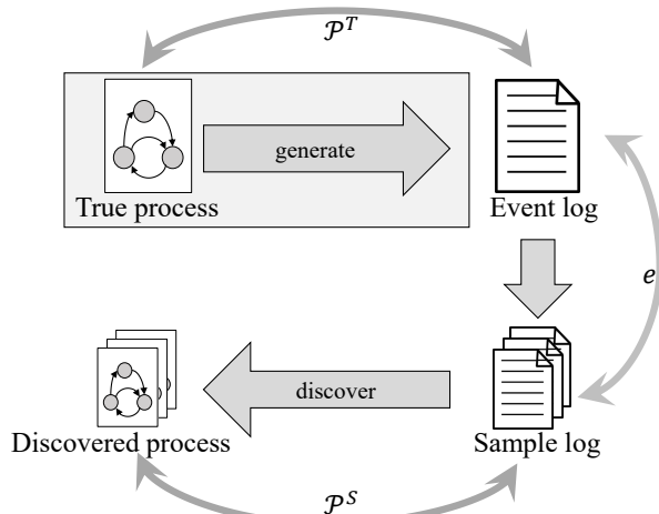
Figure 1: True process generates an event log L with unknown quality \mathcal{P}^T . Any sample S drawn from L has some error e . Discovering a model from S results in a model with quality \mathcal{P}^S .
