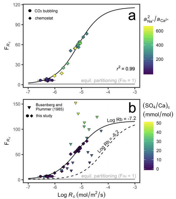
Fig. 5. Effect of crystal growth rate on calcite \text{Na}/\text{Ca} expressed with the term F_{R_c} (i.e. the effect of the solution (\text{Na}^+)/\text{Ca}^{2+} activity ratio on (\text{Na}/\text{Ca})_c was removed; see Eqs. (20)–(22)). (a) Results for all the calcite experiments carried in this study and best-fit line (continuous black curve) obtained with Eq. (22) and R_b = 10^{-7.2} mol/m 2 /s, \Delta_{\text{eq}} = 6.3 \times 10^{-5} and \Delta_f = 7.4 \times 10^{-3} . This panel shows a crystal growth rate effect on calcite \text{Na}/\text{Ca} that is independent of the solution (\text{Na}^+)/\text{Ca}^{2+} activity ratio. (b) same as (a) but with additional data calculated from the Busenberg and Plummer (1985) calcite experiments. The effect of calcite \text{SO}_4/\text{Ca} on (\text{Na}/\text{Ca})_c is apparent. F_{R_c} values that are significantly lower than the continuous black curve may be explained by lower R_b values (e.g. dotted black curve obtained with R_b = 10^{-6.2} mol/m 2 /s). Uncertainties in \log R_c values (error bars) are mostly due to the uncertainty in the surface area of calcite crystals during the course of an experiment.
