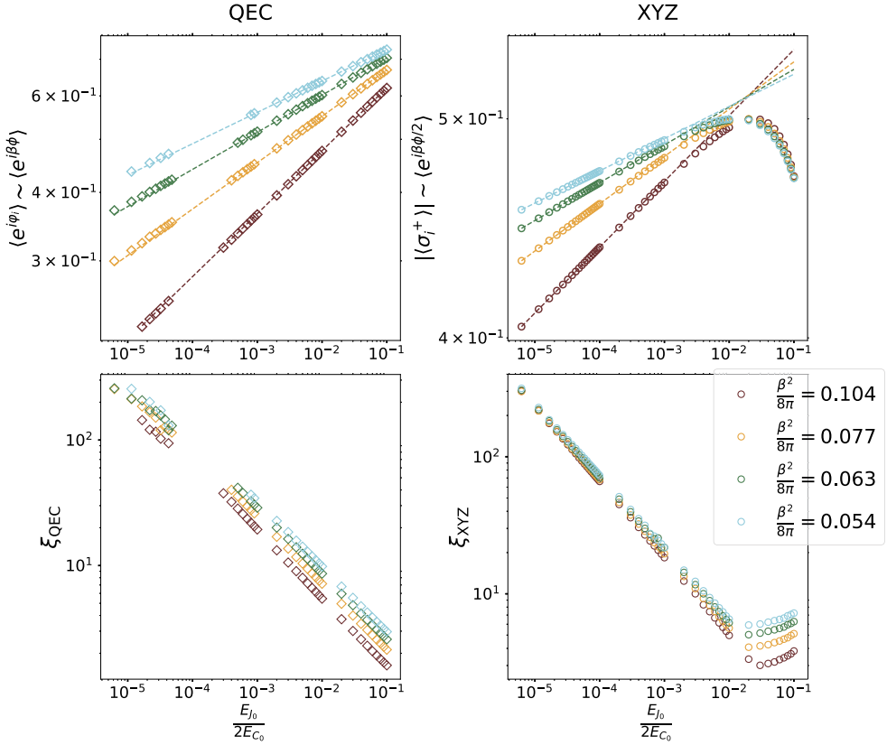
Fig. 7. Comparison of the expectation values of the vertex operators obtained using infinite DMRG for the QEC lattice model ( \langle e^{i\varphi_i} \rangle \sim \langle e^{i\beta\phi} \rangle , top left) and the XYZ chain ( |\langle \sigma_i^+ \rangle| \sim \langle e^{i\beta\phi/2} \rangle , top right) as a function of M_0/2 \propto E_{J_0}/2E_{C_0} , the mass-parameter of the qSG field theory [see Eqs. (12), (13)]. The field theory computations for both the quantities predict a linear dependence (see Figs. 4, 6). For very small M_0/2 , where the correlation-length is large for both QEC and the XYZ lattice models and the continuum qSG description is valid for both models. As E_{J_0}/E_{C_0} increases, the correlation length diminishes and the corrections to scaling becomes important. However, as seen from the QEC plot, the expectation value of the vertex operator continues to follow the straight line, while that from the XYZ chain deviates from the field theory predictions at E_{J_0}/E_{C_0} \sim 10^{-3} . This difficulty of reaching the scaling regime for the XYZ chain occurs in the region where |J_x - J_y| is no longer \ll |J_x - J_z| . Then l no longer tends to zero and thus, the correlation length \xi_{\text{XYZ}} is no longer large [see Eq. (15)]. We do not go beyond E_{J_0}/2E_{C_0} = 0.1 since the correlation length for both the XYZ and the QEC models is only a few lattice sites and it is not meaningful to apply the qSG field theory predictions beyond this point. For reference, the corresponding correlation lengths are shown in the bottom left and bottom right panels. Note that the correlation length for the XYZ chain actually goes up for E_{J_0}/E_{C_0} > 10^{-2} . This is because for this choice of parameters, the XYZ chain is no longer in the scaling limit and increasing the aforementioned ratio no longer corresponds to increasing the mass gap of the model (see main text for more details).
