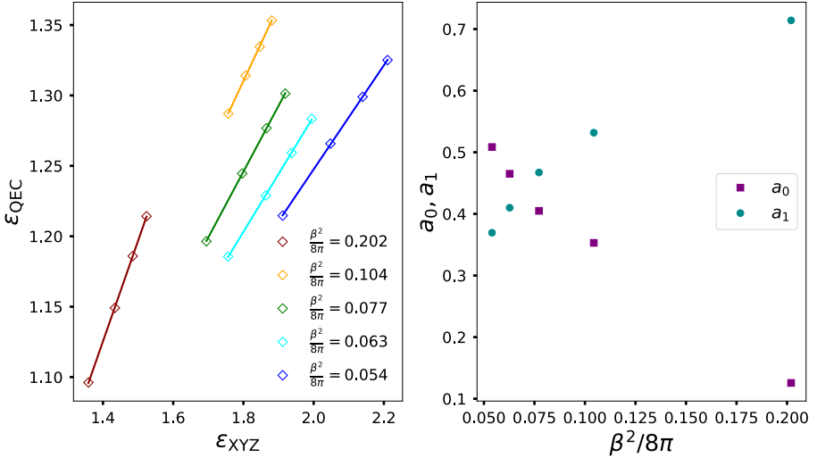
Fig. 12. (Left) Verification of the linear dependence of \varepsilon_{\text{QEC}} on \varepsilon_{\text{XYZ}} for different choices of \beta^2/8\pi . (Right) The parameters of the linear fit, a_0, a_1 [see Eq. (22)] as a function of \beta^2/8\pi .
