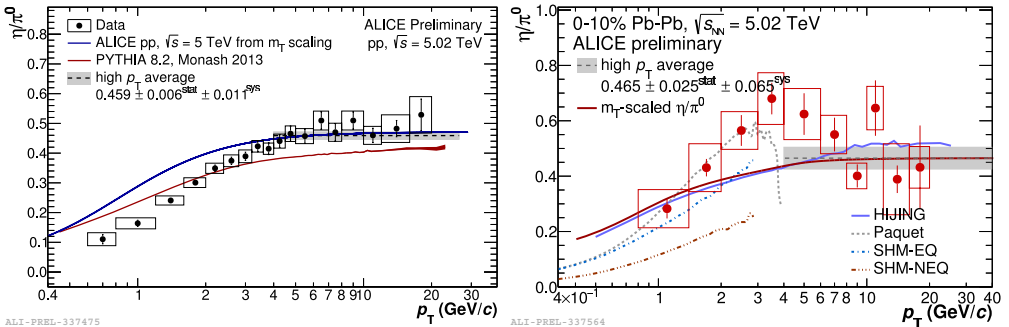
Fig. 2. The \eta/\pi^0 ratio for pp collisions at \sqrt{s} = 5 TeV (left), and Pb-Pb collisions at \sqrt{s_{NN}} = 5.02 TeV (right).
