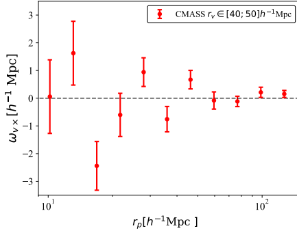
Figure B3. \times correlation for voids with r_v \in 40\text{-}50 h^{-1} Mpc.
