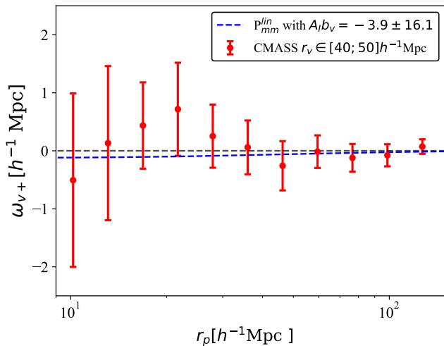
Figure 5. \omega_{v+} with r_v \in [40; 50] h^{-1} \text{Mpc} , and the large-scale prediction with A_I b_v = -3.9 \pm 16.1 . The signal at intermediate scales is too noisy to have a detection of alignments in the intermediate-scale regime.
