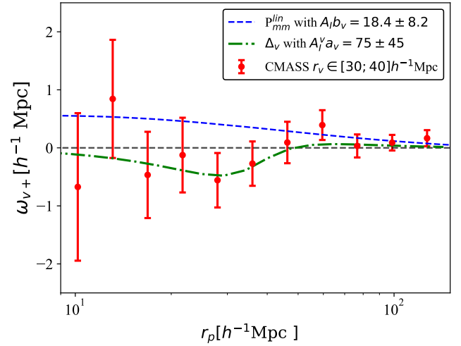
Figure 4. \omega_{v+} with r_v \in [30, 40] h^{-1} \text{ Mpc} , the intermediate-scale prediction with A_V^Y a_v = 75 \pm 45 , and the large-scale one with A_I b_v = 18.4 \pm 8.2 .
