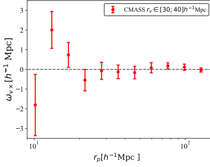
Figure B2. \times correlation for voids with r_v \in 30\text{-}40 h^{-1} Mpc.
