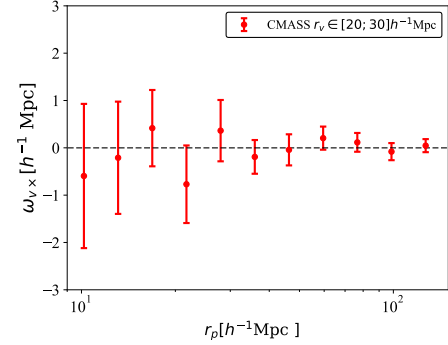
Figure B1. \times correlation for voids with r_v \in 20\text{--}30 h^{-1} Mpc.
