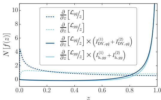
Figure 3. The derivative of the parton luminosity (dashed) and its point-by-point multiplication with the integrated LP partonic coefficient function up to NNLO (solid), for both DY (dark blue) and single Higgs (light blue) production at Q = \mu = 125 GeV. All curves are normalized according to eq. (2.16).
