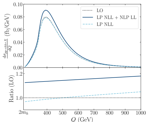
Figure 13. Differential cross section for hh production showing the LO (black dotted), LP NLL (dashed light-blue), and NLP LL + LP NLL (solid dark-blue) results. The scale \mu is set to Q/2 . The bottom panel shows the ratio with respect to the LO distribution.
