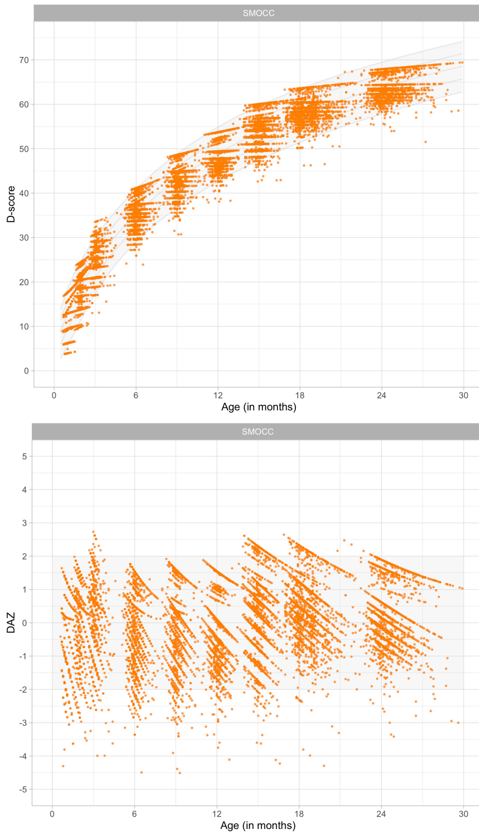
Figure 9.1. Distribution of D-score and DAZ by child age in a cohort of Dutch children aged 0-2 years (Source: SMOCC data, n = 2151 , 9 occasions).
