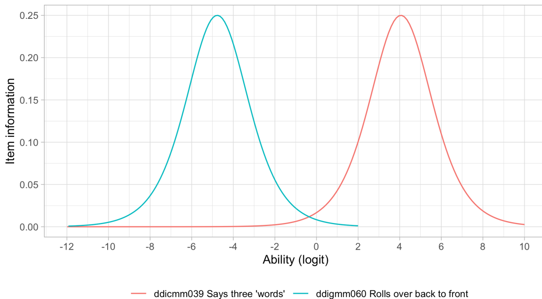
Figure 6.8. The item information curve for two milestones from the DDI.
