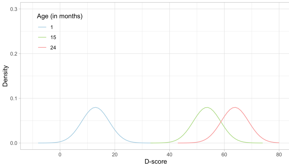
Figure 5.3. Age-dependent starting priors for the D-score at the ages of 1, 15 and 24 months.
