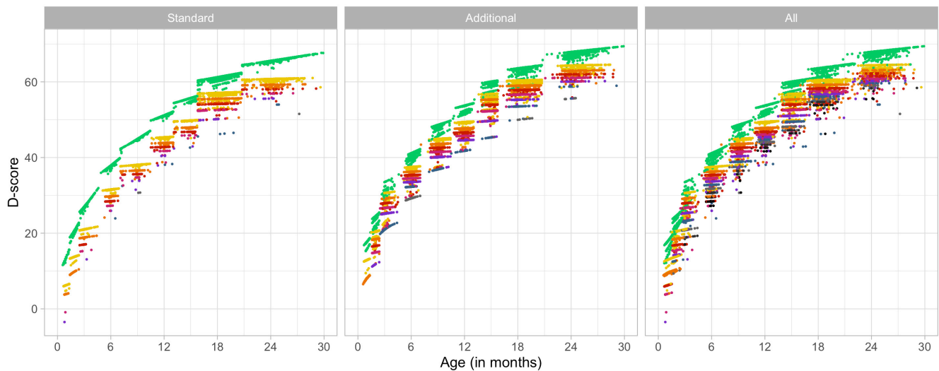
Figure 8.4. D-score by age 0–30 months for standard, additional and all available milestones at each measurement occasion.
