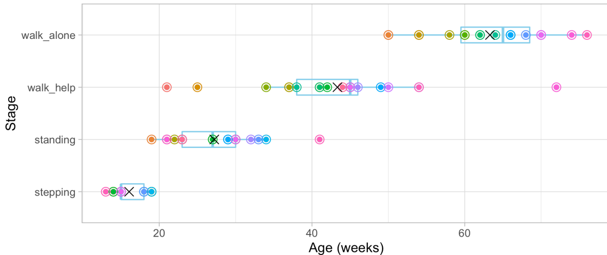
Figure 3.2. Mean (symbol x) and spread of the ages at which 21 children achieve four motor development milestones.
