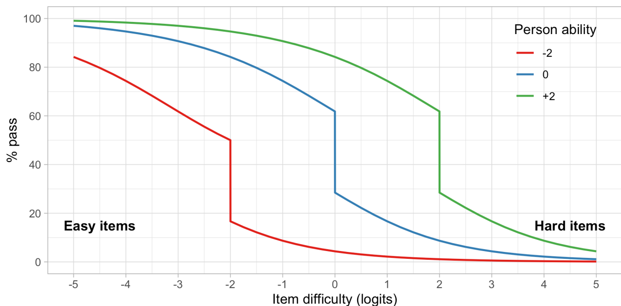
Figure 4.7. Person response functions for three children with abilities -2, 0 and +2, using a small test of items A, C and D.
