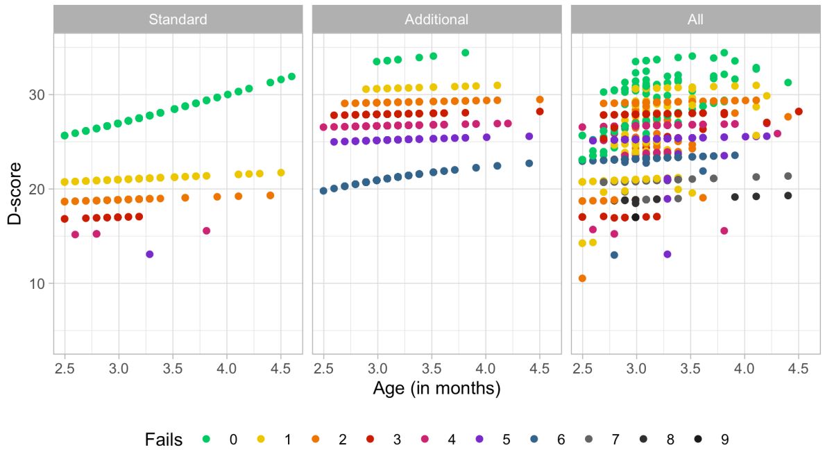
Figure 8.3. Distribution of the D-scores calculated from the standard, additional and all available milestones at month 3. Colors correspond to the number of fails.
