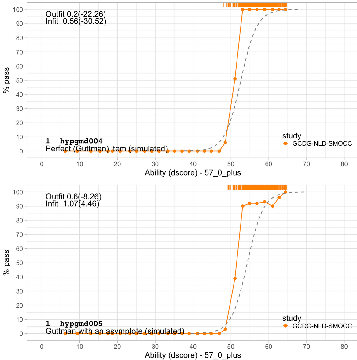
Figure 6.3. Two simulated items that illustrate item overfit.
