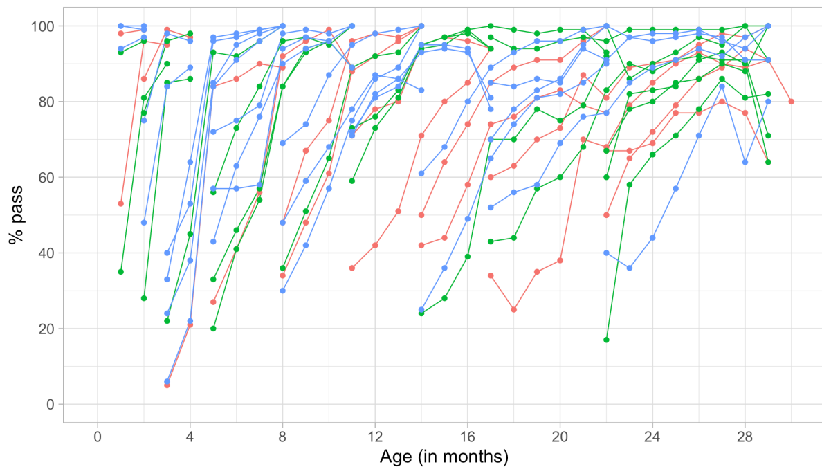
Figure 4.1. Empirical percentage of passing each milestone in the DDI against age (Source: SMOCC data, n = 2151 , 9 occasions).
