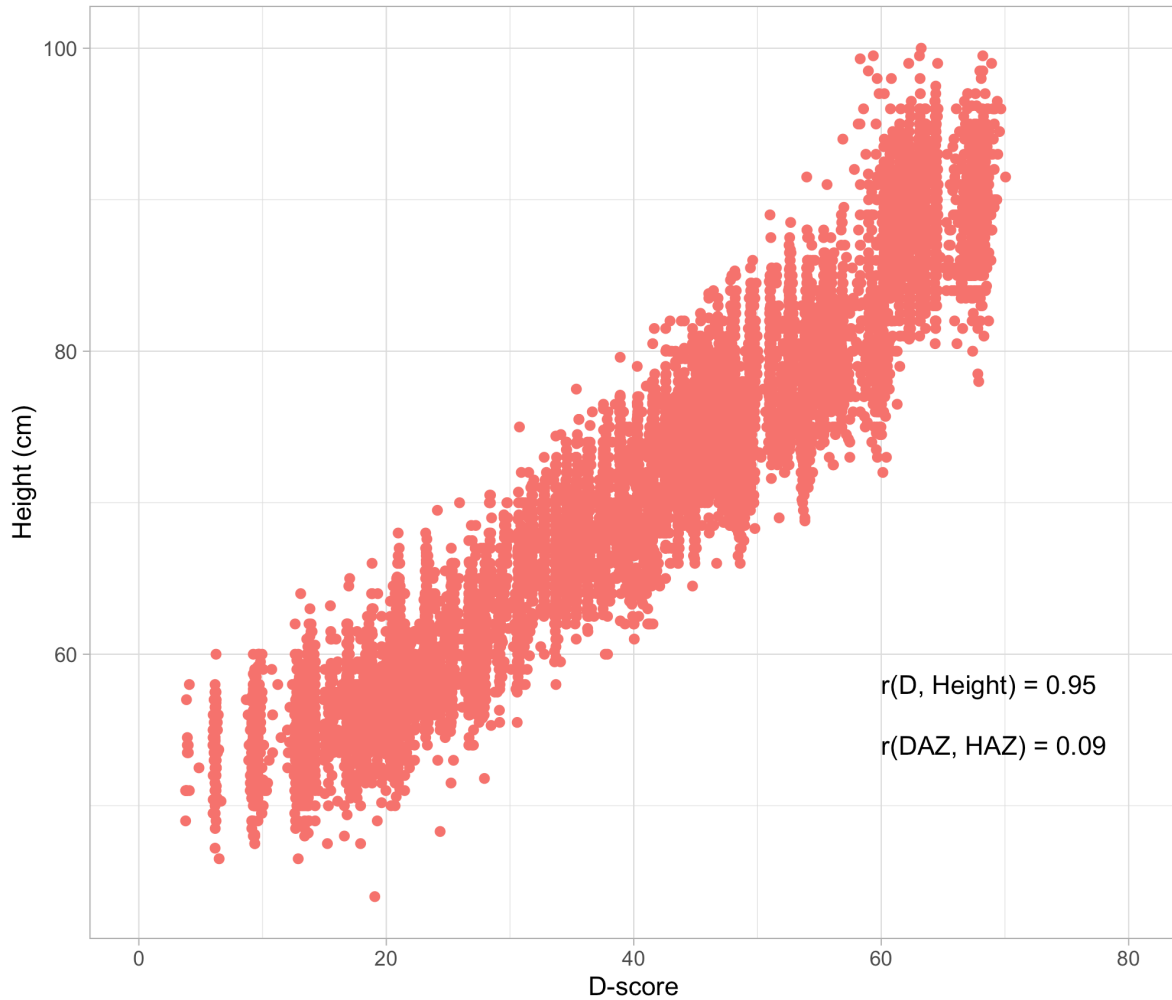
Figure 7.3. Relation between body height and the D-score in the SMOCC data.
