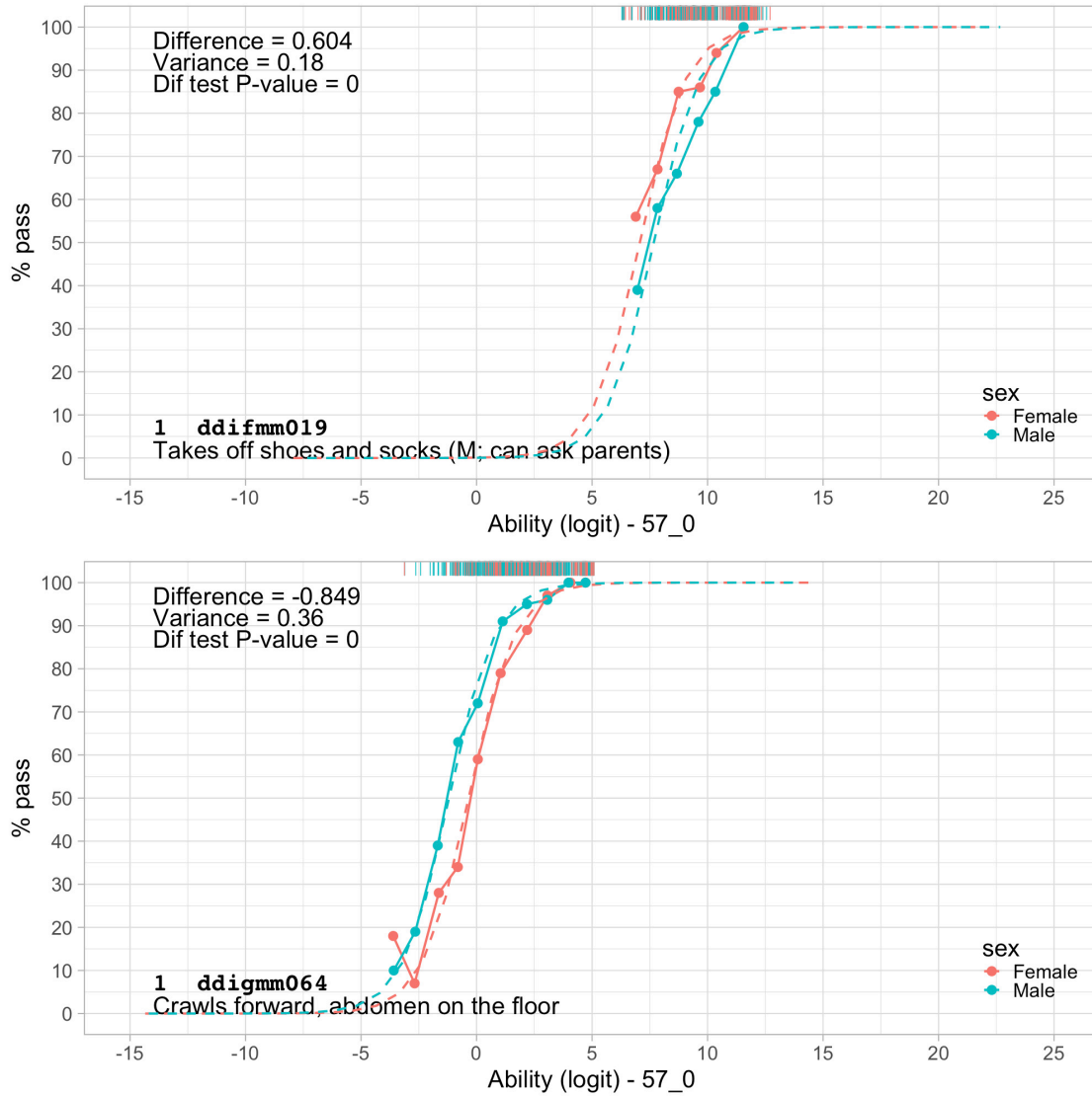
Figure 6.7. Two milestones from the DDI with different item response curves for boys and girls. There is evidence for uniform DIF.
