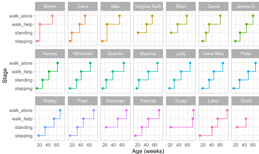
Figure 2.3. Staircase plot indicating the age at which each baby achieves a new milestone of gross-motor functioning.
