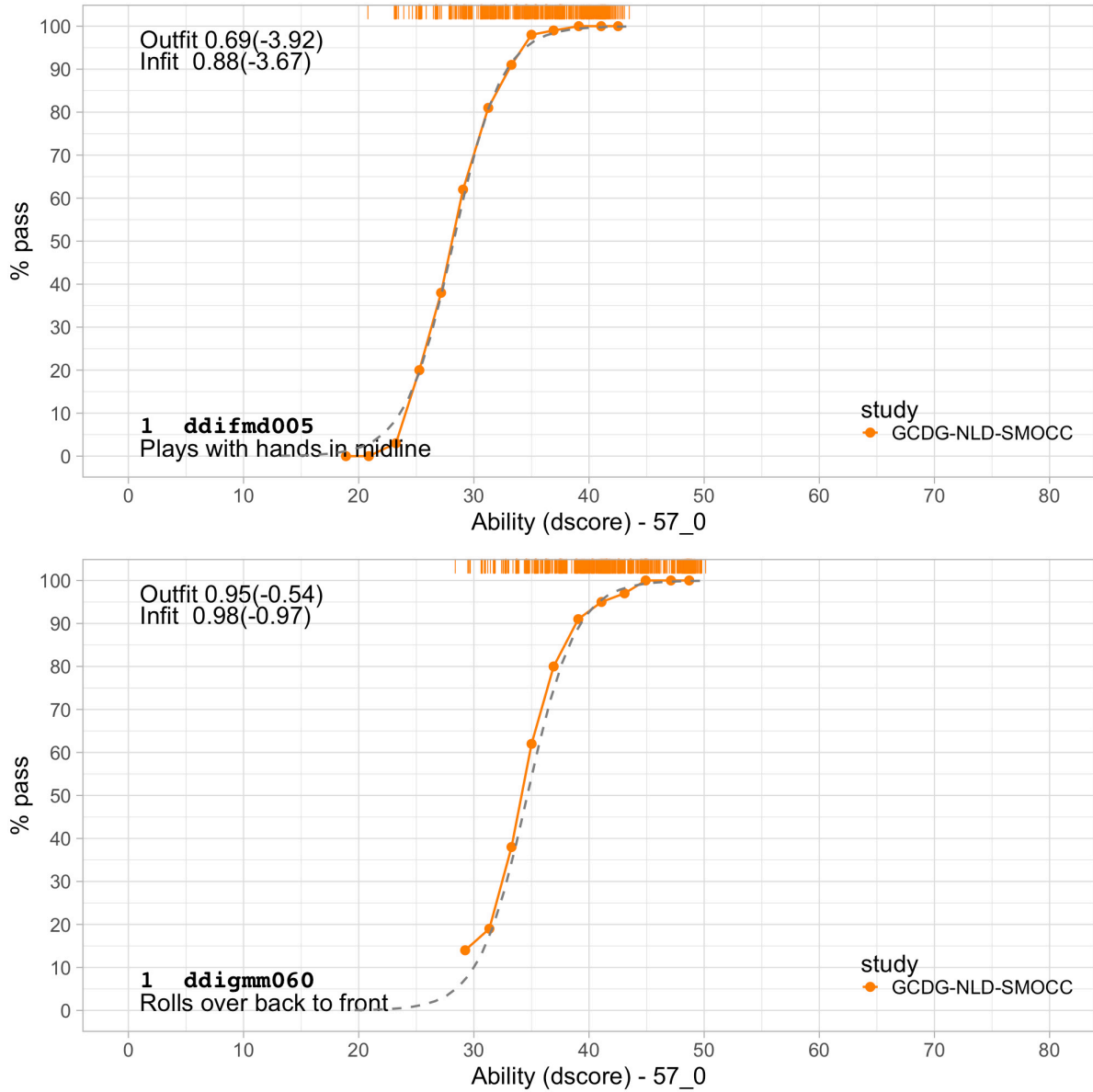
Figure 6.1. Empirical and fitted item response curves for two milestones from the DDI (SMOCC data).
