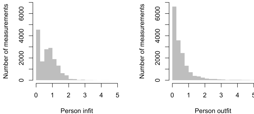
Figure 6.5. Frequency distribution of person infit (left) and person outfit (right) for 16538 measurements of the DDI (SMOCC data).
