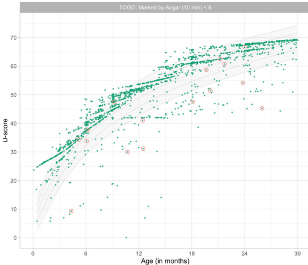
Figure 9.9. Distribution of D-score by age labelled by Apgar score (10 minutes) lower than 8. (Source: TOGO data).
