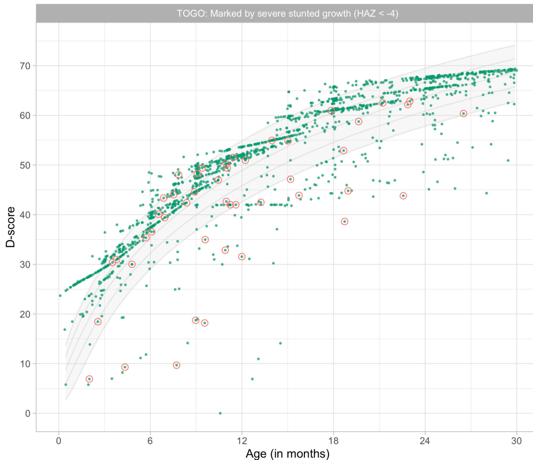
Figure 9.11. Distribution of D-score by age labelled by severe stunting (HAZ < -4) (Source: TOGO data).
