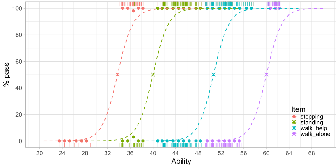
Figure 3.5. Modeled probability of achieving four motor milestones against the D-score.
