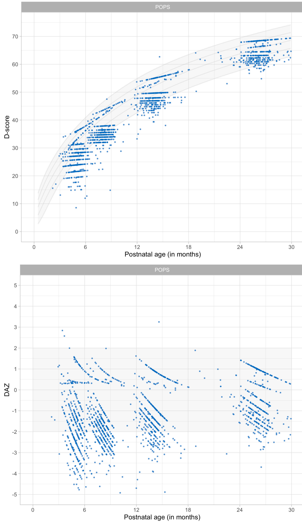
Figure 9.4. Distribution of D-score and DAZ without age correction for preterm birth ( f = 0.00 ).
