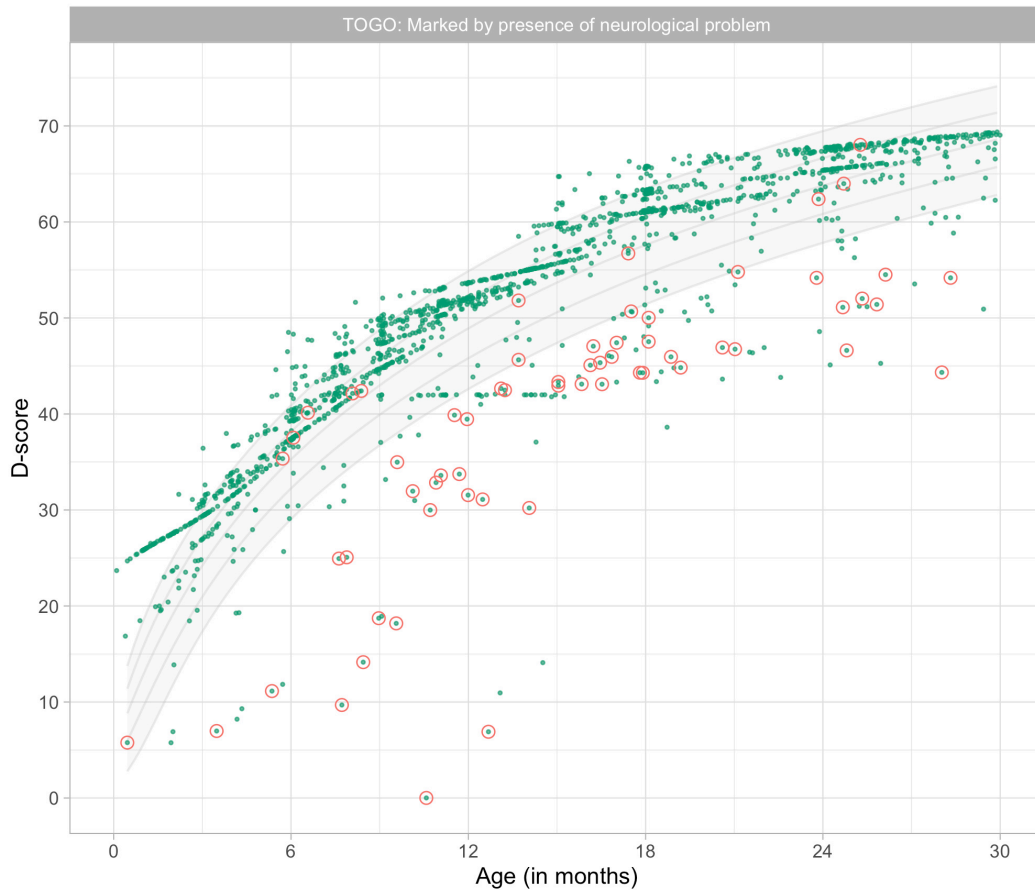
Figure 9.8. Distribution of D-score by age labelled by neurological (tonus and/or reflex) problems. (Source: TOGO data).
