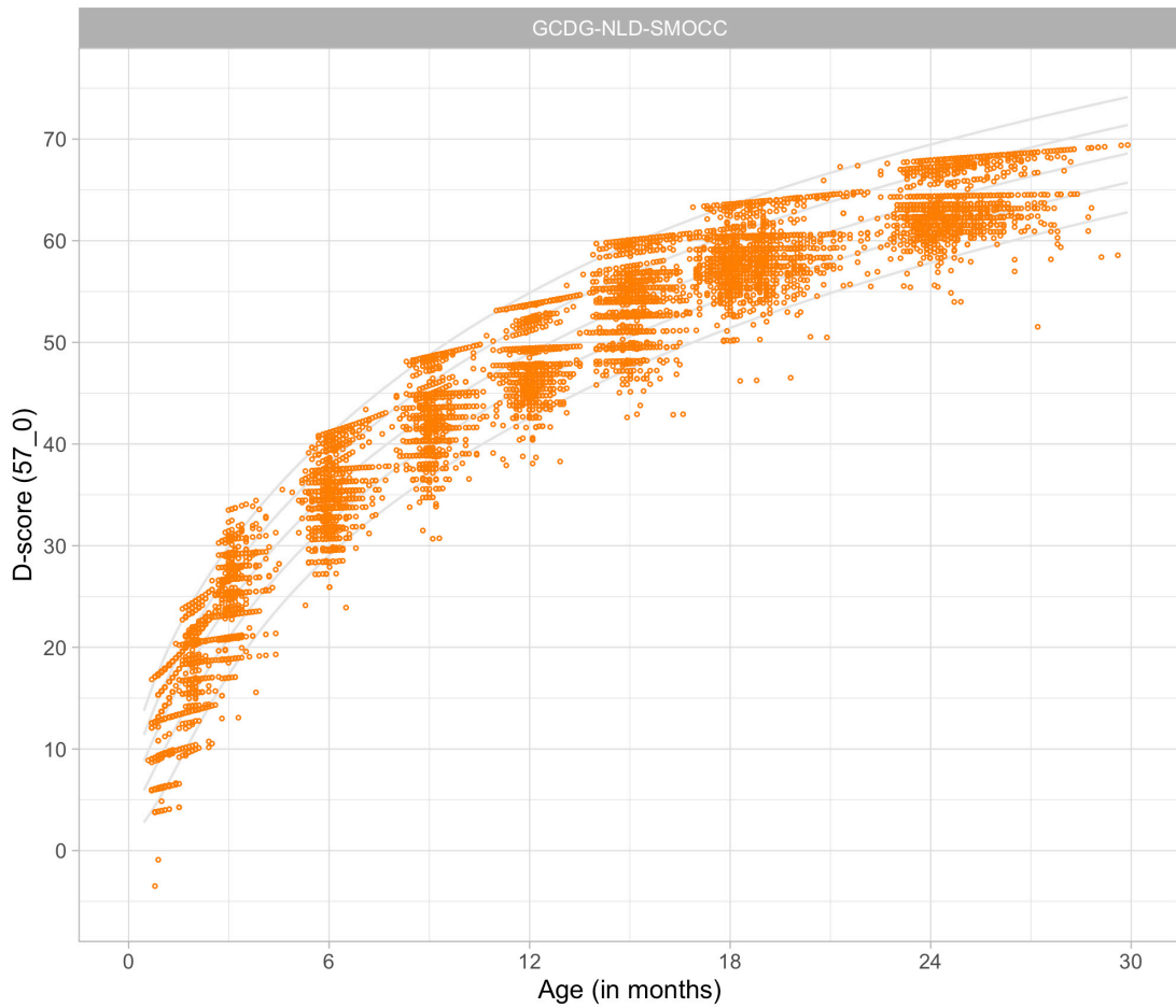
Figure 4.3. Relation between child D-score and child age in a cohort of Dutch children (Source: SMOCC data, n = 2151 , 9 occasions).
