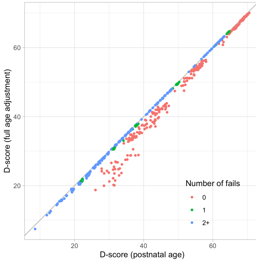
Figure 9.3. Scatterplot of two versions of the D-score, one calculated using postnatal age ( f = 0.00 ), the other calculated using full age-adjustment ( f = 1.00 ).
