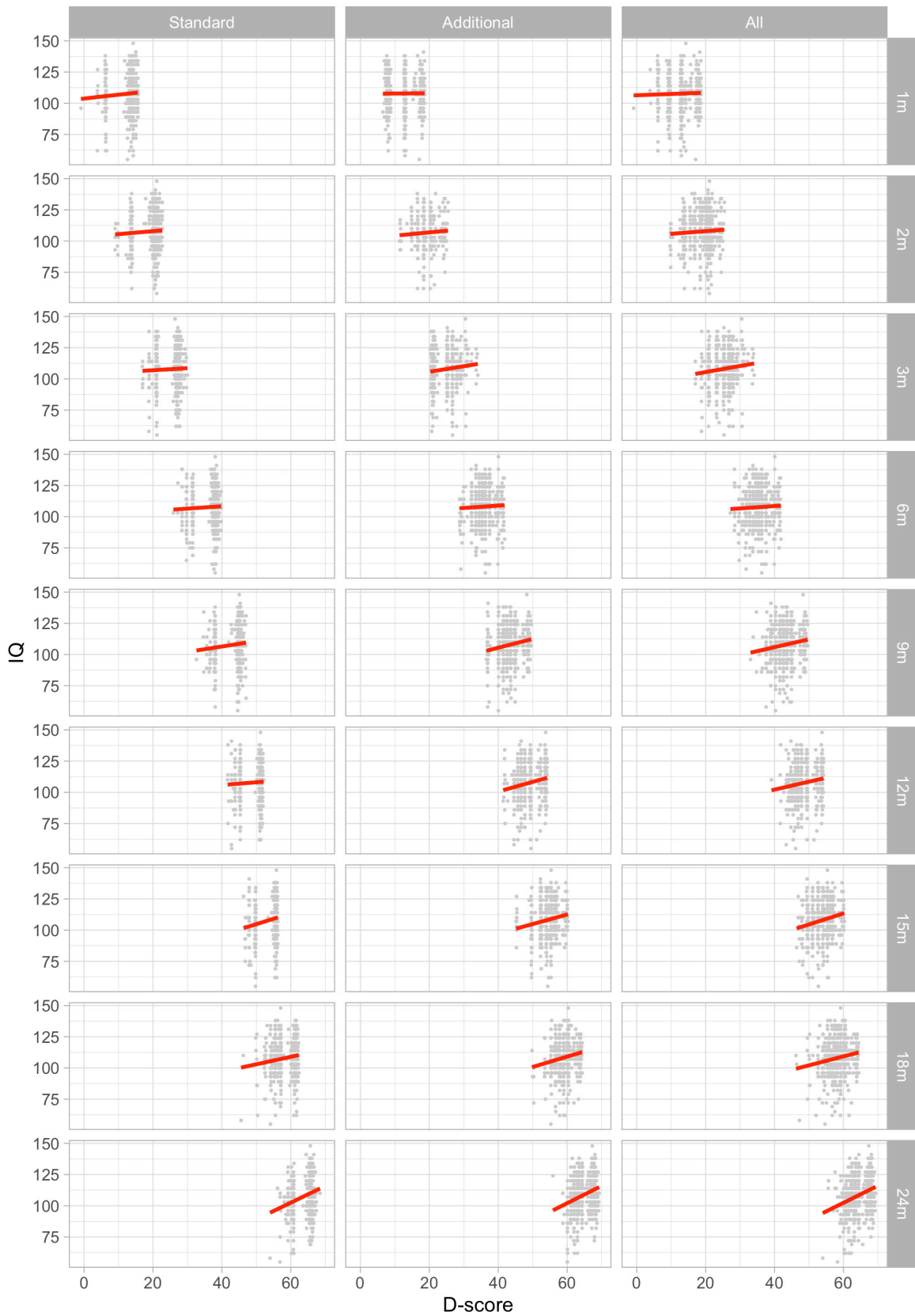
Figure 8.6. Relation between D-score at infancy and IQ at age 5 years according to three milestone sets and nine visits (SMOCC data, n = 557 ).
