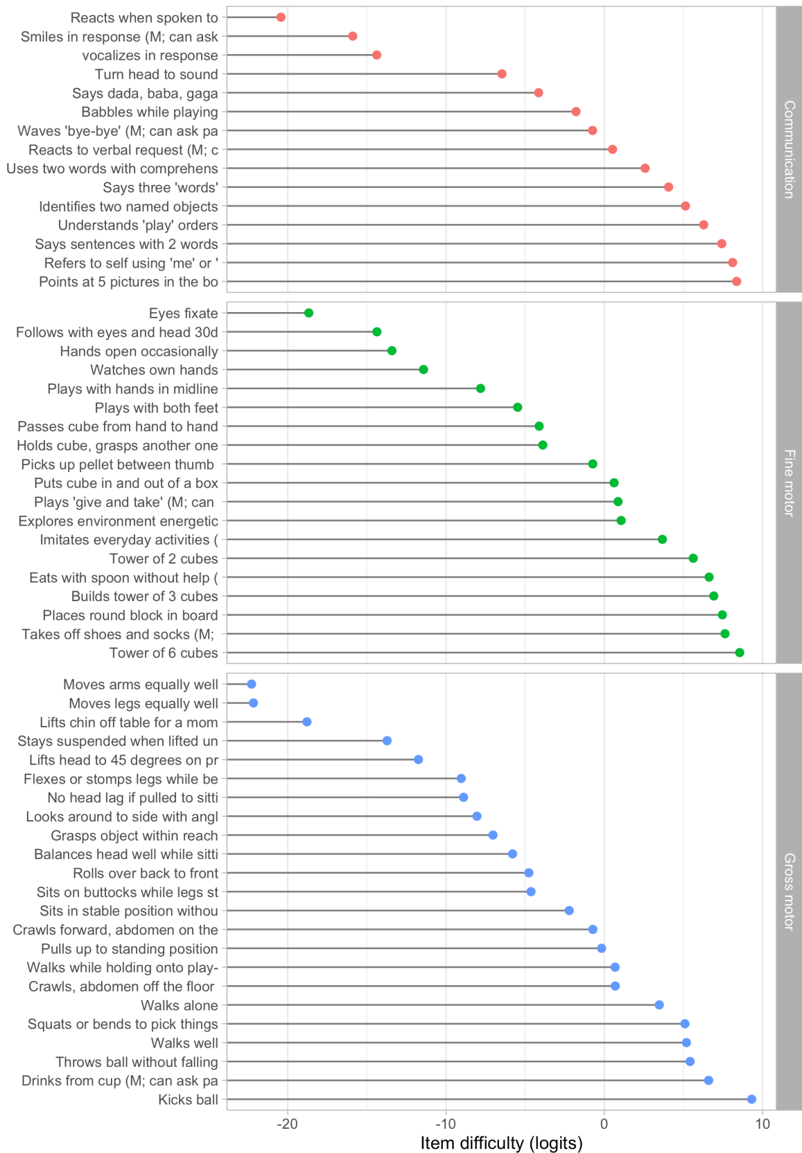
Figure 5.1. Estimated item difficulty parameters ( d_i ) for 57 milestones of the DDI (0 - 2 years).
