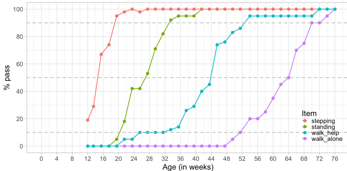
Figure 3.3. Probability of achieving four motor milestones against age.
