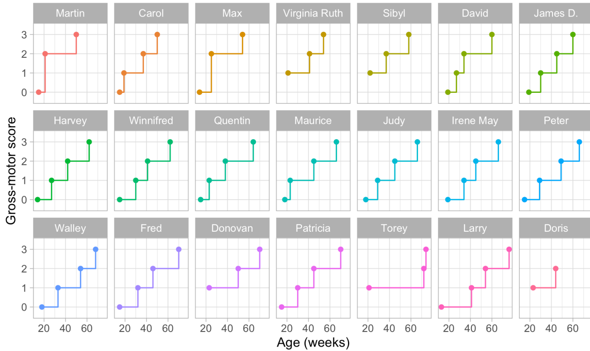
Figure 3.4. Same data as in Figure 2.3, but now with the vertical axis representing gross-motor score.
