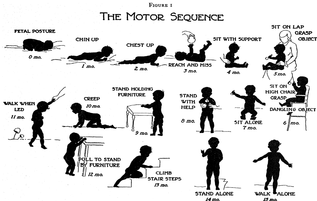
Figure 2.1. Gross motor development as a sequence of milestones. Source: Shirley (1933), with permission.
