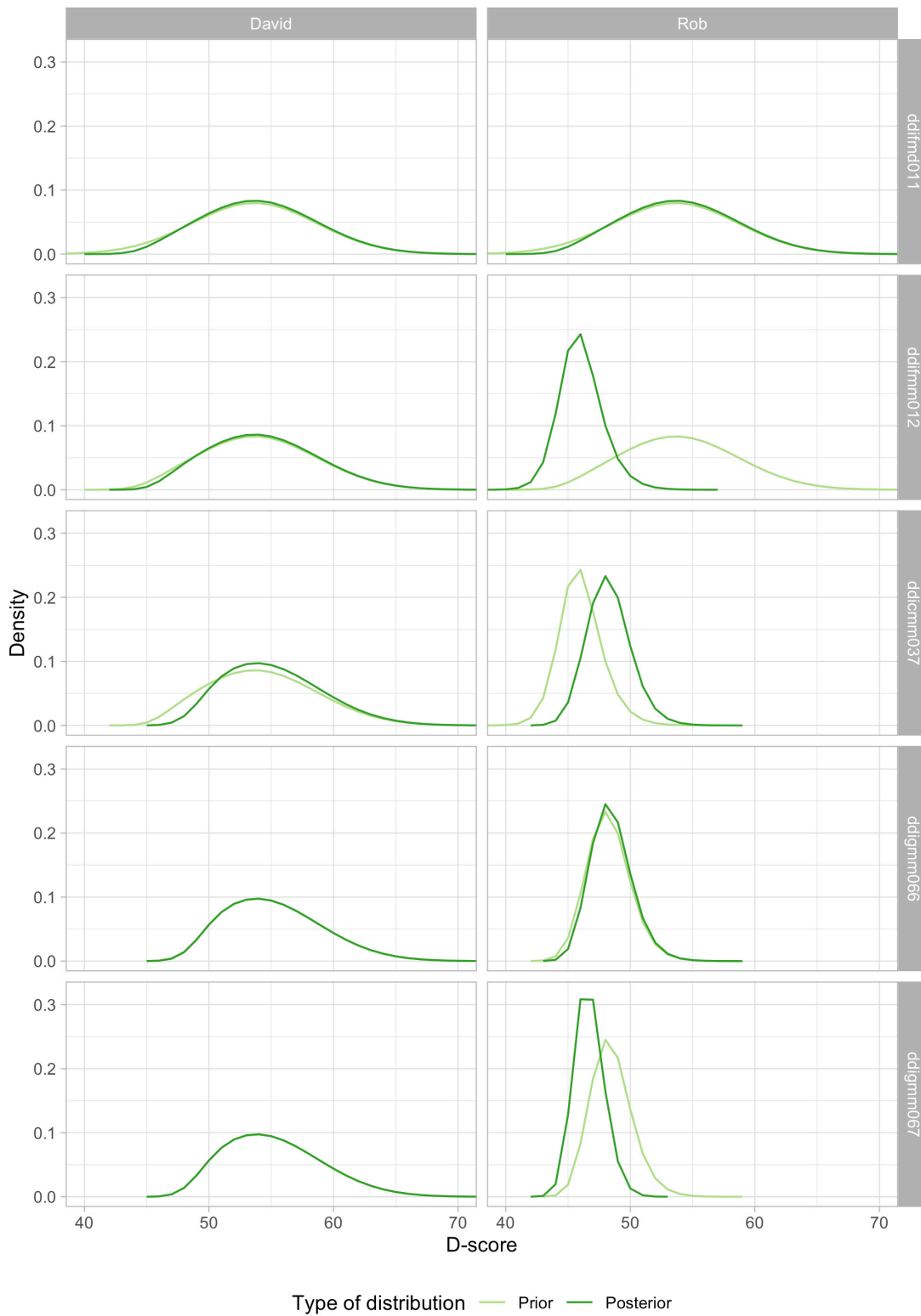
Figure 5.4. D-score distribution for David and Rob before (prior) and after (posterior) a milestone is taken into account.
