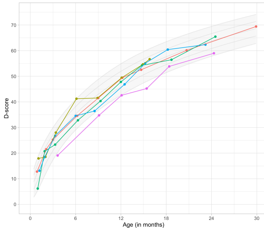
Figure 10.1. D-chart with five children from the SMOCC study.
