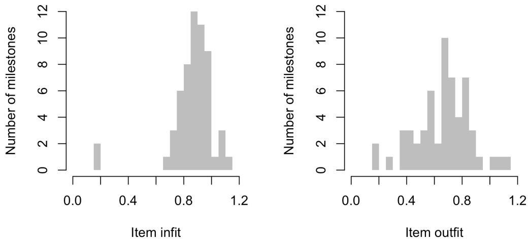
Figure 6.4. Frequency distribution of infit (left) and outfit (right) of 57 milestones from the DDI (SMOCC data).
