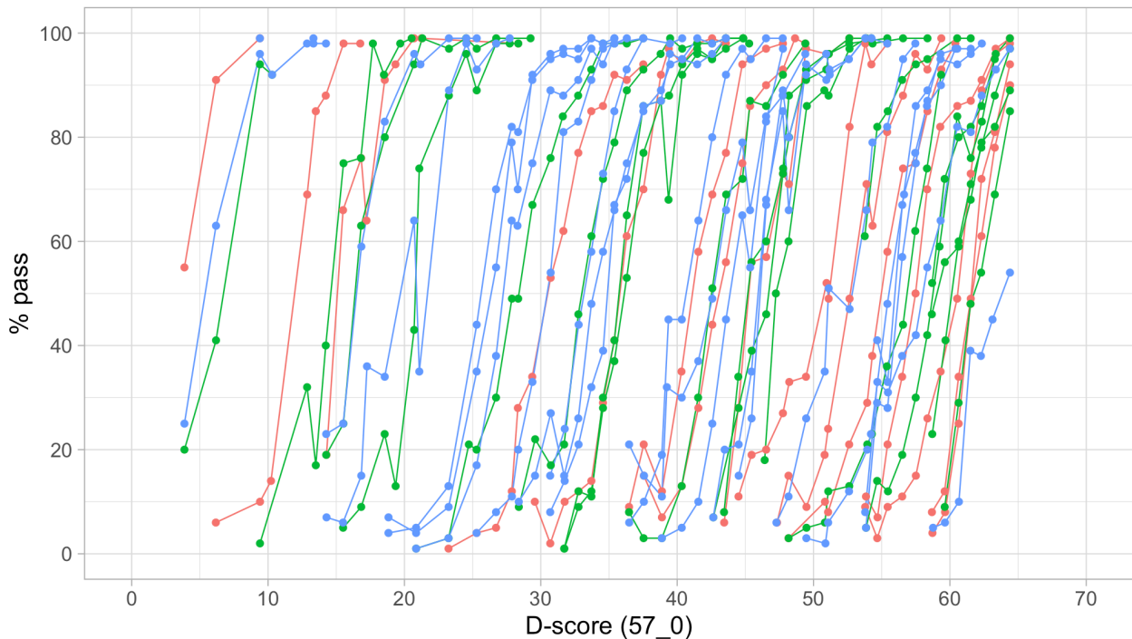
Figure 4.2. Empirical percentage of passing each milestone in the DDI against the D-score (Source: SMOCC data, 2151 children, 9 occasions).
