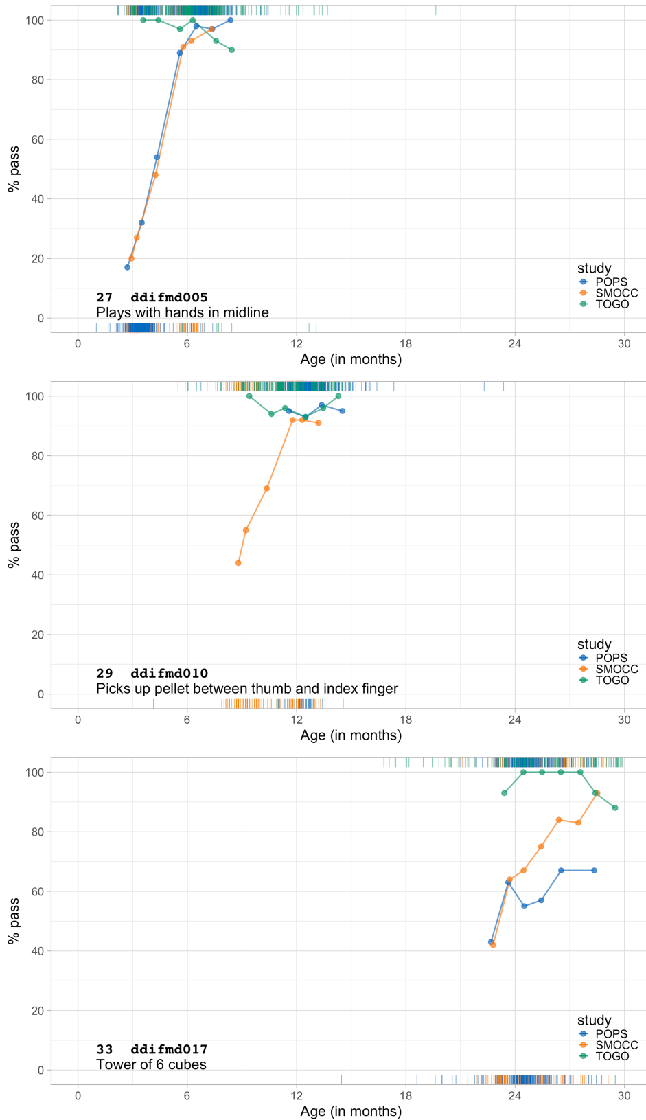
Figure 9.13. Fine motor milestones. Probability by age for SMOCC, POPS (corrected age) and TOGO studies for three milestones.
