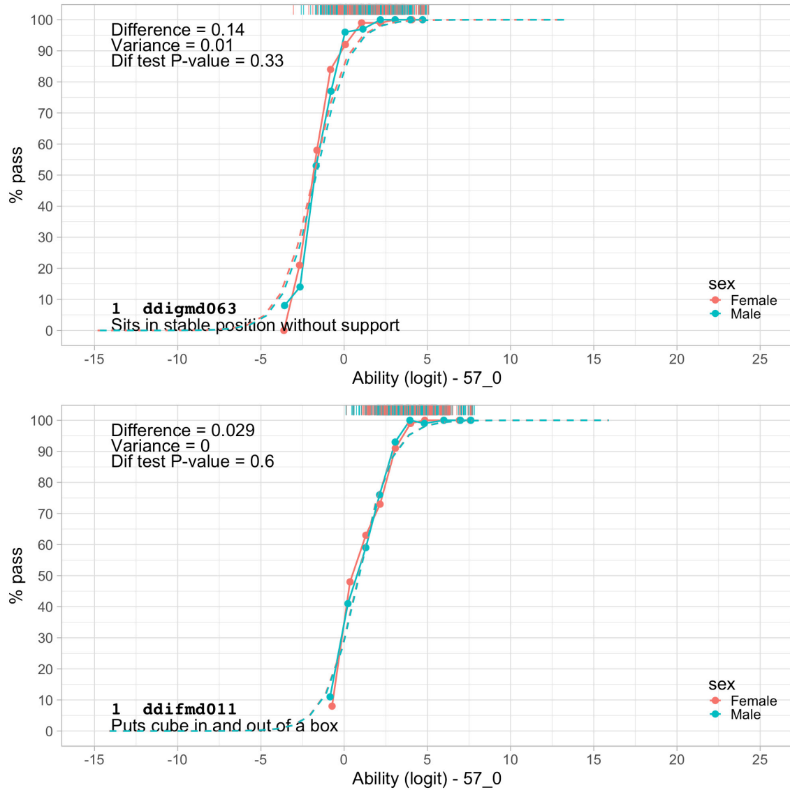
Figure 6.6. Two milestones from the DDI with similar item response curves for boys and girls. There is no DIF for sex.
