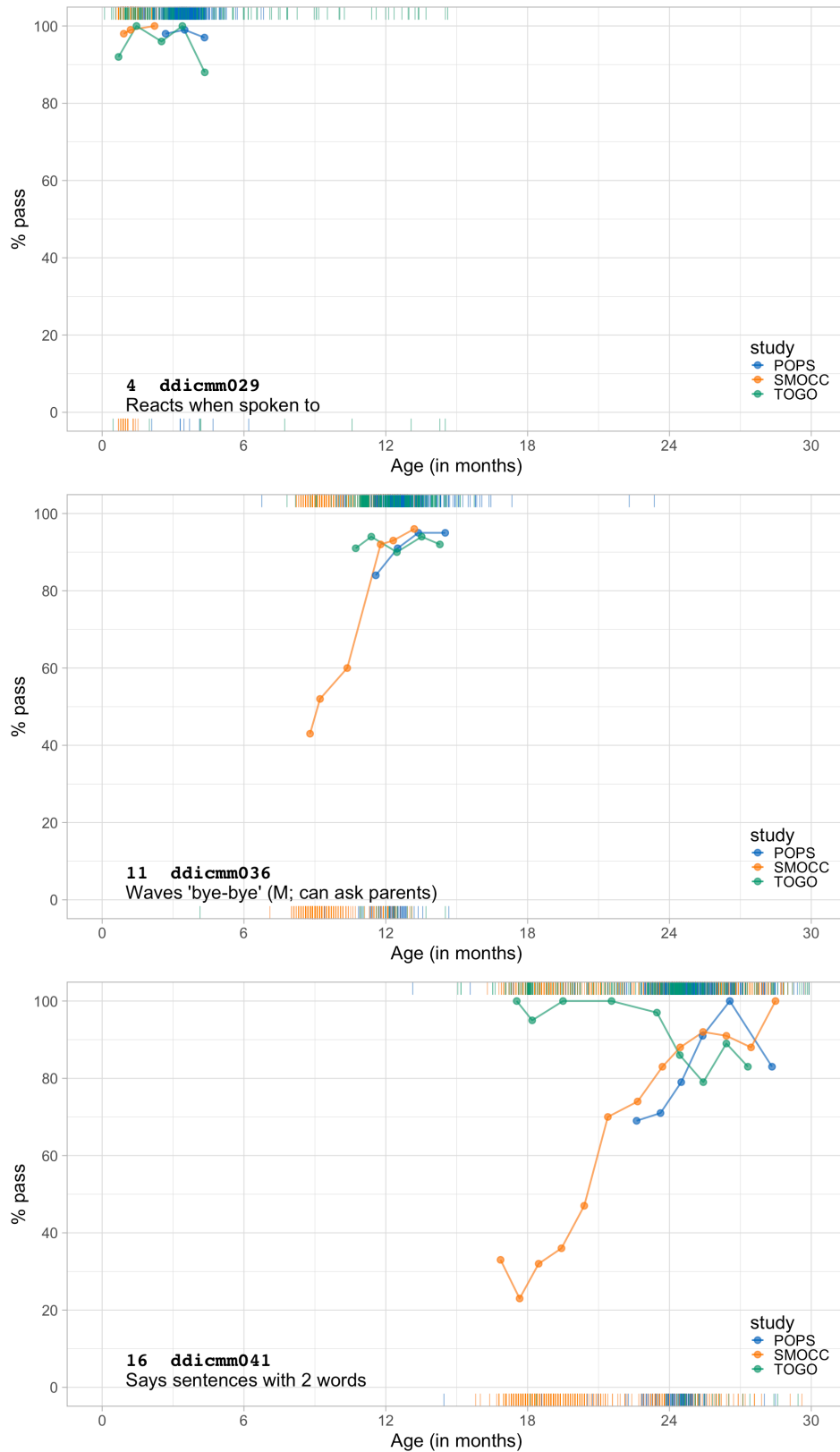
Figure 9.14. Communication and language milestones. Probability by age for SMOCC, POPS (corrected age) and TOGO studies for three milestones.
