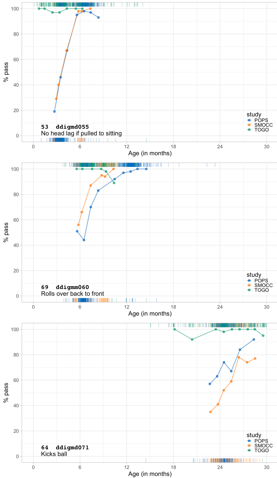
Figure 9.12. Gross motor milestones. Probability by age for SMOCC, POPS (corrected age) and TOGO studies for three milestones.
