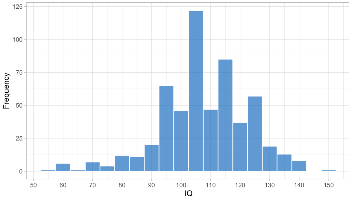
Figure 8.5. Histogram of UKKI IQ scores taken around the age of five years (SMOCC data, n = 557 ).
