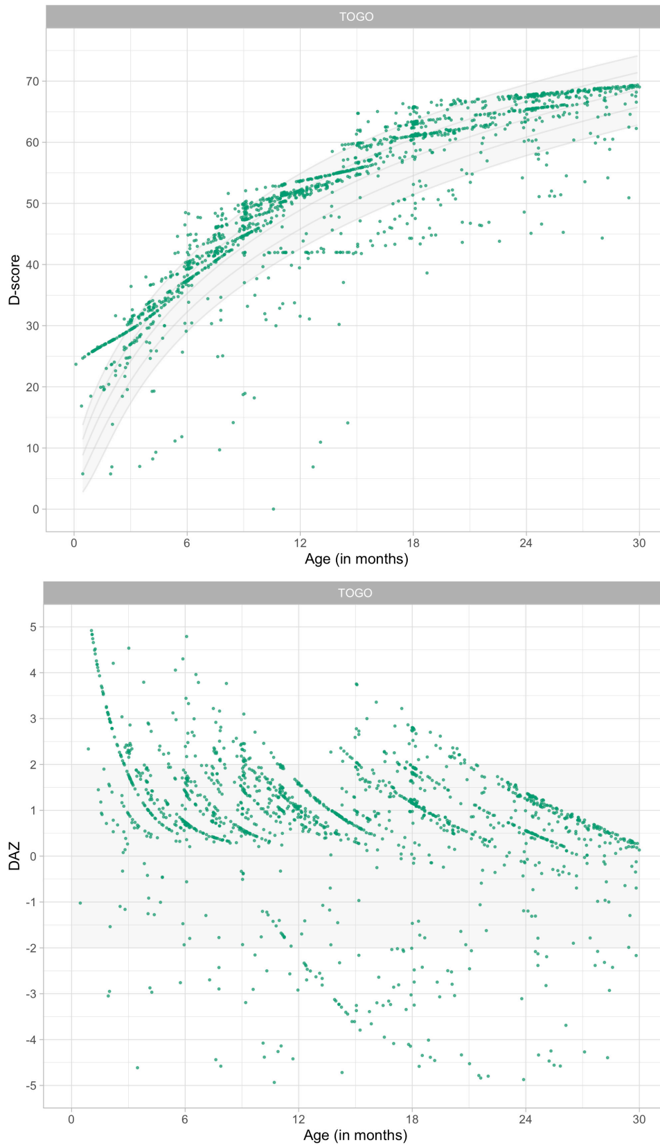
Figure 9.6. Distribution of D-score and DAZ by child age of children living near Kpalimé, Togo (Source: TOGO data, n = 1567 ).
