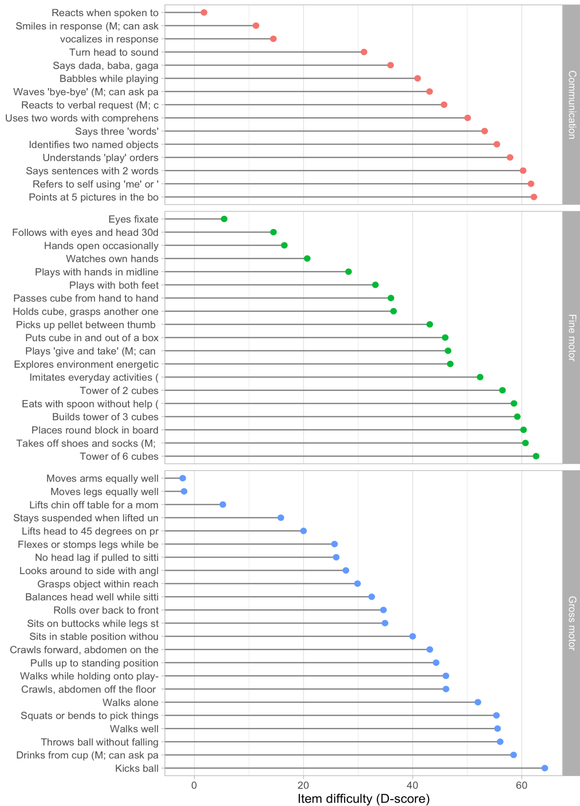
Figure 5.2. Estimated item difficulty parameters ( d_i ) for 57 milestones of the DDI (0 - 2 years). Milestones ddi_gmd057 and ddi_gmd063 are anchored at values of 20D and 40D, respectively.
