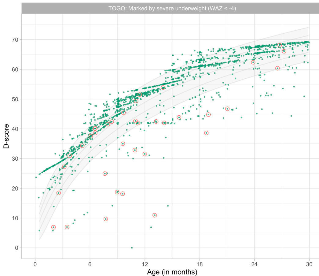
Figure 9.10. Distribution of D-score by age labelled by severe underweight (WAZ < -4) (Source: TOGO data).
