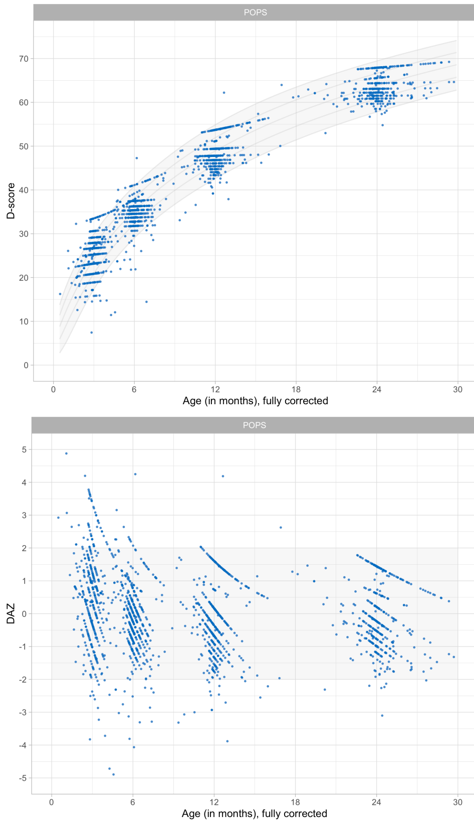
Figure 9.5. Distribution of D-score and DAZ under full age correction for preterm birth ( f = 0.00 ).
