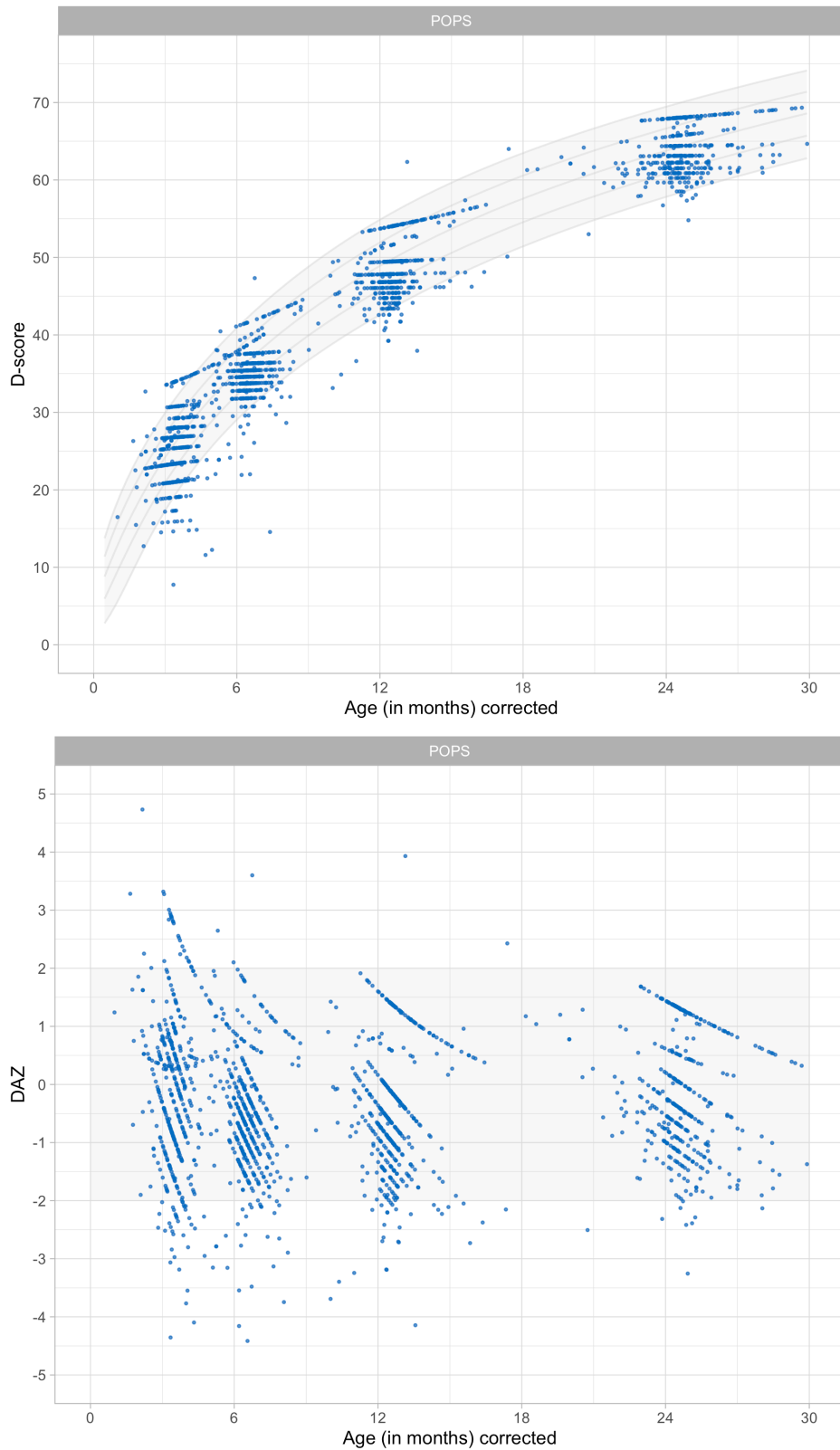
Figure 9.2. Distribution of D-score and DAZ by child age in a cohort of preterm aged 0–2 years. Ages are corrected for preterm birth by a factor of 0.75 (Source: POPS data, 450 children, four occasions).
