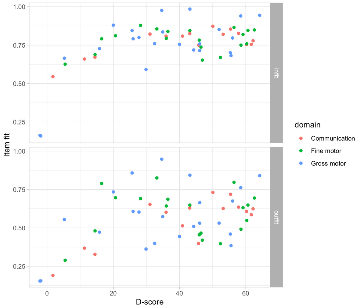
Figure 7.2. Item fit by D-score for the DDI domains.
