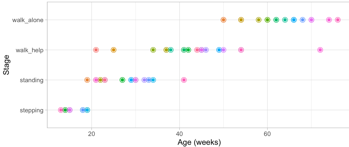
Figure 3.1. Ages at which 21 children achieve four motor development milestones.
