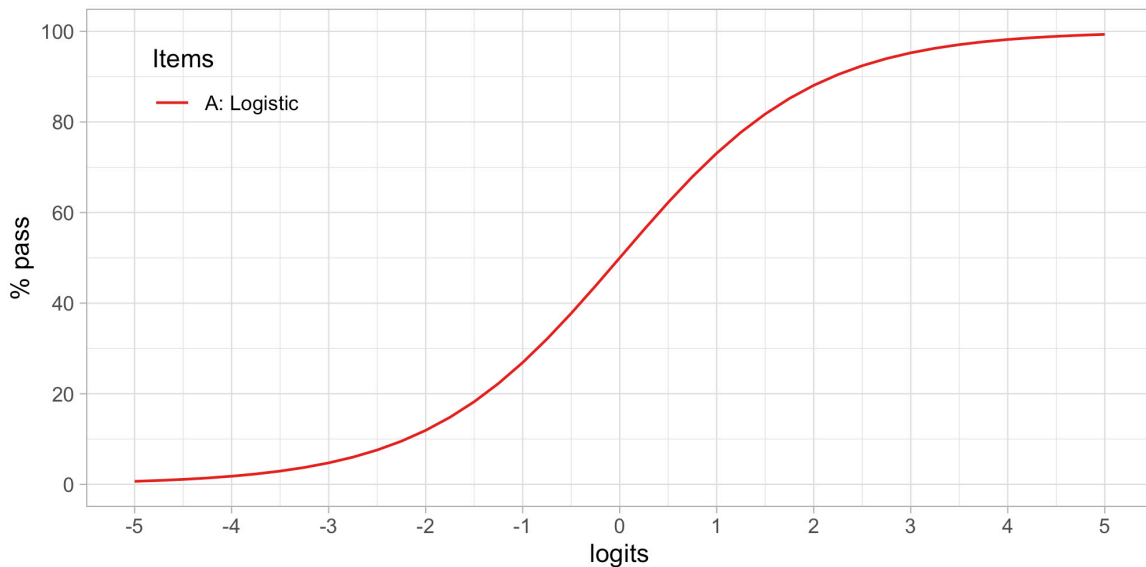
Figure 4.5. Standard logistic curve. Percentage of children passing an item for a given ability-difficulty gap \beta_n - \delta_i .
