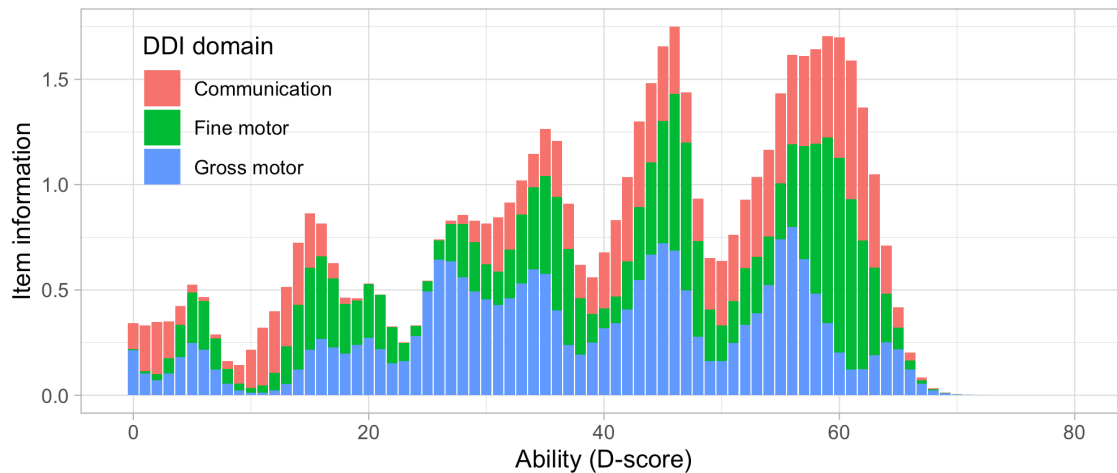
Figure 7.1. Cumulative item information by DDI domain.
