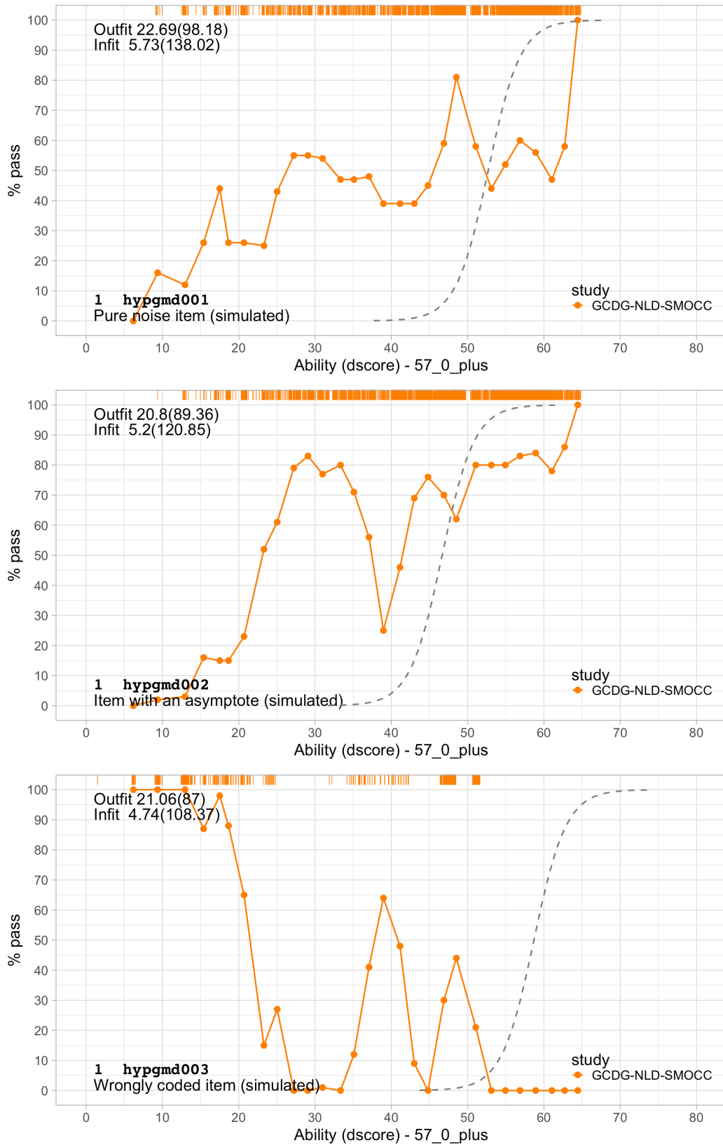
Figure 6.2. Three simulated items that illustrate various forms of item misfit.
