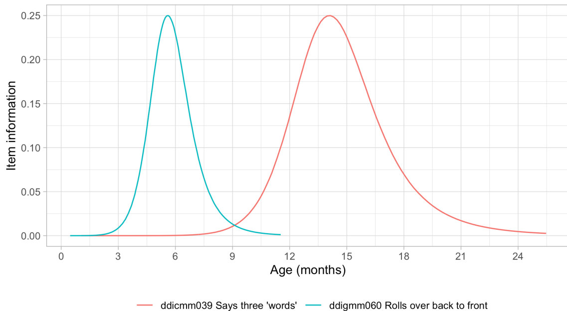
Figure 6.9. Information information of Figure 6.8 plotted against age.
