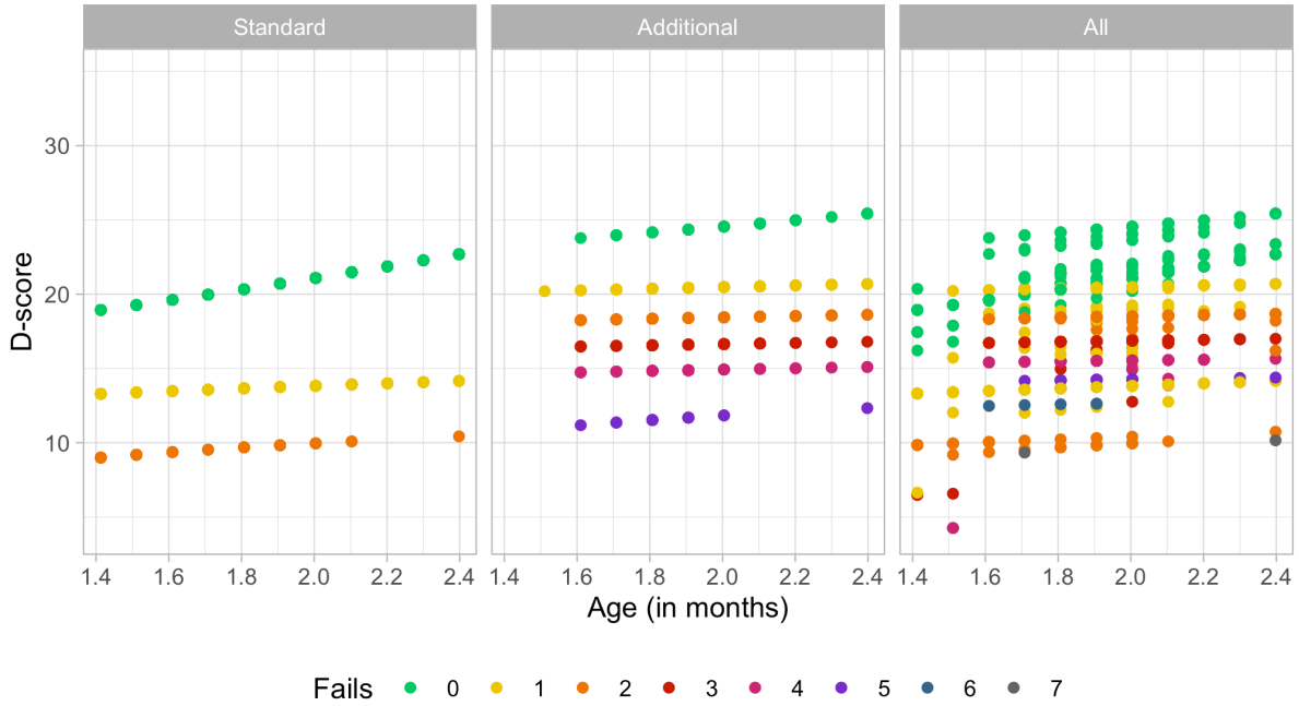
Figure 8.2. Distribution of the D-scores calculated from the standard, additional and all available milestones at month 2. Colors correspond to the number of fails.
