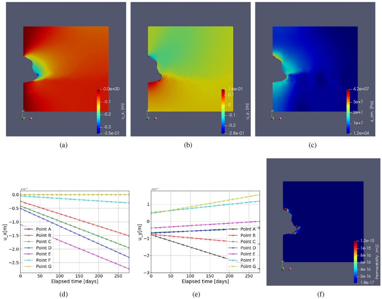
Figure 11. Test Case 5: illustration of the horizontal displacement u_x (a), vertical displacement u_y (b), von Mises stress s_{vmm} (c) and permeability (f) for irregular cavern shape model with heterogeneous properties. The variation of horizontal (d) and vertical (e) deformations over time around caverns are also shown for the marked points in Fig. 10.
