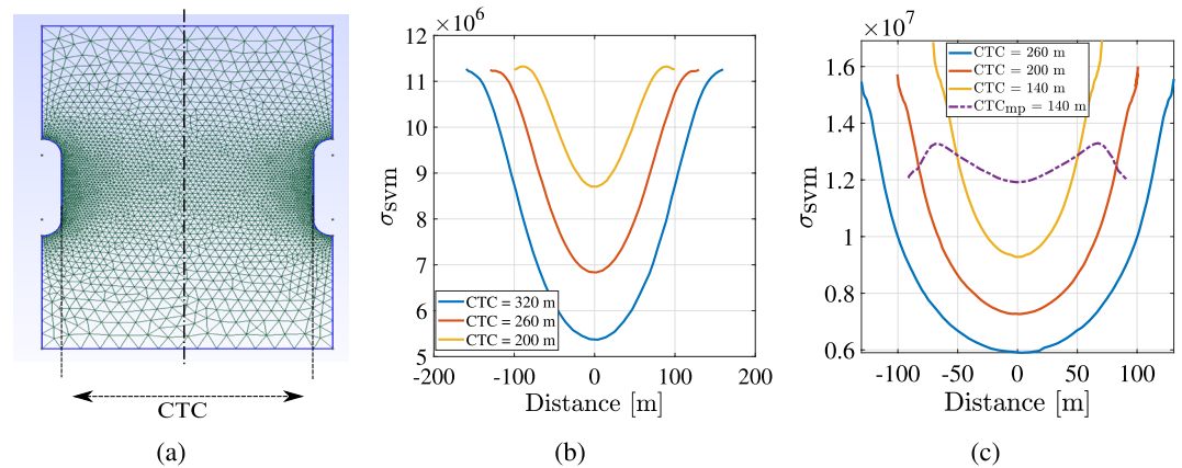
Figure 20. Multi-cavern simulation: (a) shows the example of computational mesh showing cavern to cavern distance (CTC) for regular shaped cavern. (b) shows the variation of von Mises stress with stress for regular shaped caverns at different CTC. (c) shows the variation of von Mises stress with stress for irregular shaped caverns at different CTC.
