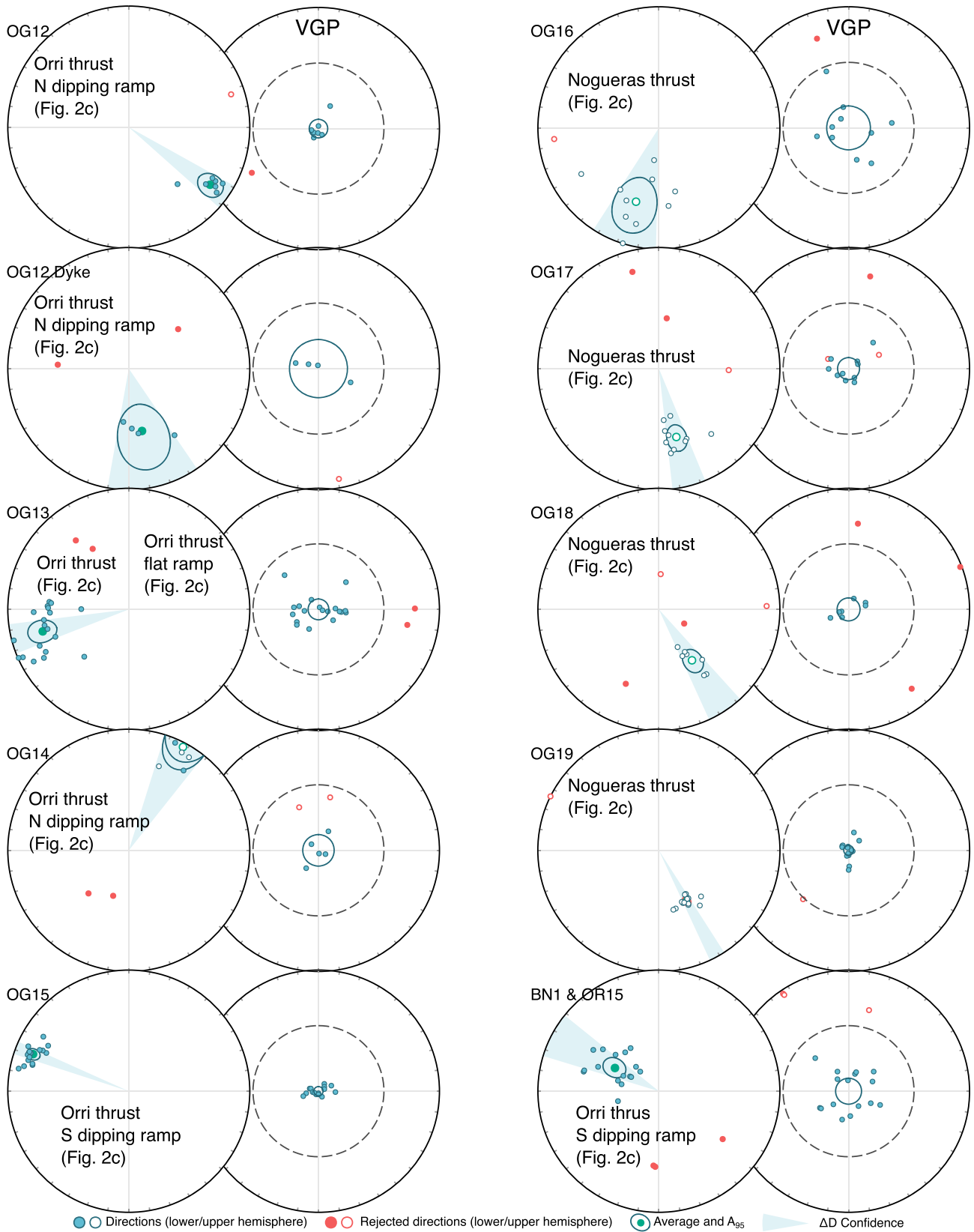
Figure 9. Directional and VGP results in geographic coordinates of sites OG12–OG19 and BN1–OR15. Uncertainty envelope is in both cases VGP A95. Red dots are those that fall outside of the 45° cut-off. Sites OG02, 05 and 08 did not provide statistically meaningful results and were not interpreted.
