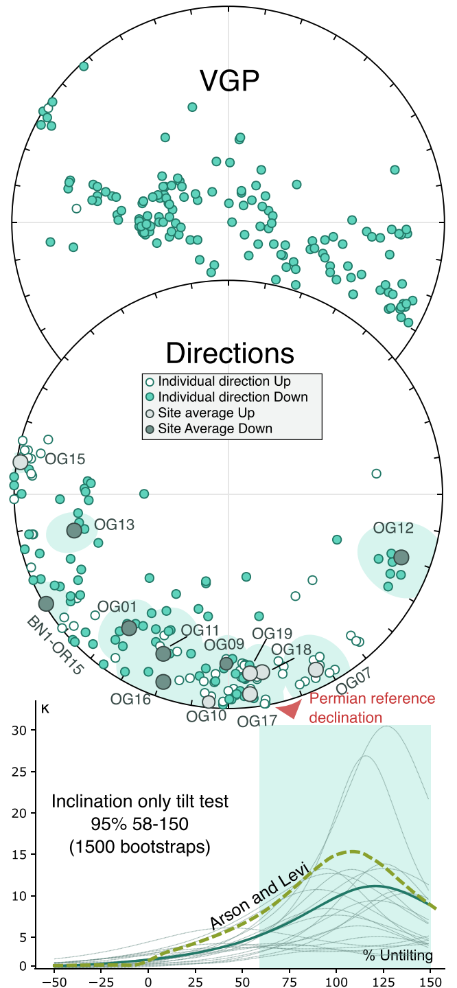
Figure 12. Results after the inferred Alpine tilt correction. Permian reference declination for Iberia is after Weil et al. (2010). The results show a positive inclination only tilt test following the methodology of Enkin & Watson (1996) (selected bootstraps in thin grey lines) and Arson & Levi (2010) approach (dashed line).
