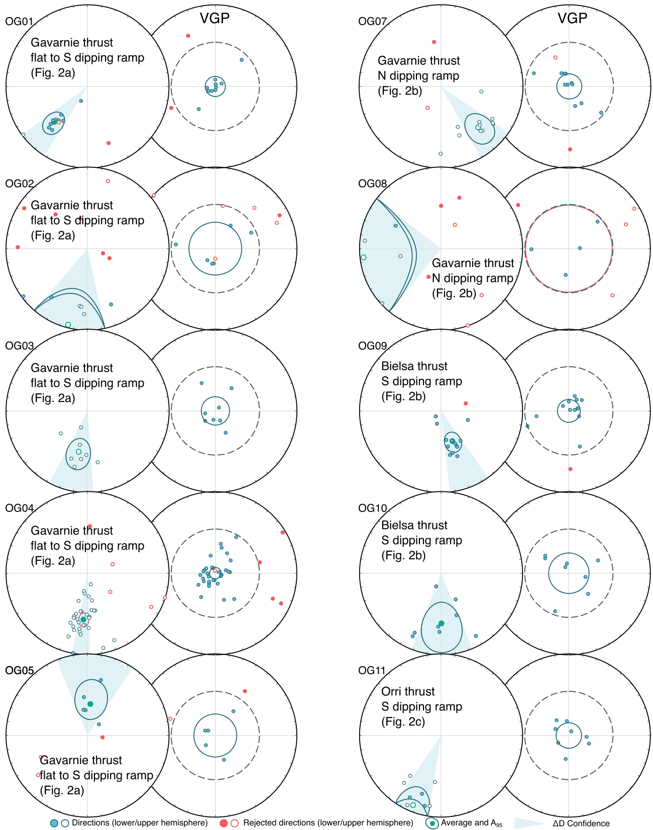
Figure 8. Directional and VGP results in geographic coordinates of sites OG01–OG11. Uncertainty envelope is in both cases VGP A_{95} . Red dots are those that fall outside of the 45^\circ cut-off. Sites OG02, 05 and 08 did not provide statistically meaningful results and were not interpreted.
