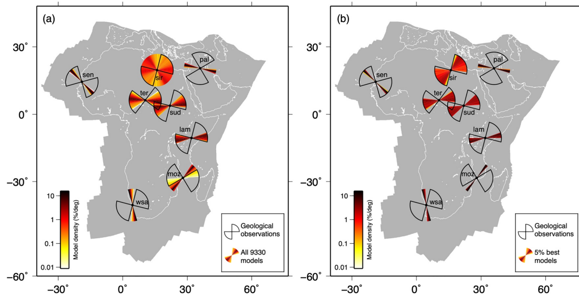
Figure 9. Comparison between modeled and observed S_{Hmin} directions for the modeled stress fields corresponding to all force sets with torque balance (a) and for only the 5% overall best-fitting models (b). The S_{Hmin} directions from geological observations are plotted as wedges to account for the observational uncertainty in stress orientation. For each location, the range of modeled S_{Hmin} directions is also plotted as wedges, with the wedges colored according to the model density. The model density represents the percentage of the total number of models per degree, so that most models line up in the dark colored directions. lam, Lamu embayment and Anza rift (Kenya); moz, Mozambique basins; pal, Palmyride and Euphrates basins (Syria); sen, Senegal basin; sir, Sirt basins (Libya); sud, Sudan rifts (South Sudan); ter, Termit trough (eastern Niger); wsa, western South African margin.
