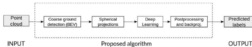
Fig. 6. Workflow of automatic point cloud segmentation.
