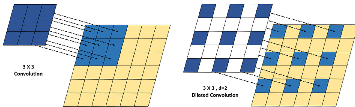
Fig. 13. Convolutions: (left) 3 × 3 regular convolution mostly used in CNNs. (right) 3 × 3 dilated convolution with d=2 covering an area of 5 × 5 is used in GRanD-Net resulting in lesser strides and parameters.
